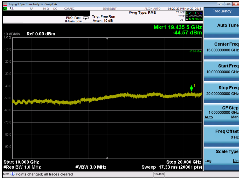
Plot 7-69. Conducted Spurious Plot (Band 2 – 20.0MHz QPSK – RB Size 1, RB Offset 0 – Mid Channel)
