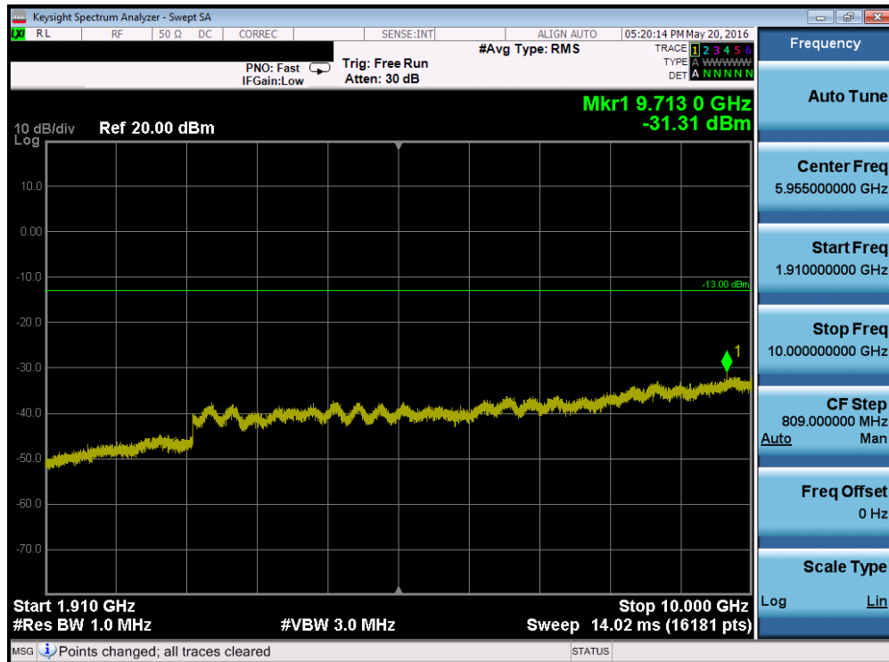
Plot 7-68. Conducted Spurious Plot (Band 2 – 20.0MHz QPSK – RB Size 1, RB Offset 0 – Mid Channel)
