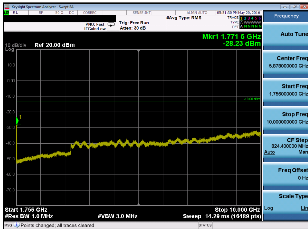
Plot 7-62. Conducted Spurious Plot (Band 4 – 20.0MHz QPSK – RB Size 1, RB Offset 0 – High Channel)
