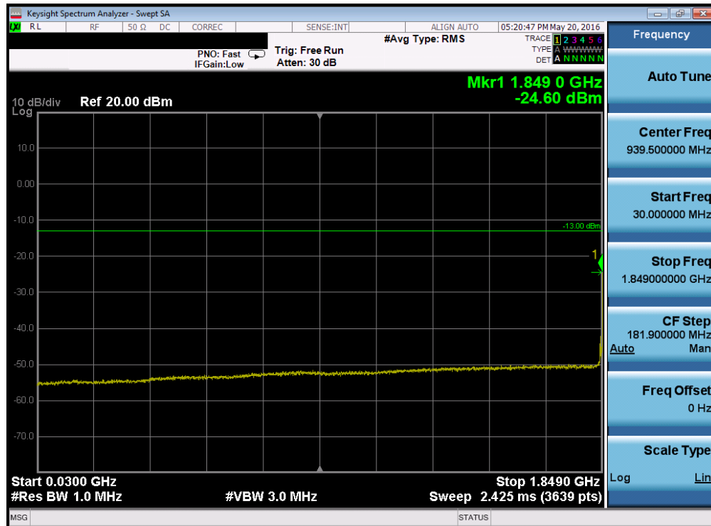
Plot 7-64. Conducted Spurious Plot (Band 2 – 20.0MHz QPSK – RB Size 1, RB Offset 0– Low Channel)
