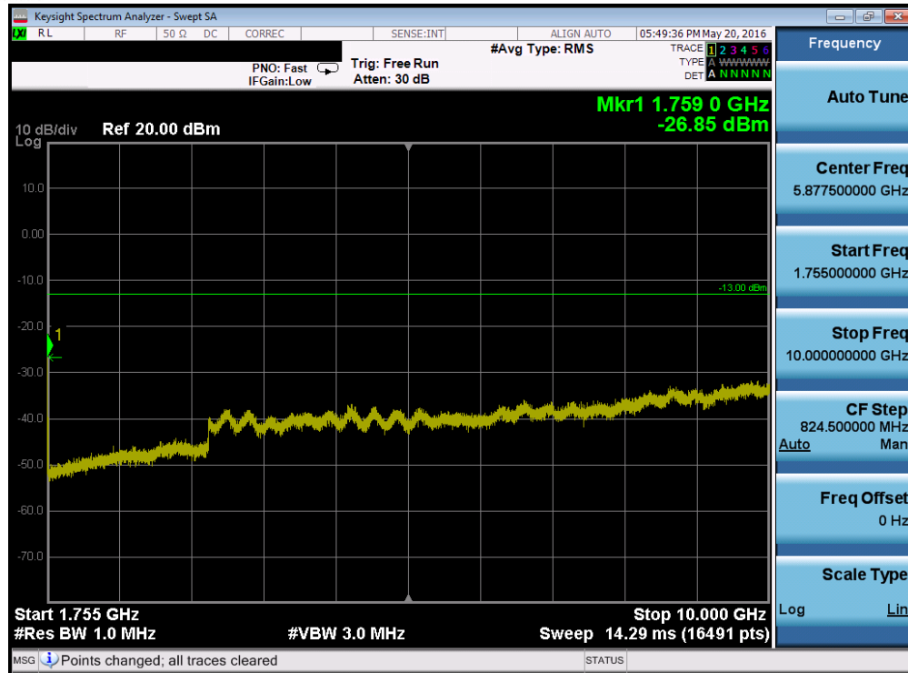
Plot 7-59. Conducted Spurious Plot (Band 4 – 20.0MHz QPSK – RB Size 1, RB Offset 0 – Mid Channel)
