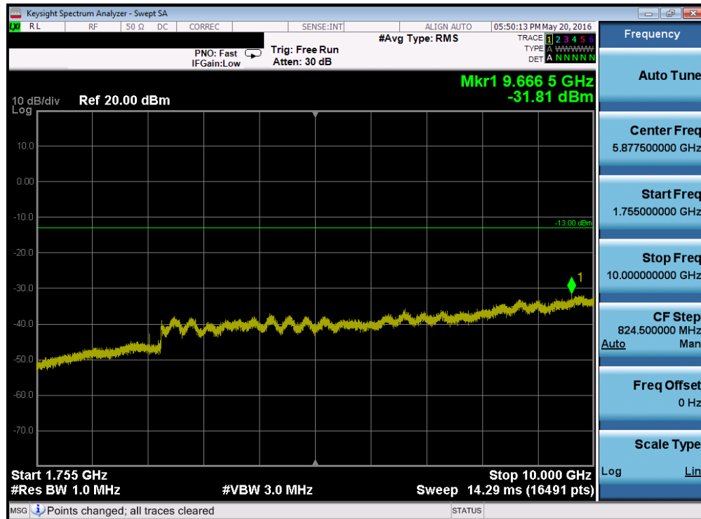
Plot 7-56. Conducted Spurious Plot (Band 4 – 20.0MHz QPSK – RB Size 1, RB Offset 0 – Low Channel)
