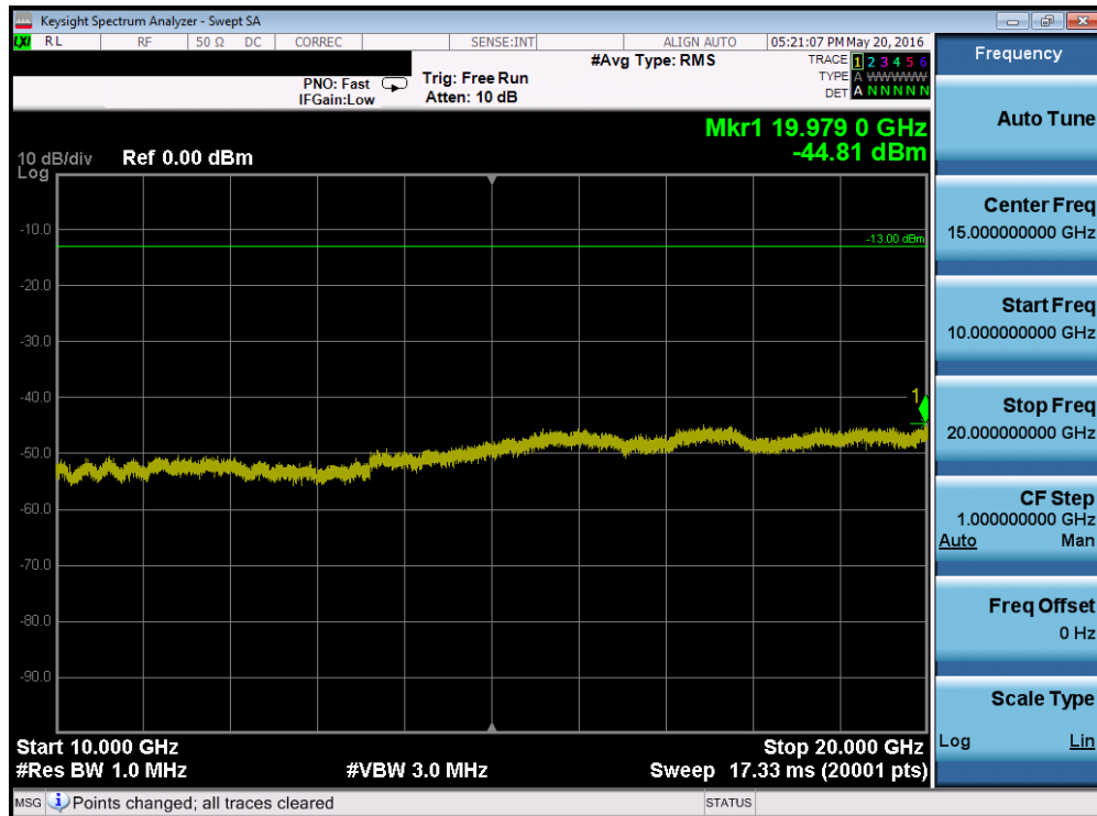
Plot 7-66. Conducted Spurious Plot (Band 2 – 20.0MHz QPSK – RB Size 1, RB Offset 0 – Low Channel)
