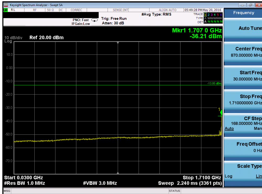
Plot 7-58. Conducted Spurious Plot (Band 4 – 20.0MHz QPSK – RB Size 1, RB Offset 0 – Mid Channel)
