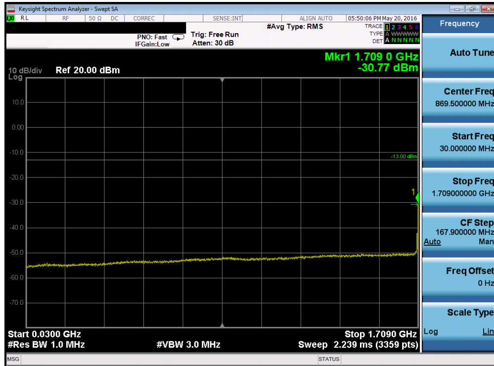
Plot 7-55. Conducted Spurious Plot (Band 4 – 20.0MHz QPSK – RB Size 1, RB Offset 0– Low Channel)
