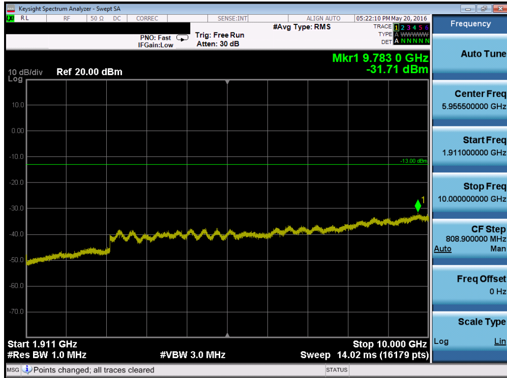
Plot 7-71. Conducted Spurious Plot (Band 2 – 20.0MHz QPSK – RB Size 1, RB Offset 0 – High Channel)
