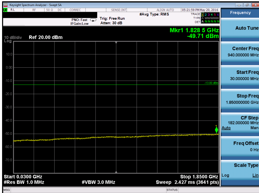
Plot 7-70. Conducted Spurious Plot (Band 2 – 20.0MHz QPSK – RB Size 1, RB Offset 0 – High Channel)
