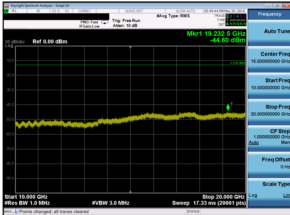
Plot 7-60. Conducted Spurious Plot (Band 4 – 20.0MHz QPSK – RB Size 1, RB Offset 0 – Mid Channel)
