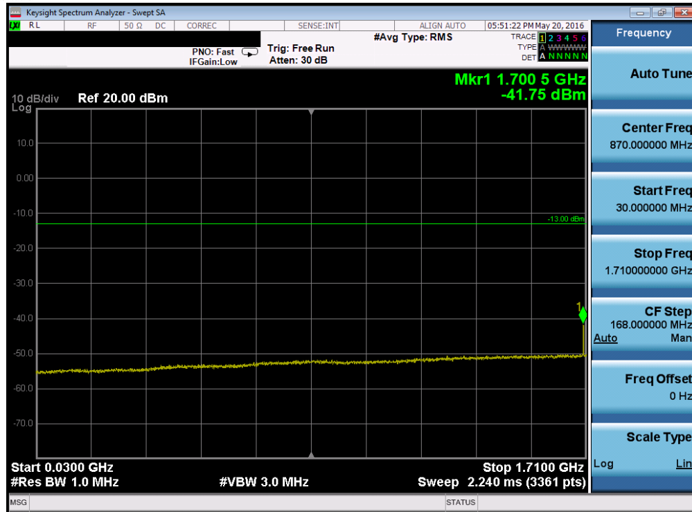
Plot 7-61. Conducted Spurious Plot (Band 4 – 20.0MHz QPSK – RB Size 1, RB Offset 0 – High Channel)
