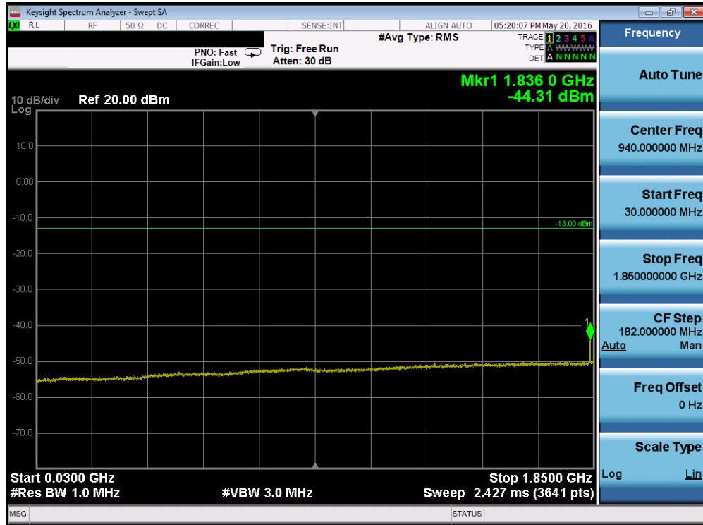
Plot 7-67. Conducted Spurious Plot (Band 2 – 20.0MHz QPSK – RB Size 1, RB Offset 0 – Mid Channel)
