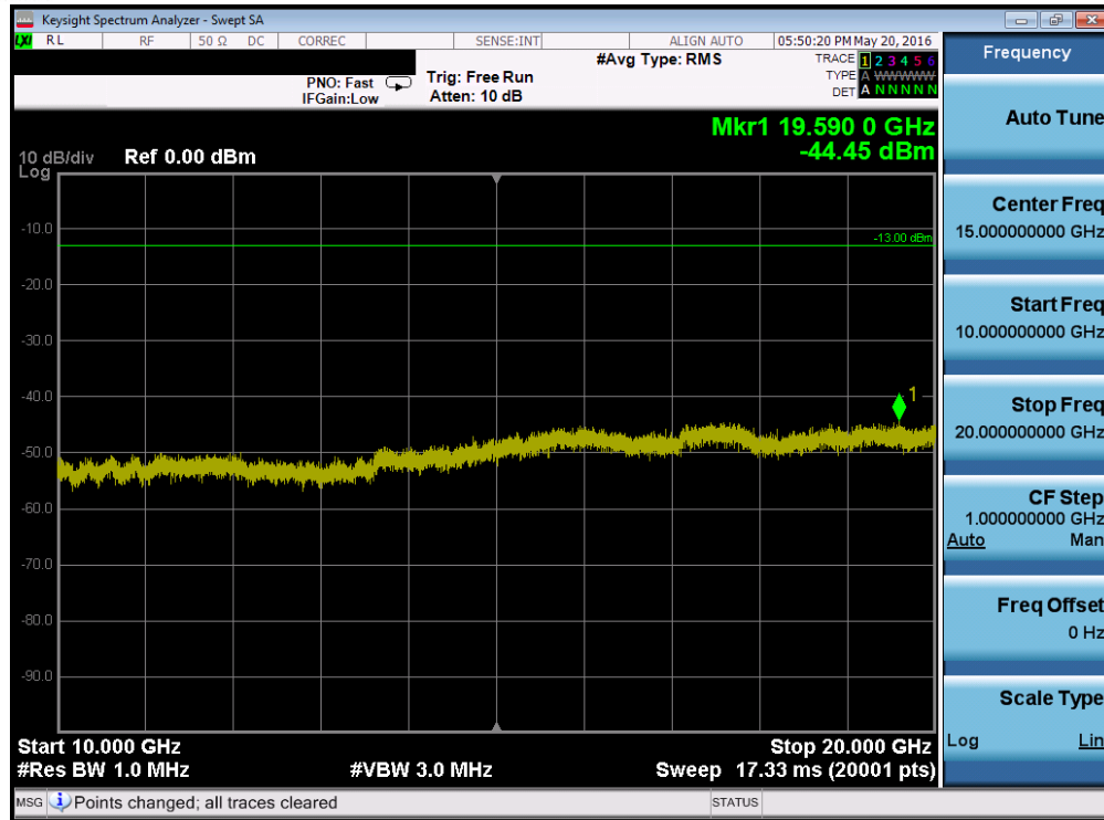
Plot 7-57. Conducted Spurious Plot (Band 4 – 20.0MHz QPSK – RB Size 1, RB Offset 0 – Low Channel)
