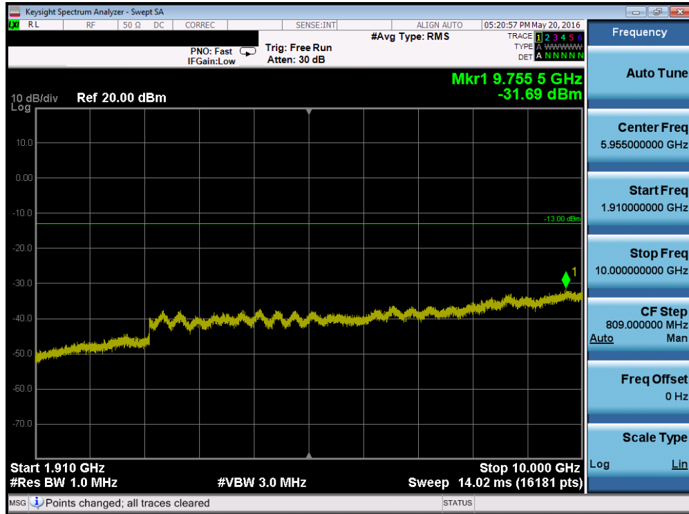
Plot 7-65. Conducted Spurious Plot (Band 2 – 20.0MHz QPSK – RB Size 1, RB Offset 0 – Low Channel)
