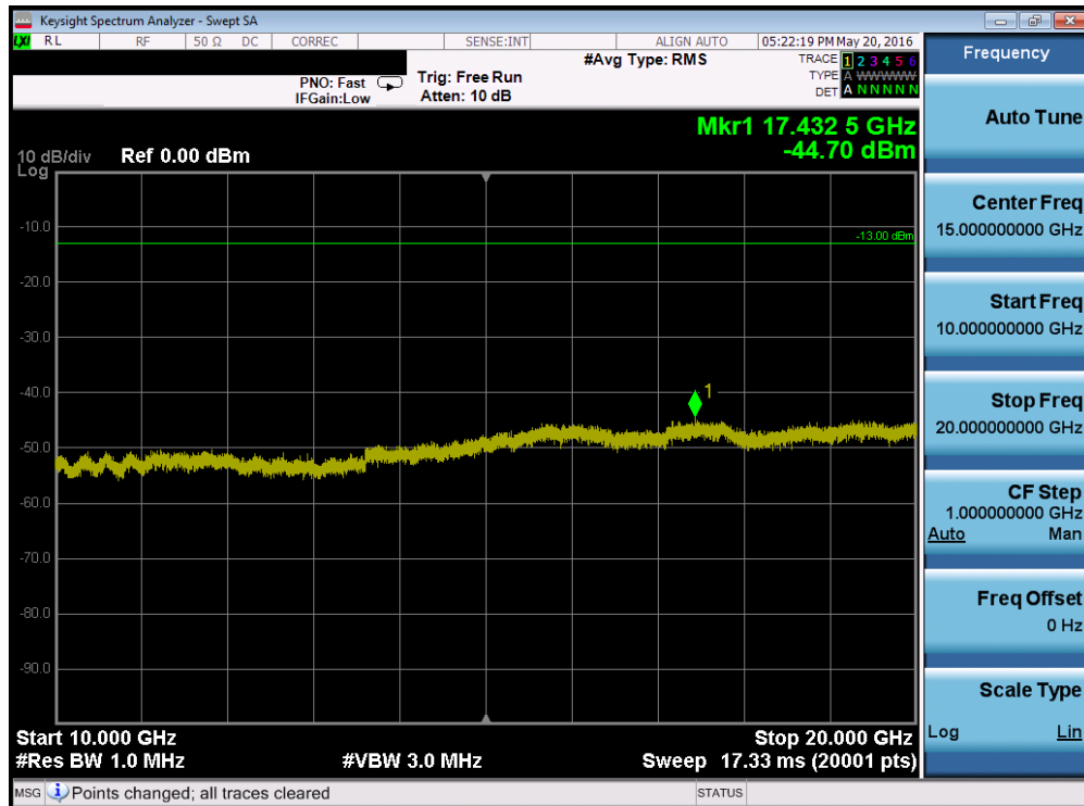
Plot 7-72. Conducted Spurious Plot (Band 2 – 20.0MHz QPSK – RB Size 1, RB Offset 0 – High Channel)
