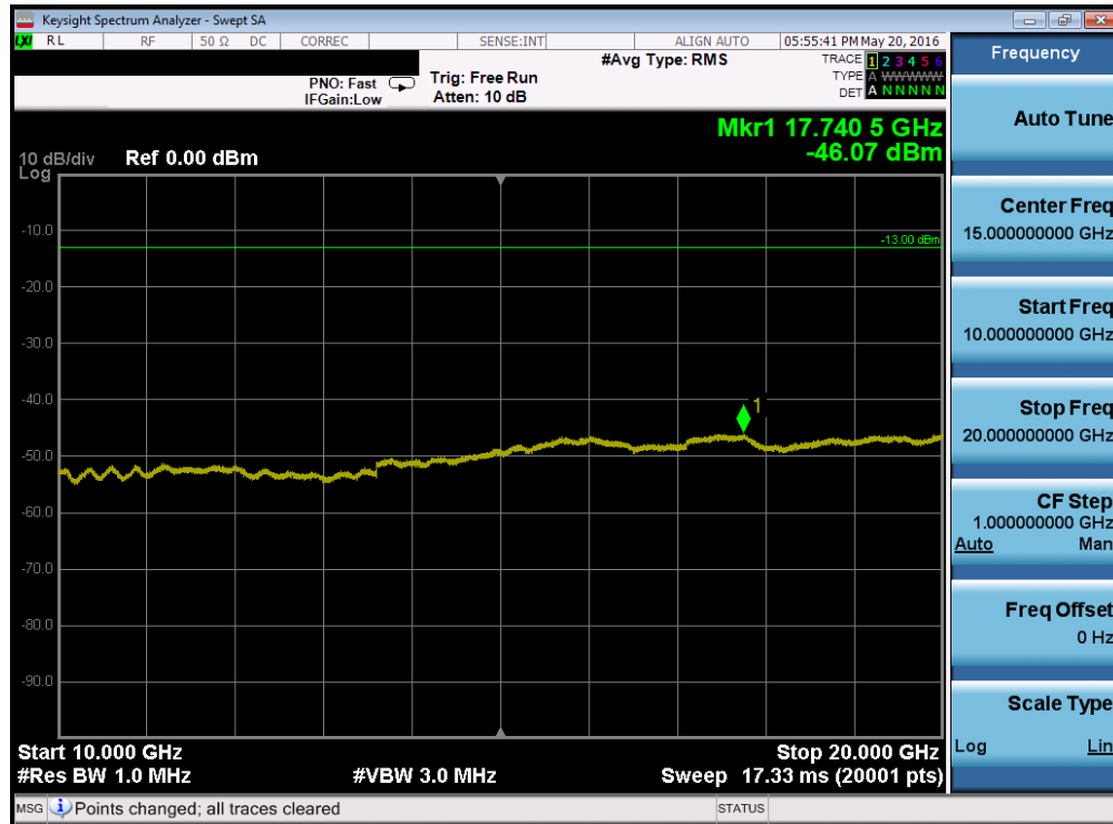
Plot 7-63. Conducted Spurious Plot (Band 4 – 20.0MHz QPSK – RB Size 1, RB Offset 0 – High Channel)
