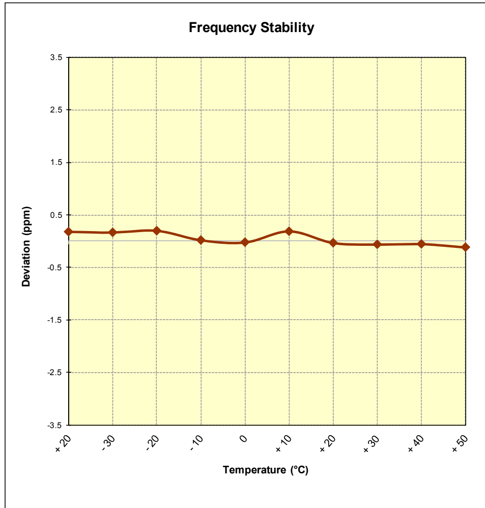
Figure 7-12. Frequency Stability Graph (PCS CDMA Mode – Ch. 600)
