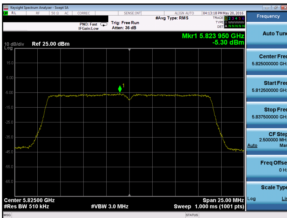
Plot 7-61. Power Spectral Density Plot (802.11a (UNII Band 3) – Ch. 165)
