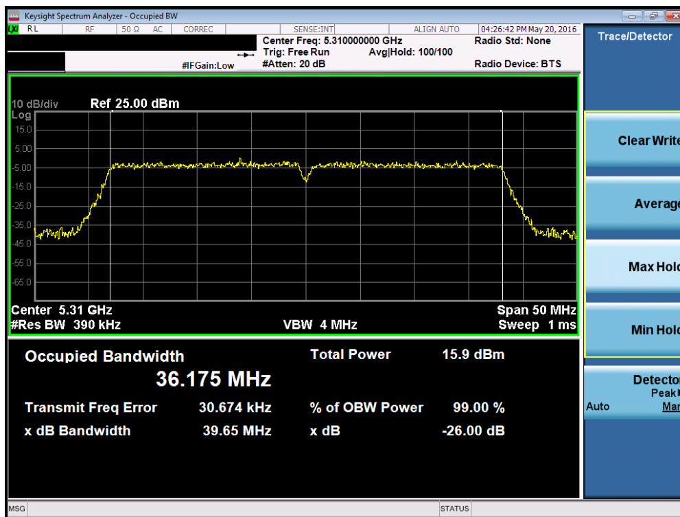
Plot 7-16. 26dB Bandwidth Plot (40MHz BW 802.11n (UNII Band 2A) – Ch. 62)
