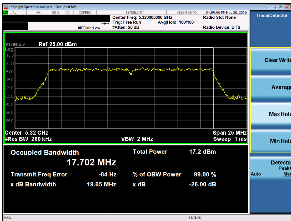
Plot 7-11. 26dB Bandwidth Plot (802.11a (UNII Band 2A) – Ch. 64)
