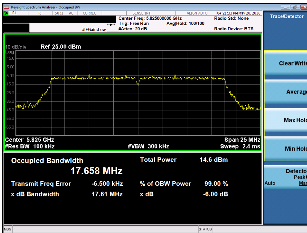
Plot 7-31. 6dB Bandwidth Plot (20MHz BW 802.11n (UNII Band 3) – Ch. 165)
