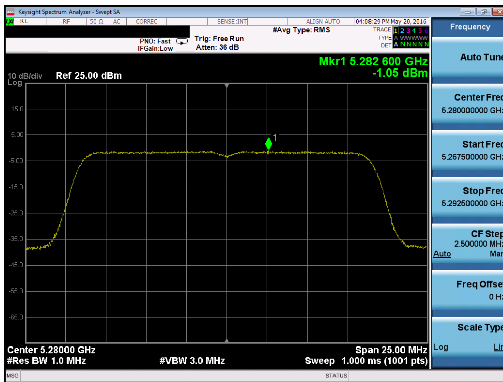
Plot 7-43. Power Spectral Density Plot (802.11a (UNII Band 2A) – Ch. 56)
