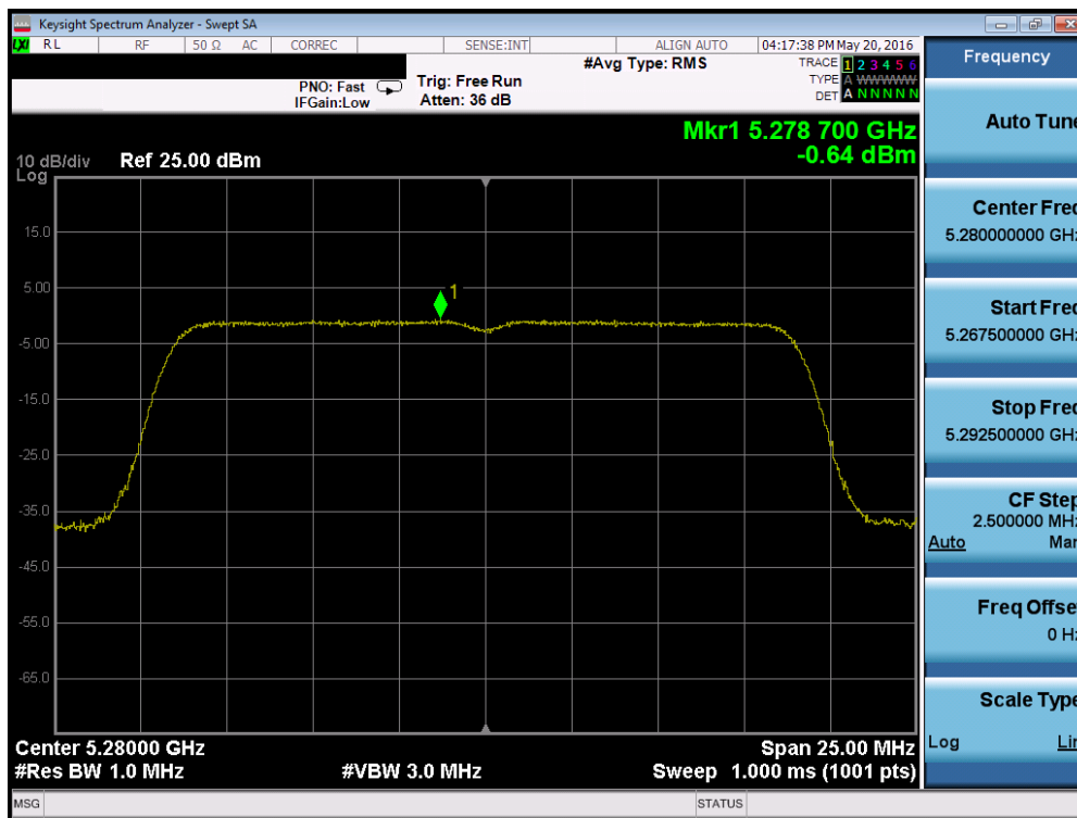
Plot 7-46. Power Spectral Density Plot (20MHz BW 802.11n (UNII Band 2A) – Ch. 56)
