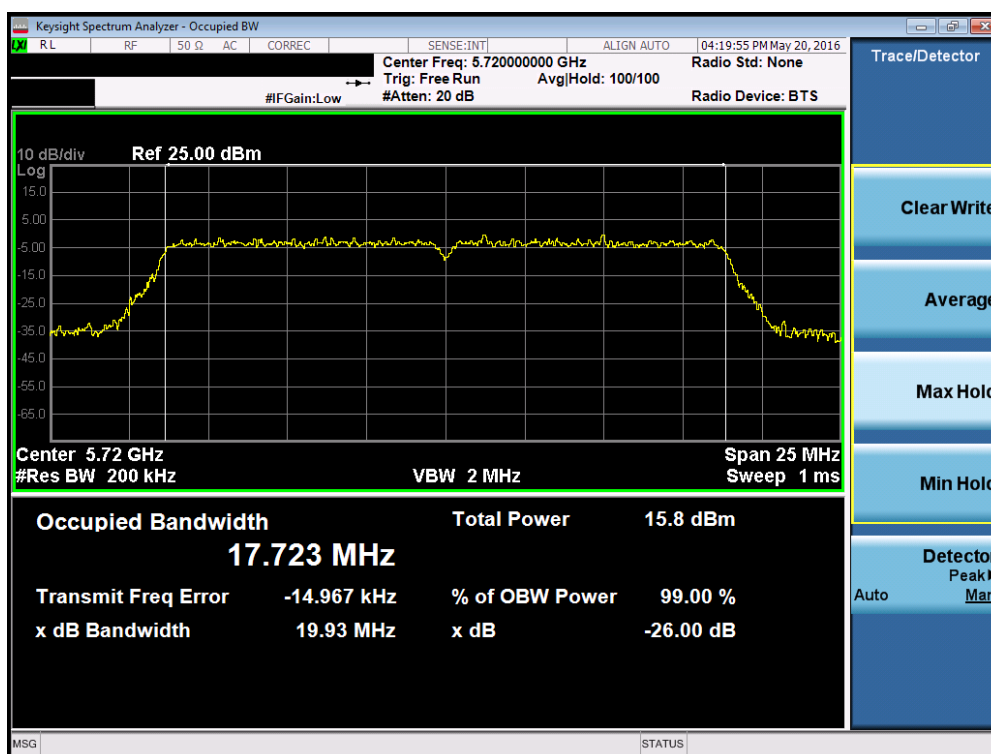
Plot 7-22. 26dB Bandwidth Plot (20MHz BW 802.11n (UNII Band 2C) – Ch. 144)
