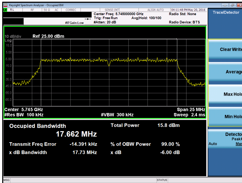
Plot 7-26. 6dB Bandwidth Plot (802.11a/n (UNII Band 3) – Ch. 149)
