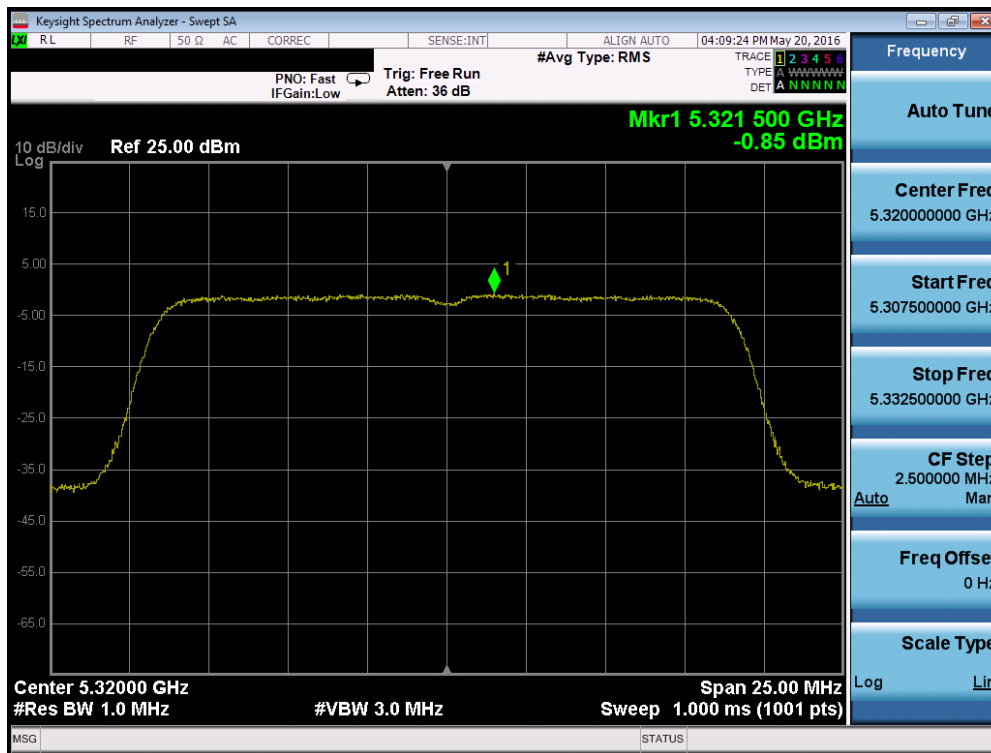
Plot 7-44. Power Spectral Density Plot (802.11a (UNII Band 2A) – Ch. 64)
