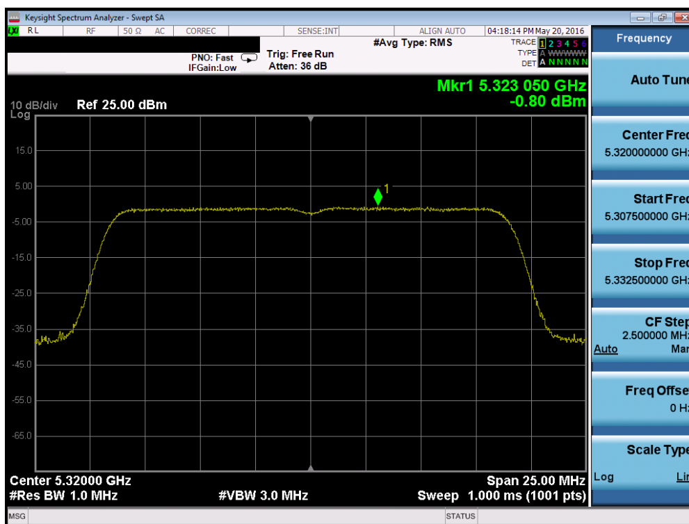
Plot 7-47. Power Spectral Density Plot (20MHz BW 802.11n (UNII Band 2A) – Ch. 64)
