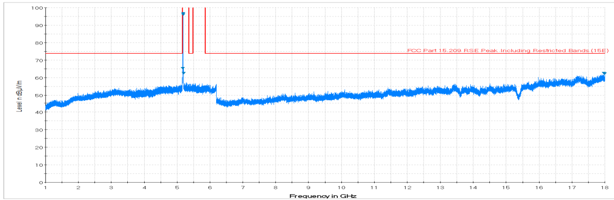
Plot 7-68. Radiated Spurious Plot above 1GHz (802.11a – U1 Ch. 40, Ant. Pol. V)
