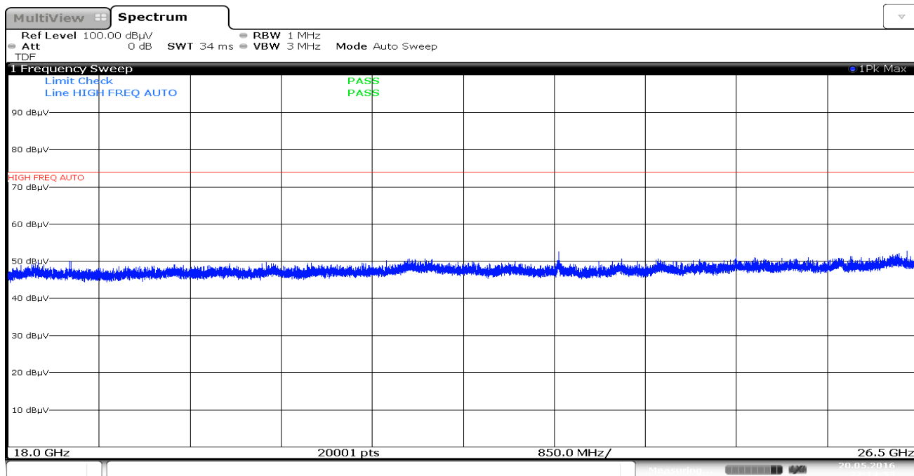
Plot 7-76. Radiated Spurious Plot above 18GHz (802.11a – Ant. Pol. V)
