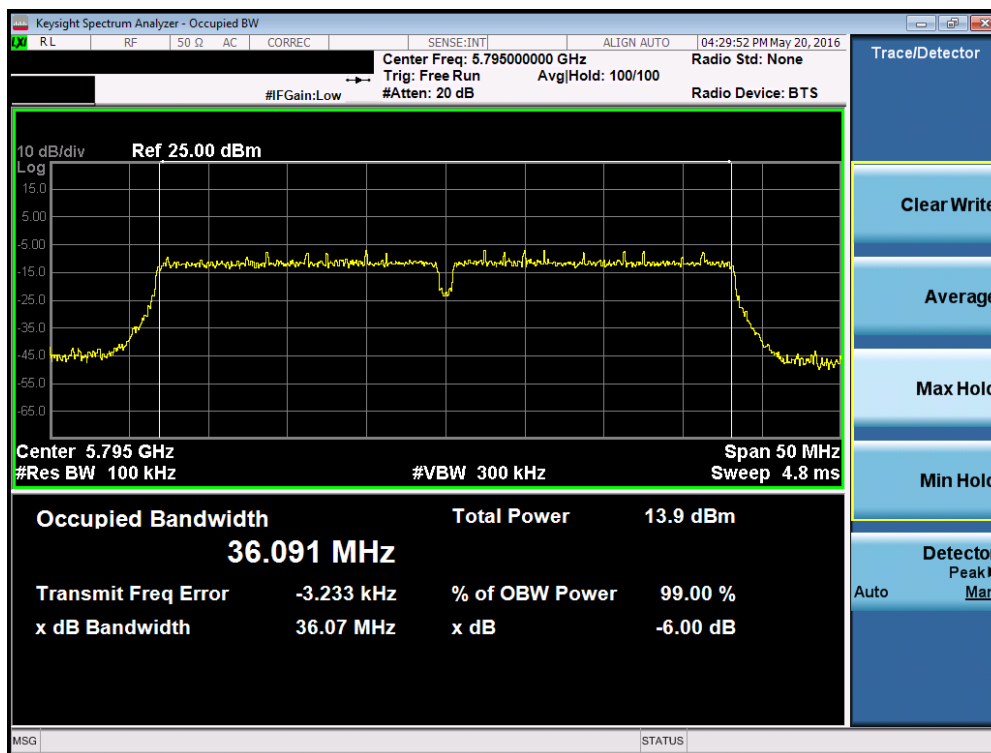
Plot 7-33. 6dB Bandwidth Plot (40MHz BW 802.11n (UNII Band 3) – Ch. 159)
