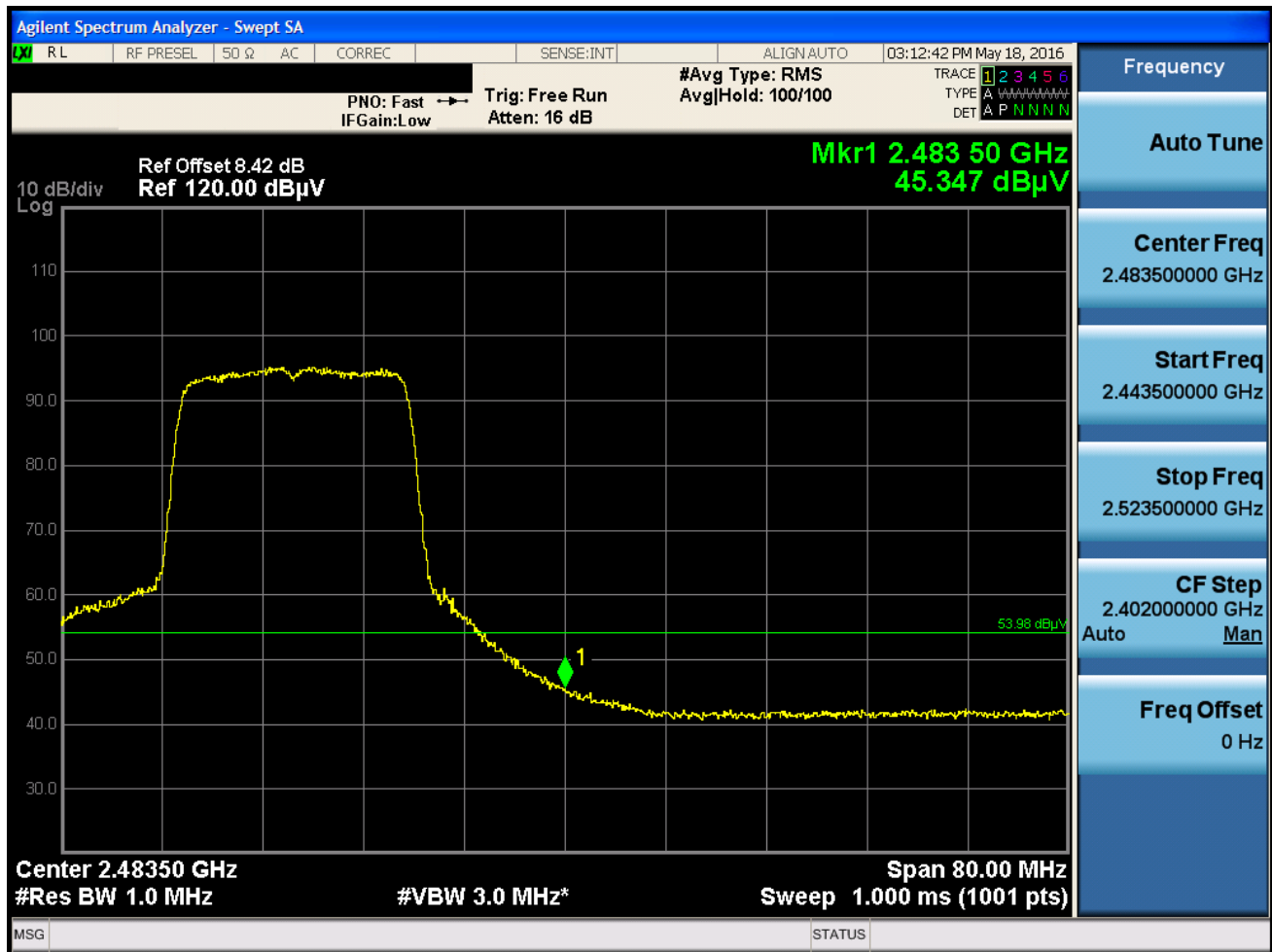
Plot 7-41. Radiated Restricted Upper Band Edge Measurement (Average)
