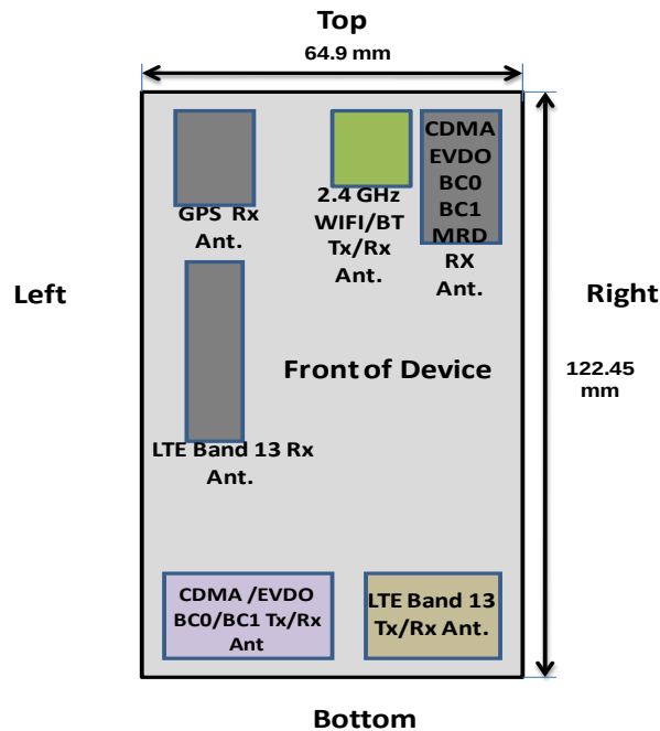
Figure 1-1 DUT Antenna Locations
