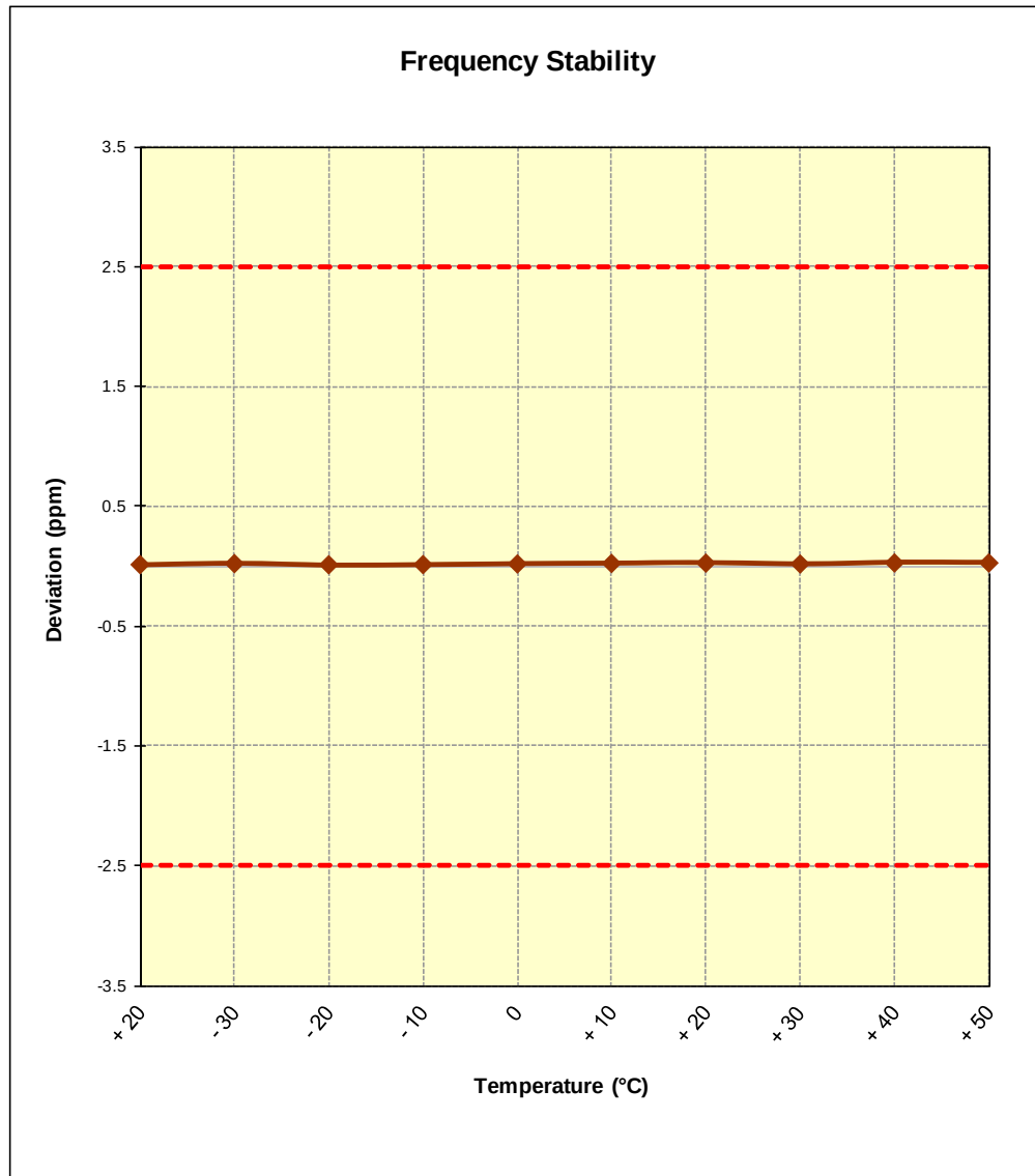
Figure 6-1. Frequency Stability Graph (Cellular CDMA Mode – Ch. 384)
