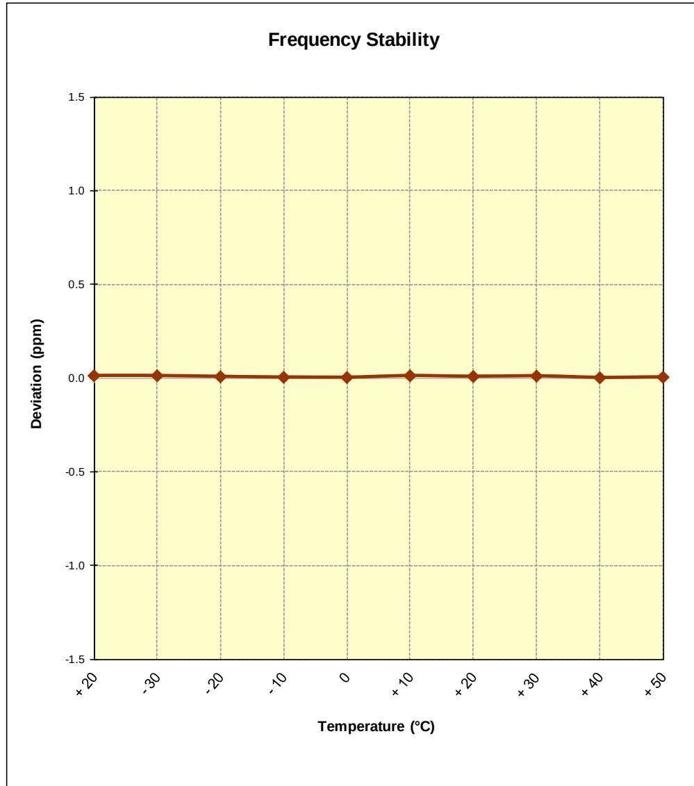
Figure 6-2. Frequency Stability Graph (PCS CDMA Mode – Ch. 600)
