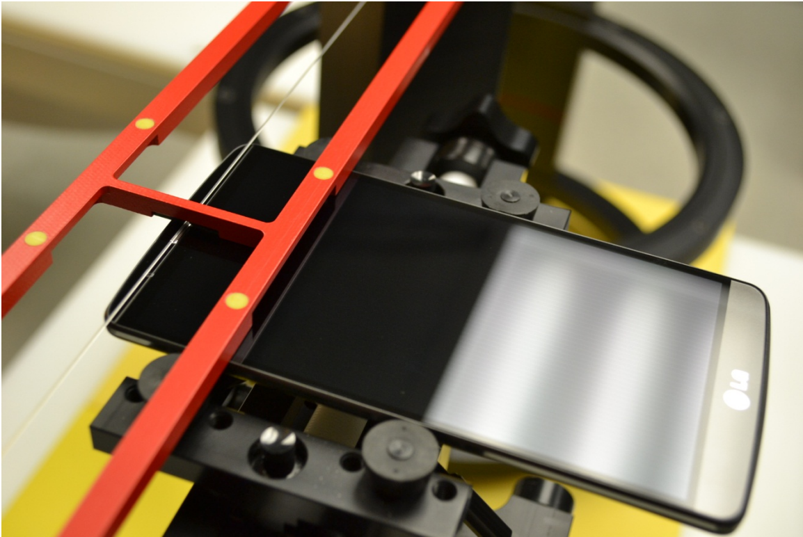
Setup Photo (Wireless Charging Cover)
