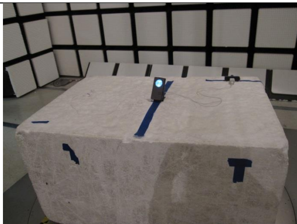
RADIATED EMISSION Smart Cover and Dock PHOTO
