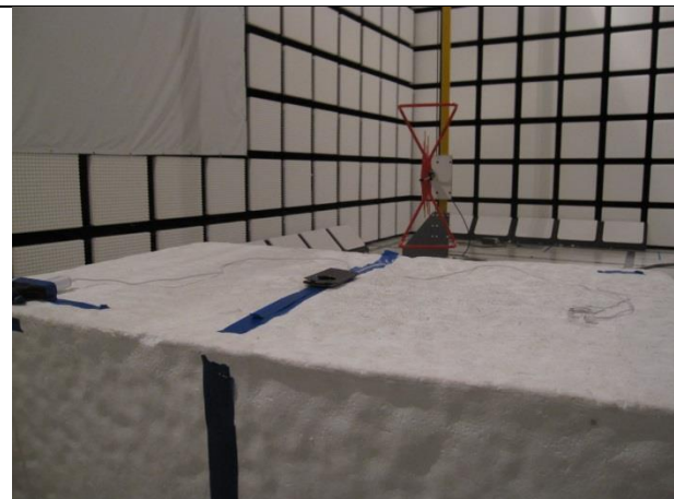
RADIATED EMISSION Smart Cover PHOTO
