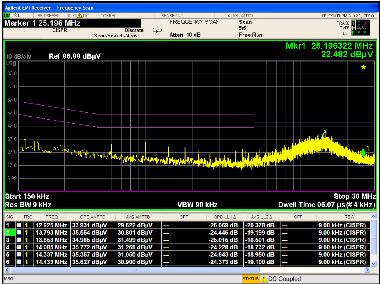
Plot 7-30. Line Conducted Plot with Bluetooth LE (L1)
