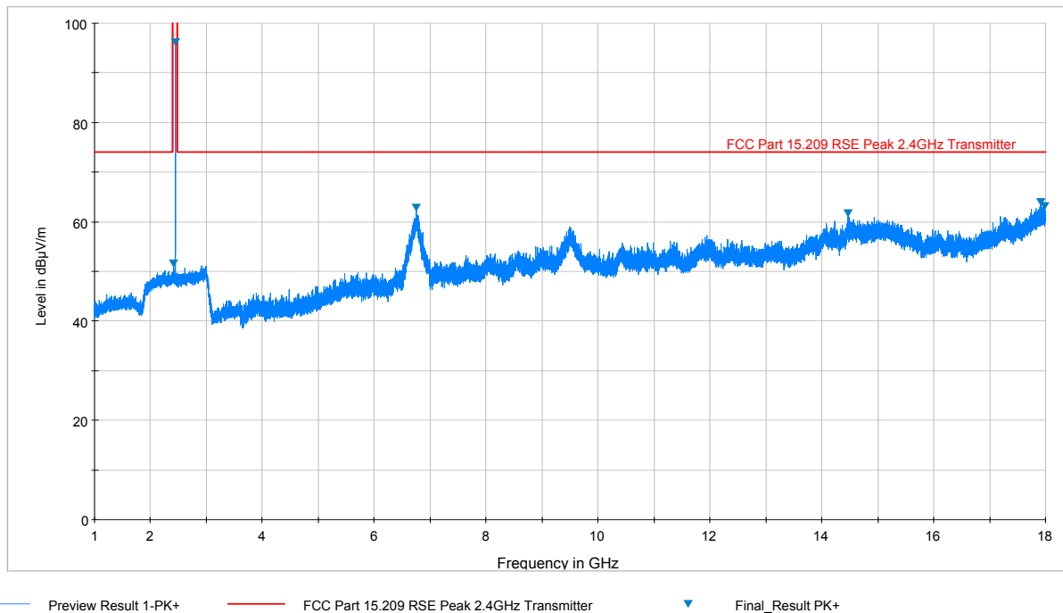
Plot 7-21. Radiated Spurious Plot above 1GHz (BT LE – Ch. 19, Ant. Pol. V)
