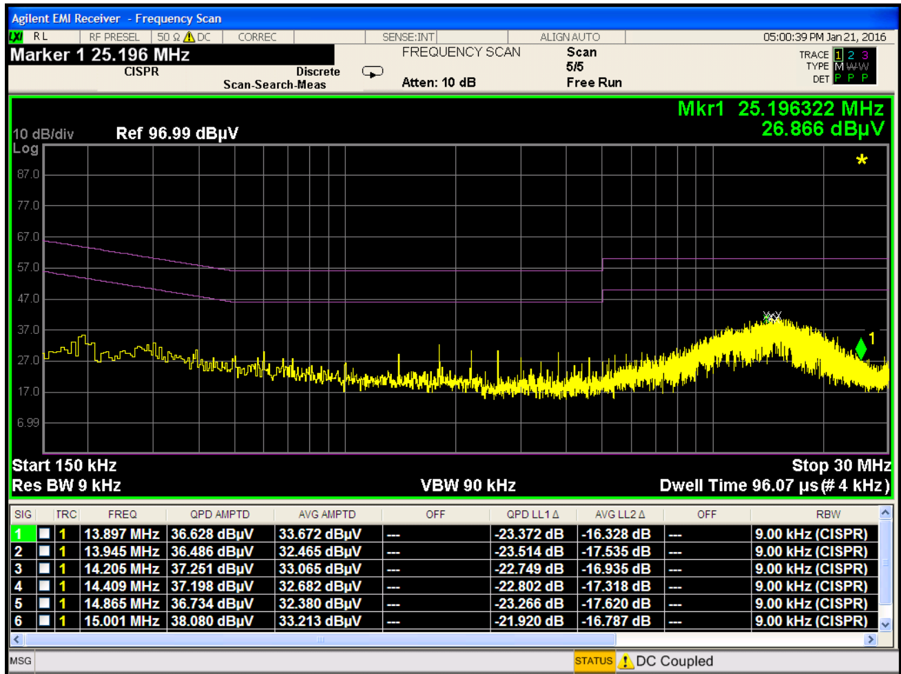
Plot 7-31. Line Conducted Plot with Bluetooth LE (N)
