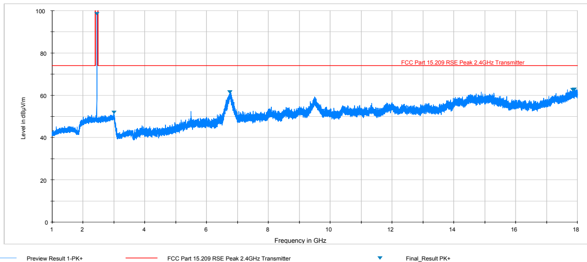
Plot 7-20. Radiated Spurious Plot above 1GHz (BT LE – Ch. 19, Ant. Pol. H)
