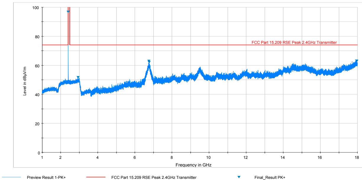
Plot 7-18. Radiated Spurious Plot above 1GHz (BT LE – Ch. 0, Ant. Pol. H)
