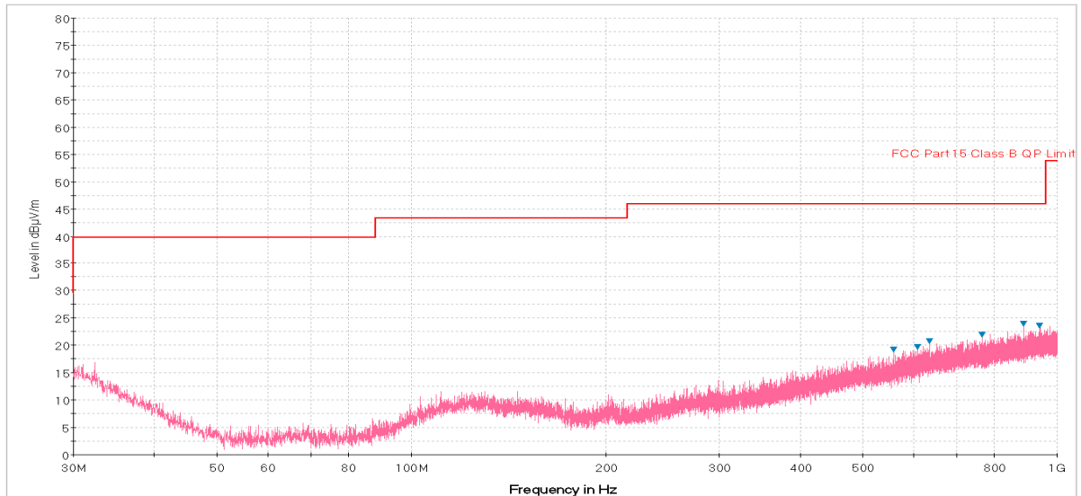
Plot 7-28. Radiated Spurious Plot below 1GHz (Pol. H)
