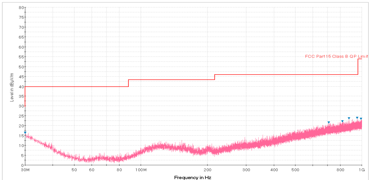
Plot 7-29. Radiated Spurious Plot below 1GHz (Pol. V)
