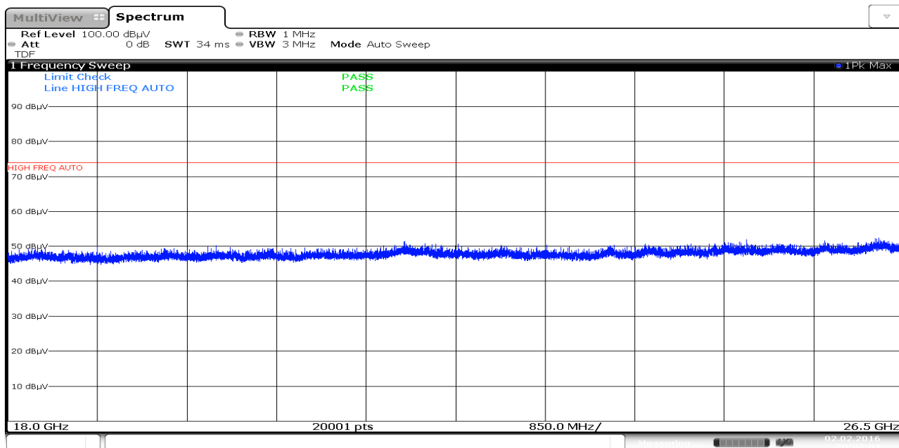
Plot 7-24. Radiated Spurious Plot above 18GHz (Pol. H)
