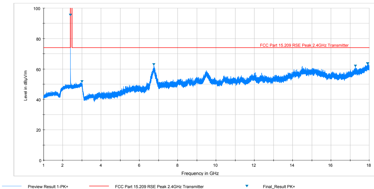
Plot 7-19. Radiated Spurious Plot above 1GHz (BT LE – Ch. 0, Ant. Pol. V)
