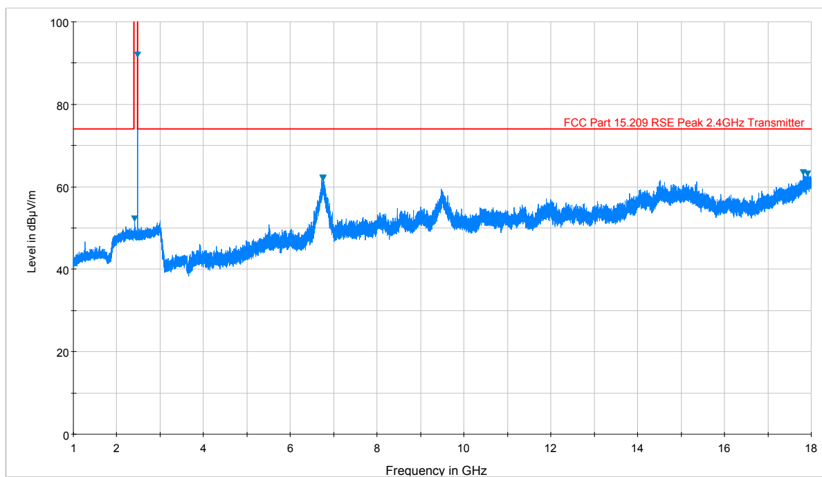
Plot 7-23. Radiated Spurious Plot above 1GHz (BT LE – Ch. 39, Ant. Pol. V)
