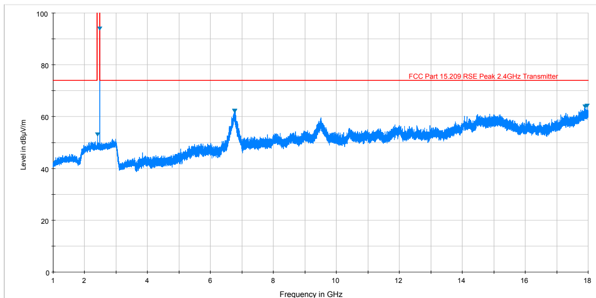
Plot 7-22. Radiated Spurious Plot above 1GHz (BT LE – Ch. 39, Ant. Pol. H)
