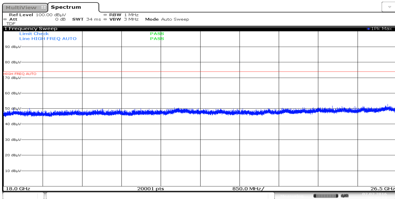
Plot 7-25. Radiated Spurious Plot above 18GHz (Pol. V)
