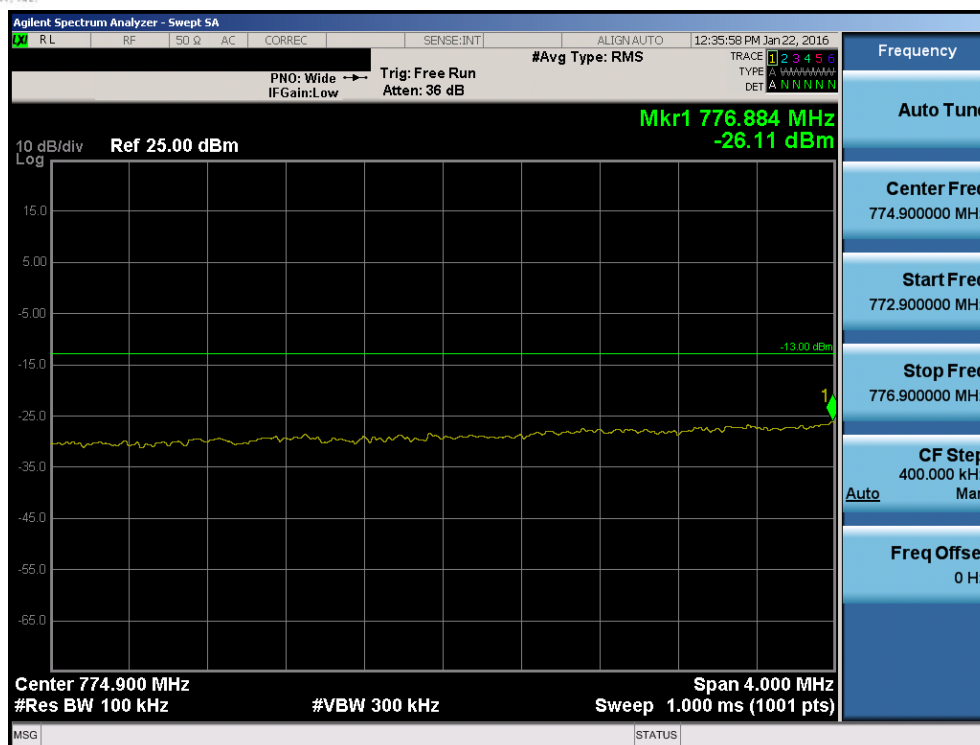
Plot 7-2. Lower Extended Band Edge Plot (Band 13 – 5.0MHz QPSK – RB Size 25)
