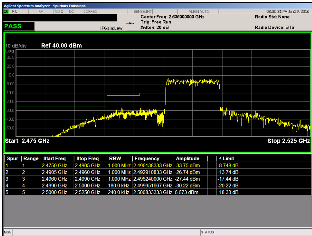
Plot 7-231. Lower ACP Plot (Band 7 – 10.0MHz QPSK – RB Size 50)
