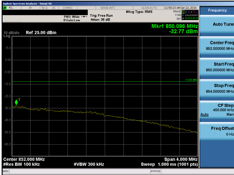
Plot 7-148. Upper Extended Band Edge Plot (Band 5 – Band 5 – 3.0MHz QPSK – RB Size 15)
