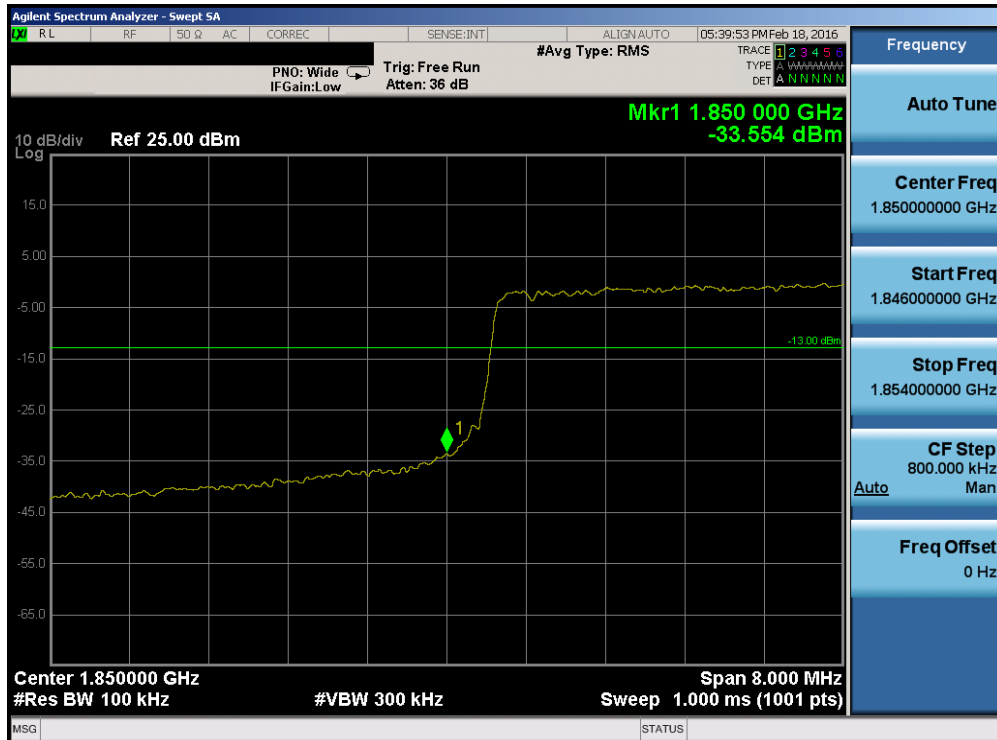
Plot 7-217. Lower Band Edge Plot (Band 25 – 10.0MHz QPSK – RB Size 50)
