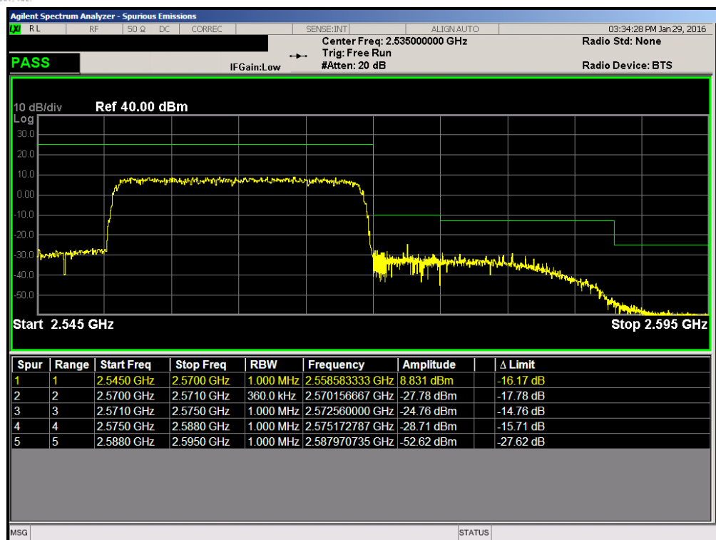
Plot 7-236. Upper ACP Plot (Band 7 – 20.0MHz QPSK – RB Size 100)
