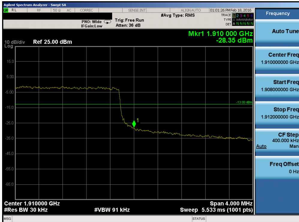
Plot 7-191. Upper Band Edge Plot (Band 2 – 5.0MHz QPSK – RB Size 25)
