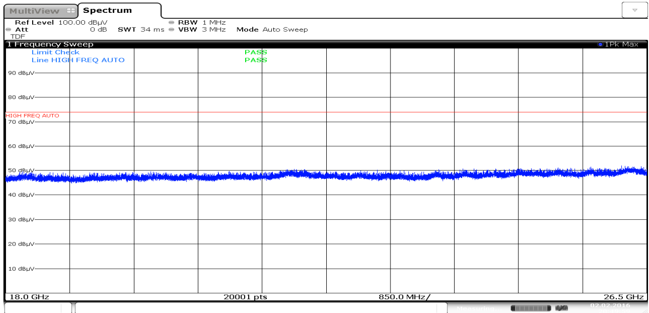
Plot 7-49. Radiated Spurious Plot above 18GHz (Pol. V)
