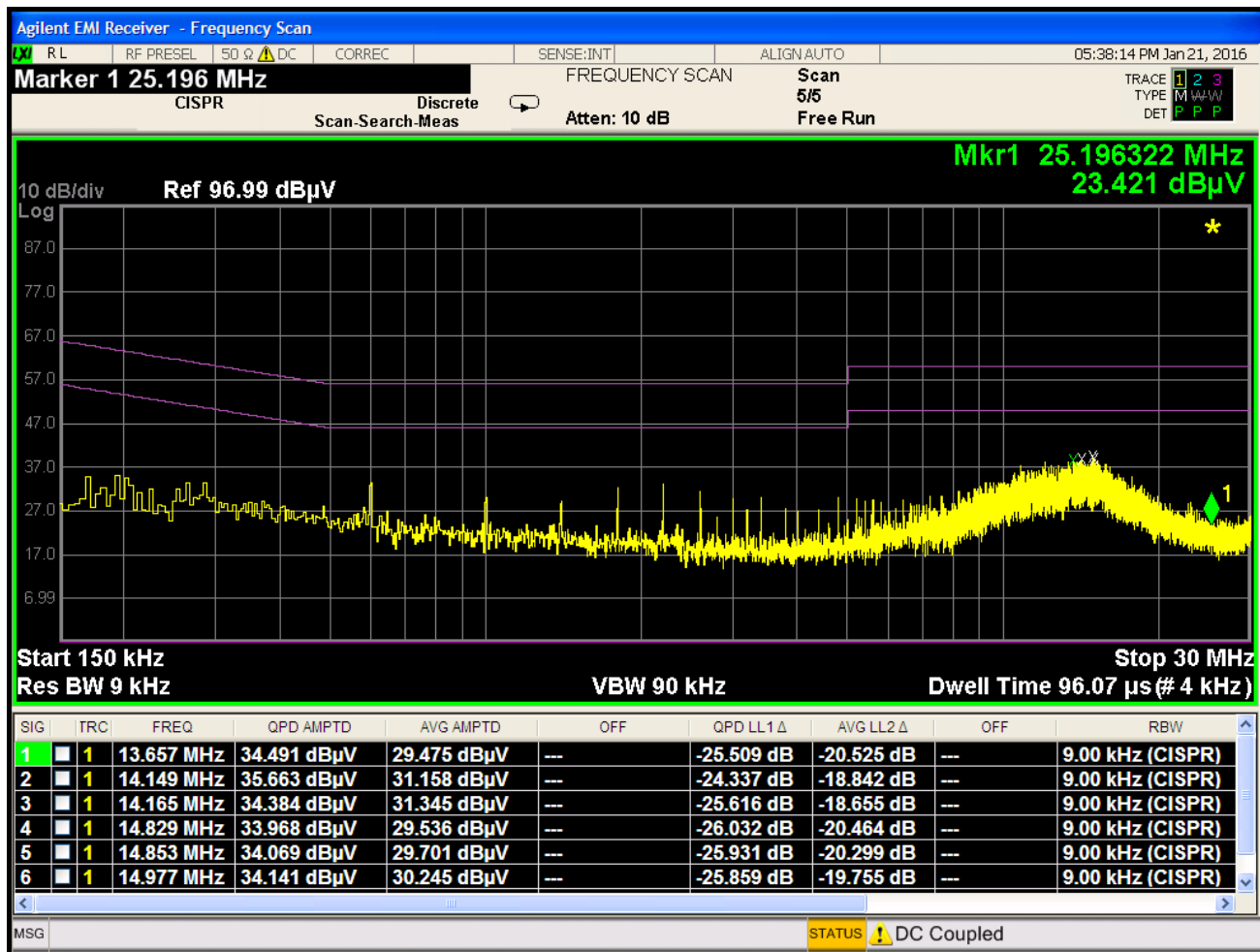
Plot 7-122. Line Conducted Plot with 802.11a UNII Band 2C (L1)
