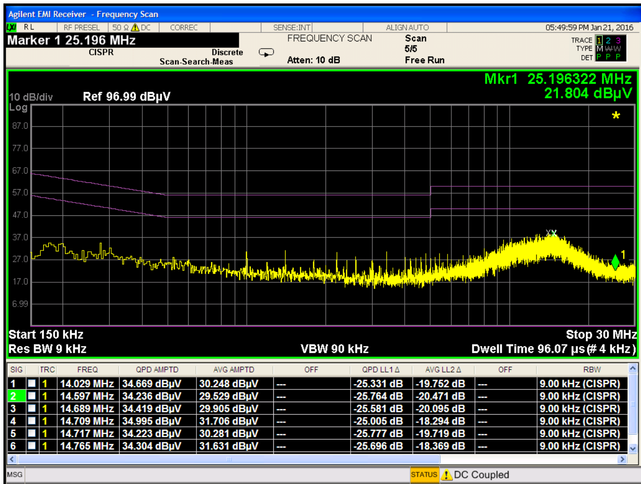
Plot 7-124. Line Conducted Plot with 802.11a UNII Band 3 (L1)
