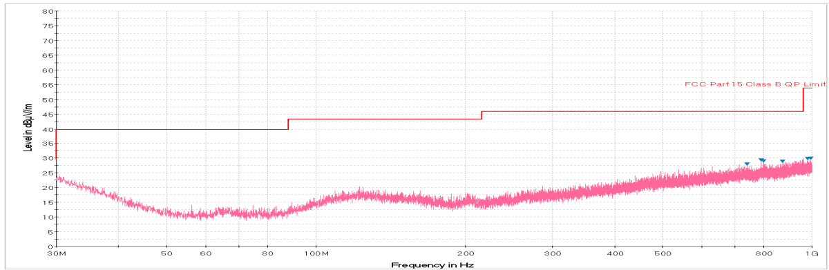
Plot 7-117. Radiated Spurious Plot below 1GHz (802.11a – U3 Ch. 157, Ant. Pol. V)
