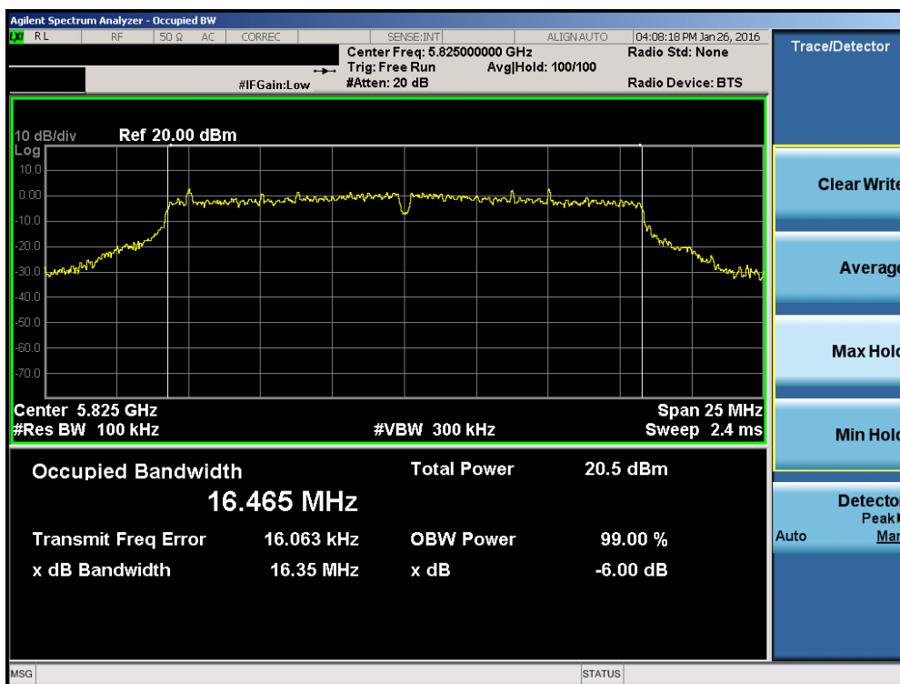
Plot 7-32. 6dB Bandwidth Plot (802.11a (UNII Band 3) – Ch. 165)
