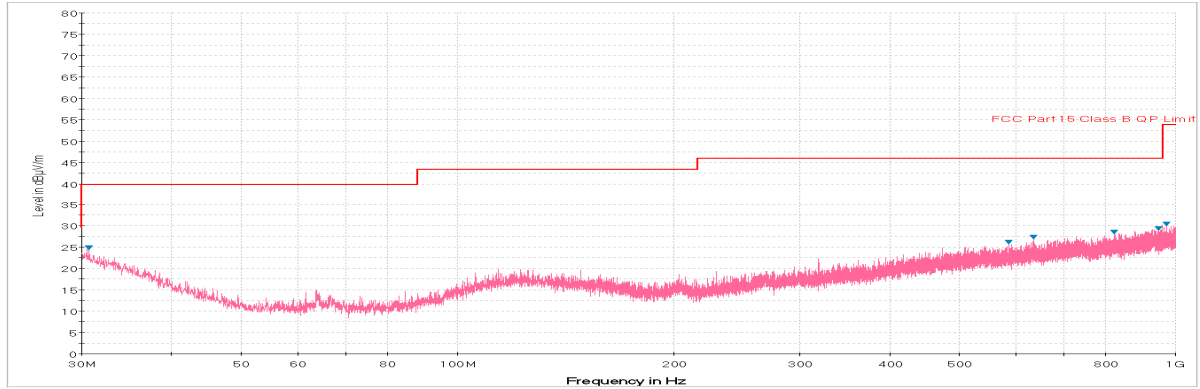
Plot 7-116. Radiated Spurious Plot below 1GHz (802.11a – U3 Ch. 157, Ant. Pol. H)
