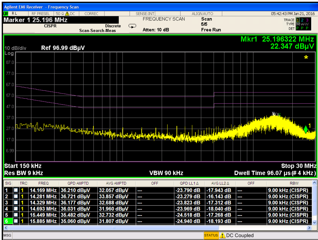
Plot 7-123. Line Conducted Plot with 802.11a UNII Band 2C (N)
