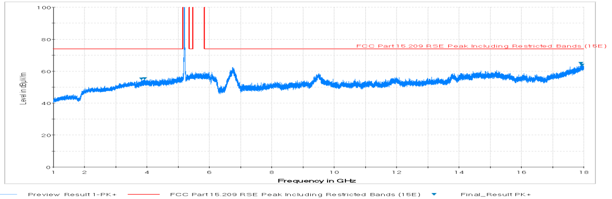
Plot 7-77. Radiated Spurious Plot above 1GHz (802.11a – U1 Ch. 40, Ant. Pol. H)
