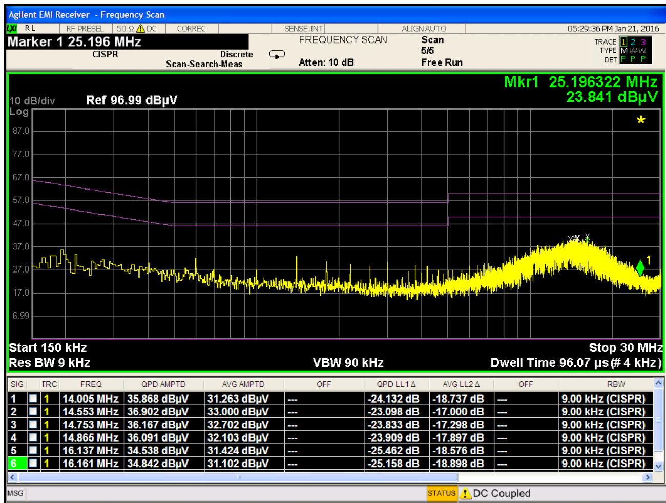
Plot 7-121. Line Conducted Plot with 802.11a UNII Band 2A (N)
