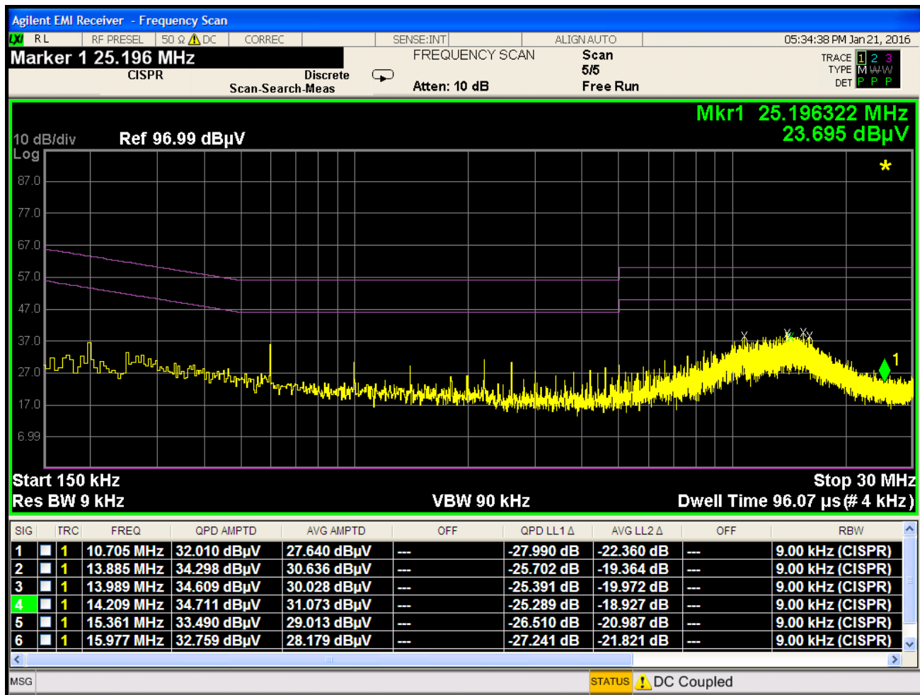
Plot 7-120. Line Conducted Plot with 802.11a UNII Band 2A (L1)
