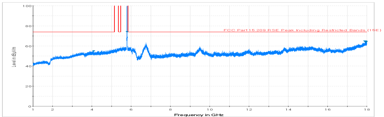
Plot 7-84. Radiated Spurious Plot above 1GHz (802.11a – U3 Ch. 157, Ant. Pol. V)
