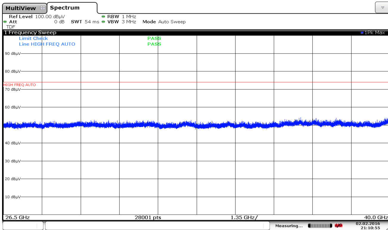
Plot 7-88. Radiated Spurious Plot above 26GHz (802.11a – Ant. Pol. V)
