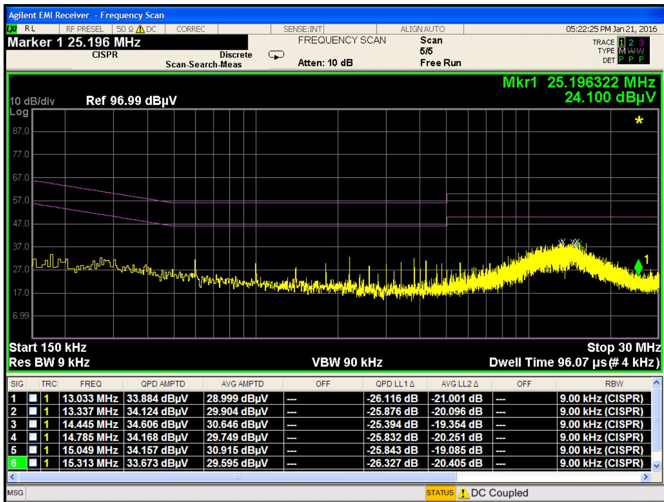
Plot 7-118. Line Conducted Plot with 802.11a UNII Band 1 (L1)
