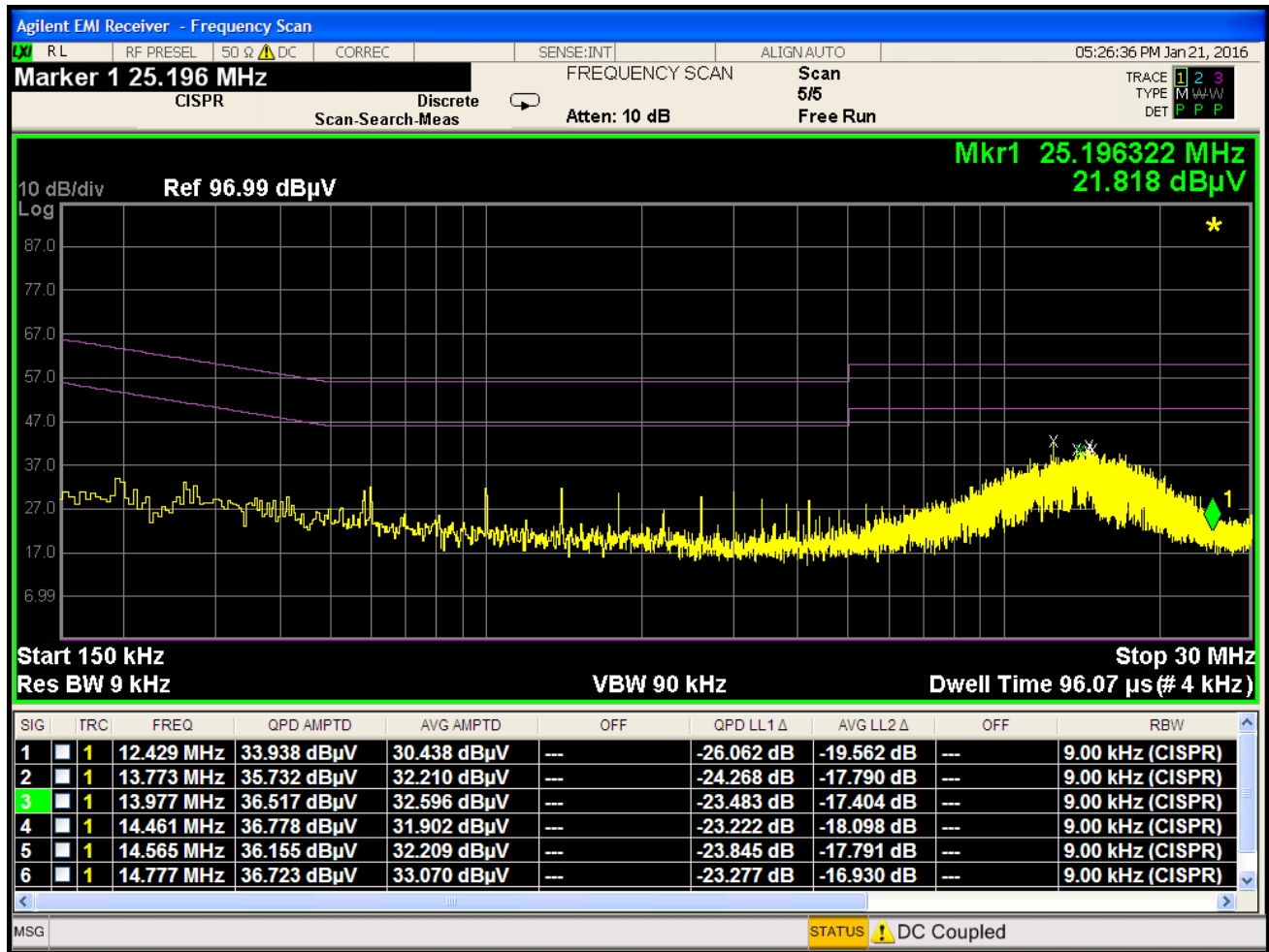
Plot 7-119. Line Conducted Plot with 802.11a UNII Band 1 (N)
