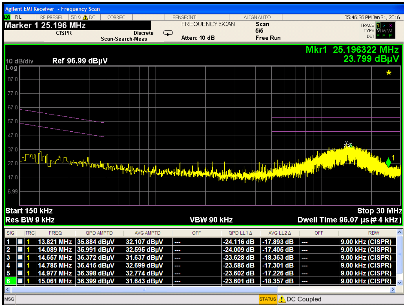
Plot 7-125. Line Conducted Plot with 802.11a UNII Band 3 (N)
