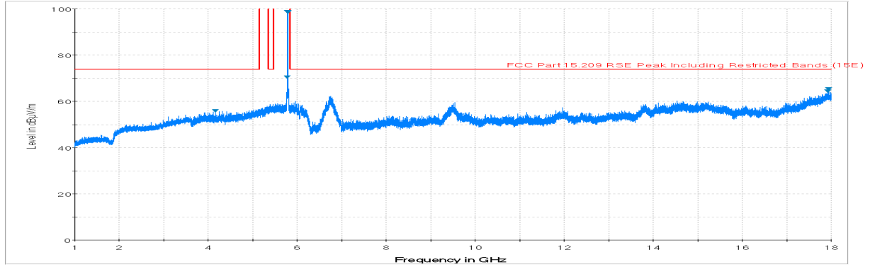
Plot 7-83. Radiated Spurious Plot above 1GHz (802.11a – U3 Ch. 157, Ant. Pol. H)
