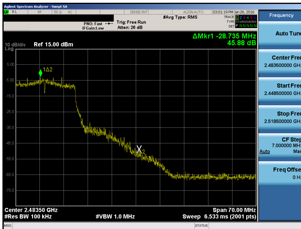
Plot 7-29. Band Edge Plot (802.11n - Ch. 10)
