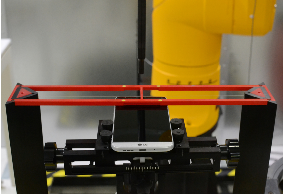
Figure 18-1 Ear Reference Point HAC Phantom Alignment
