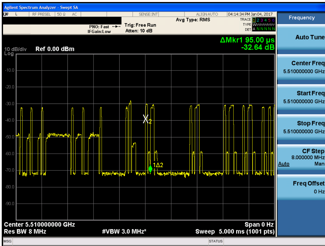
Figure 5-4. Band 2C Period
