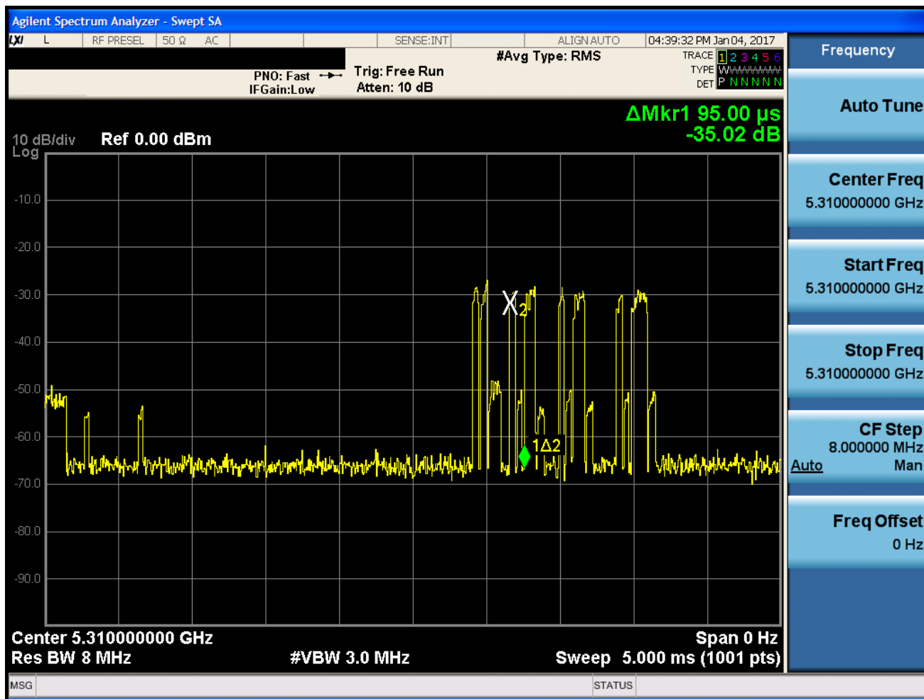
Figure 5-2. Band 2A Period
