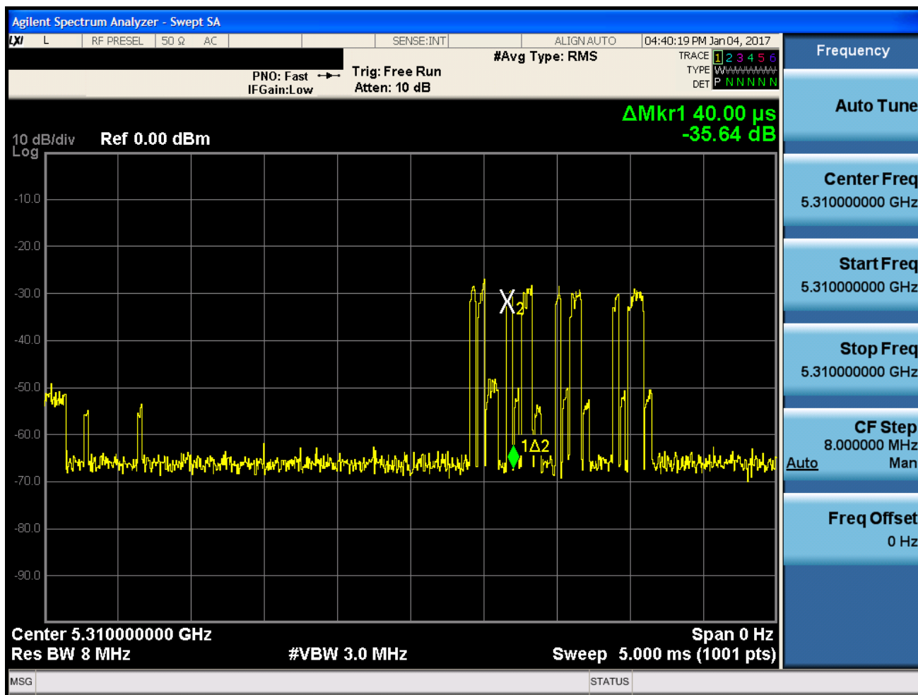
Figure 5-1. Band 2A Pulse Width
