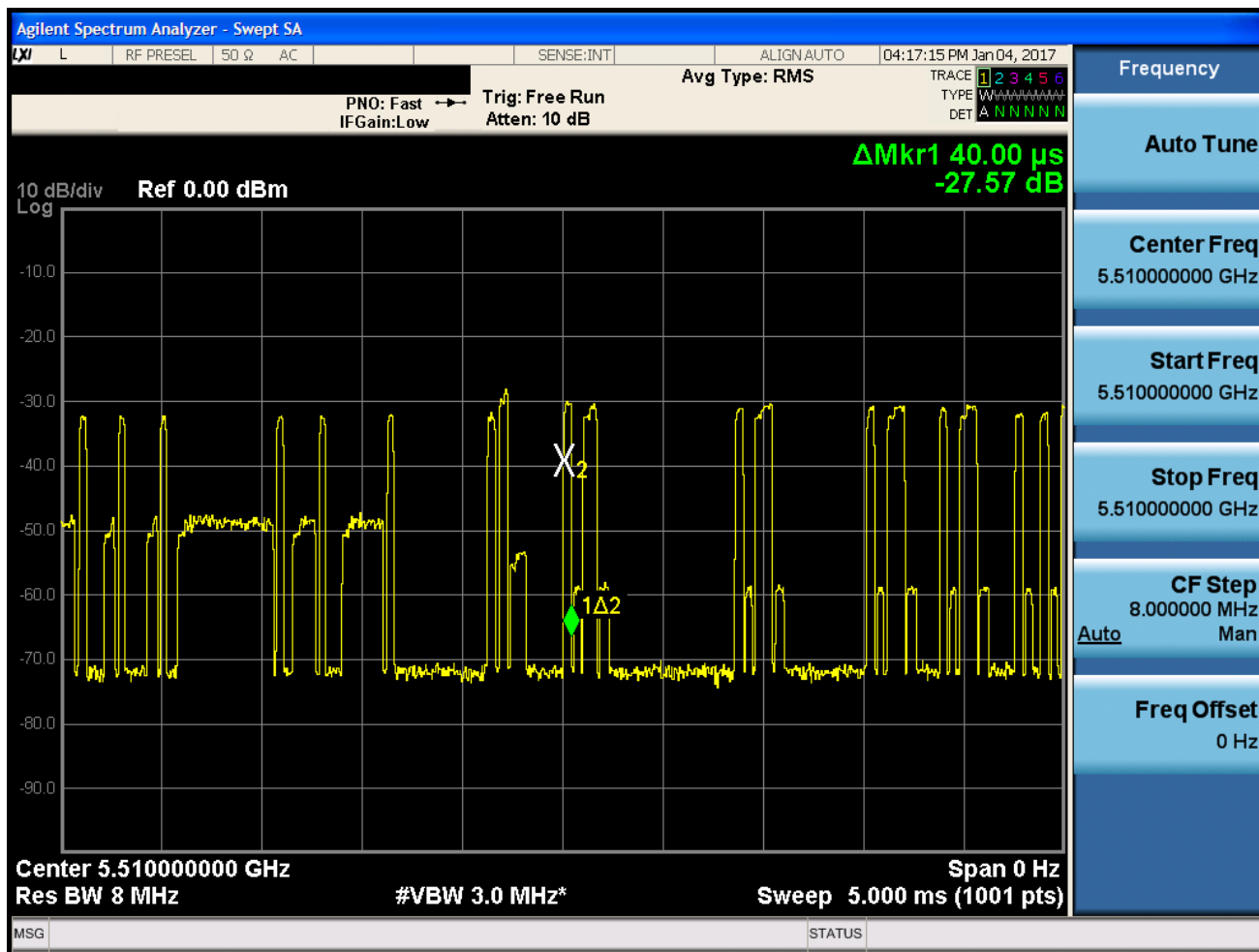
Figure 5-3. Band 2C Pulse Width
