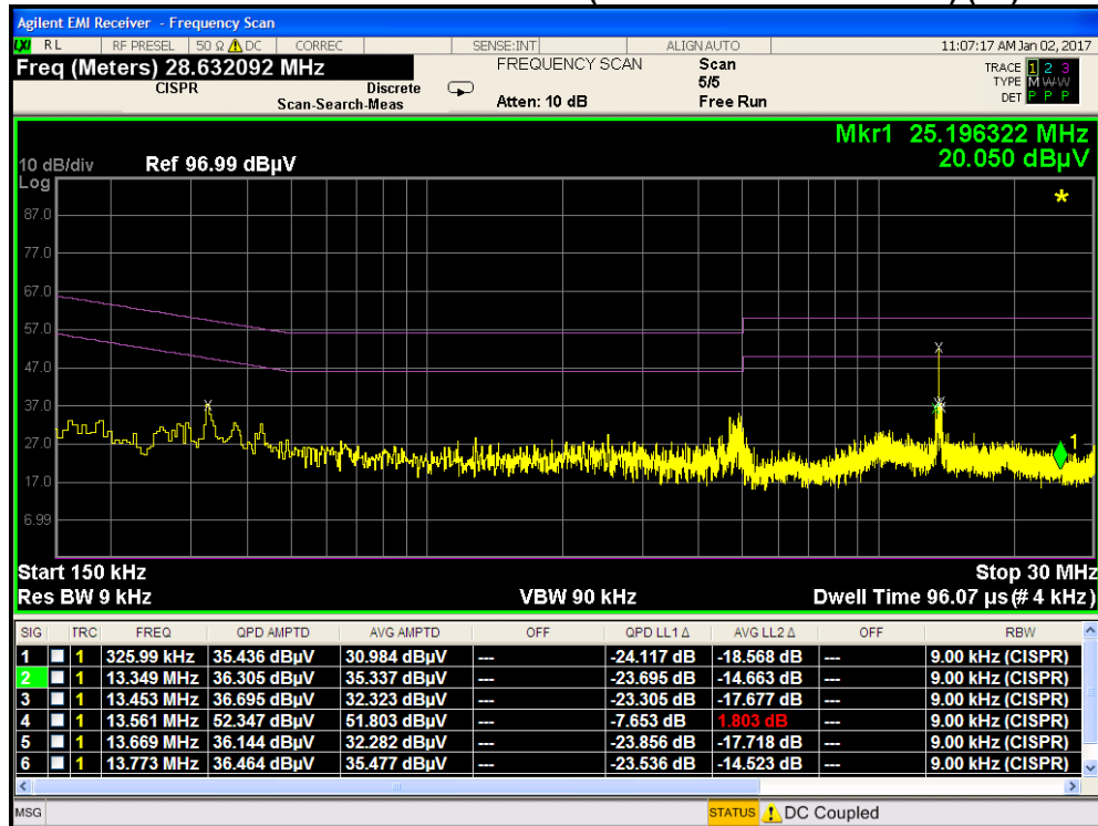
Plot 8-2. Line-Conducted Test Plot (With Antenna Connected) (N)
