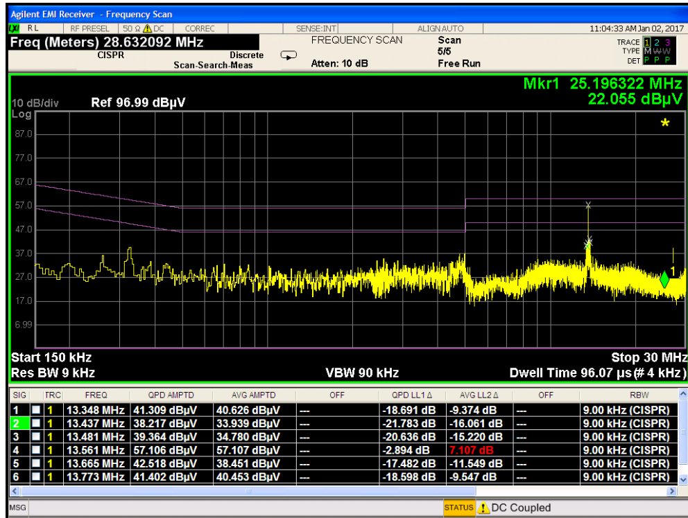
Plot 8-1. Line-Conducted Test Plot (With Antenna Connected) (L1)
