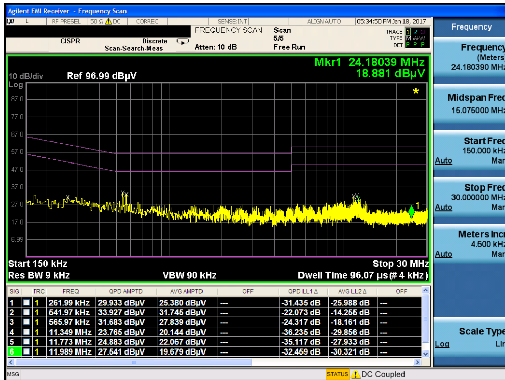
Plot 8-4. Line-Conducted Test Plot (With Antenna Terminated In 50Ω) (N)
