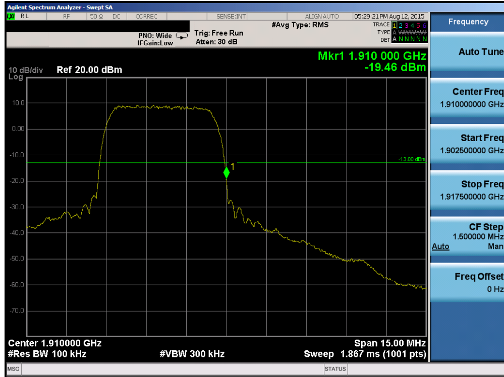
Plot 6-81. Band Edge Plot (PCS WCDMA Mode – Ch. 9538)
