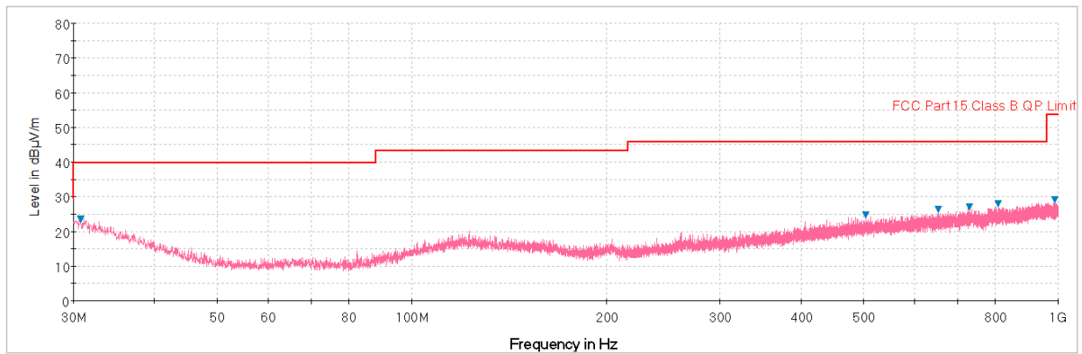
Plot 6-55. Radiated Spurious Plot below 1GHz (Pol. V)
