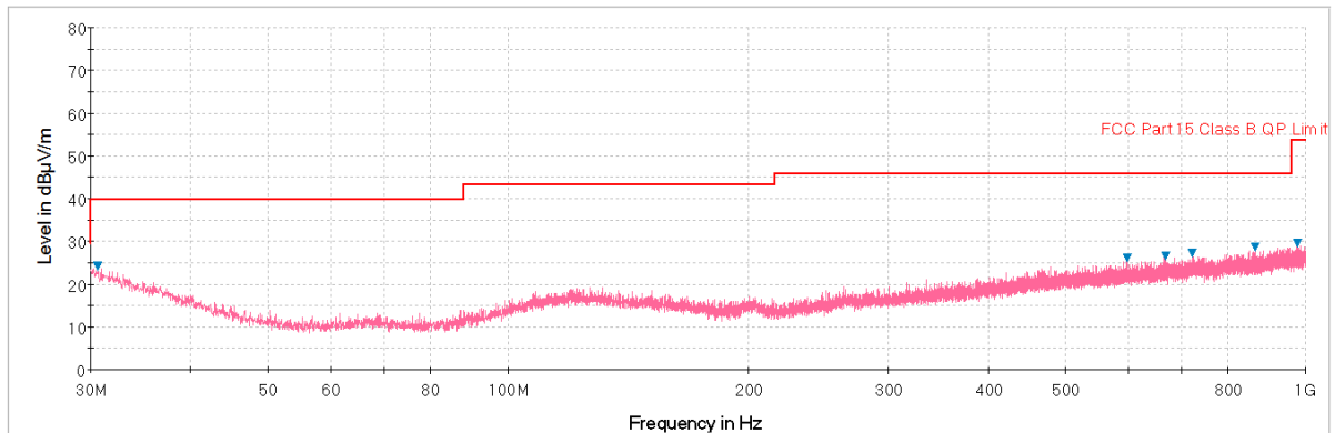
Plot 6-54. Radiated Spurious Plot below 1GHz (Pol. H)
