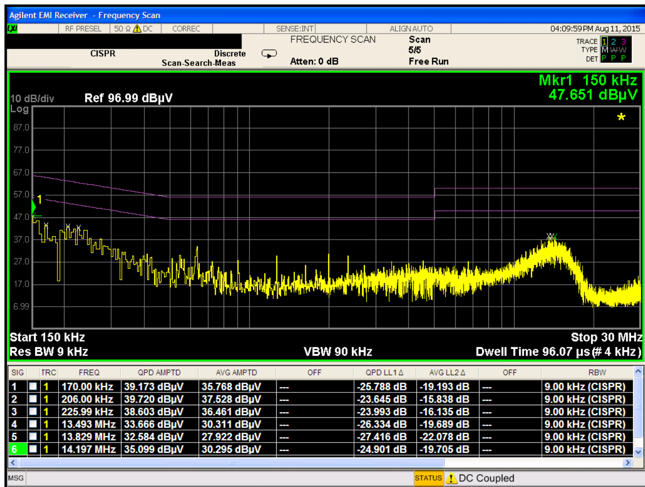
Plot 6-57. Line-Conducted Test Plot (N)
