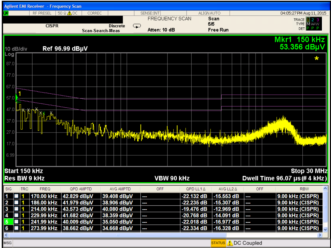
Plot 6-56. Line-Conducted Test Plot (L1)
