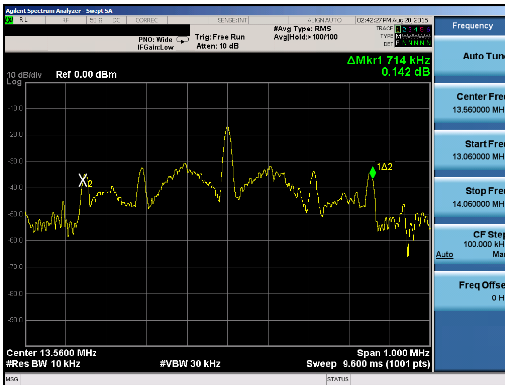
Figure 7-4. 20dB Bandwidth Plot with WCP
