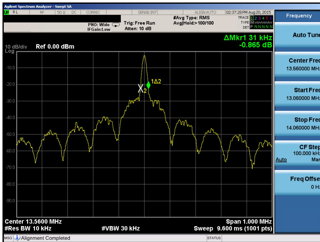
Figure 7-3. 20dB Bandwidth Plot with Wireless Charging Cover
