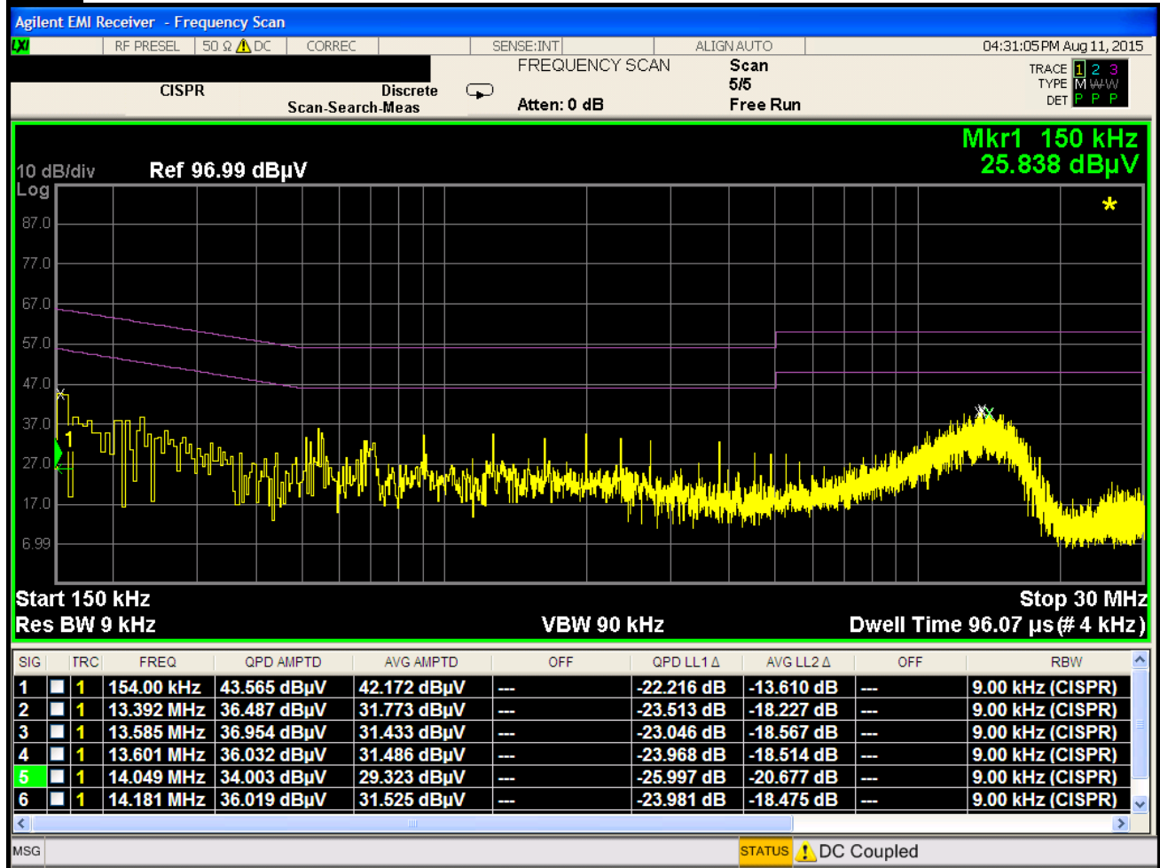
Plot 6-53. Line Conducted Plot with 802.11b (L1)
