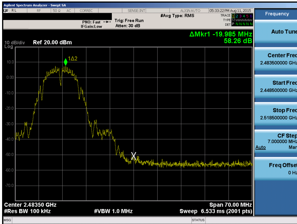
Plot 6-22. Band Edge Plot (802.11b – Ch. 11)
