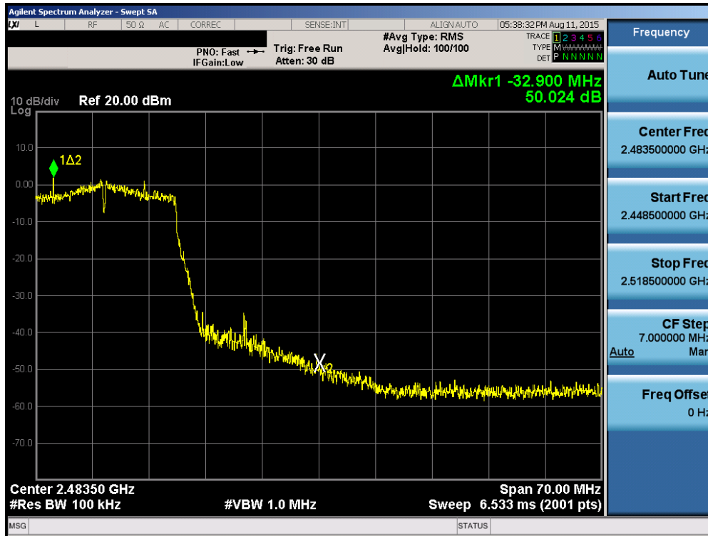
Plot 6-29. Band Edge Plot (802.11n (2.4GHz) – Ch. 10)
