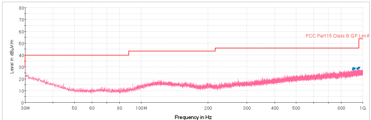
Plot 6-51. Radiated Spurious Plot below 1GHz (Pol. H)
