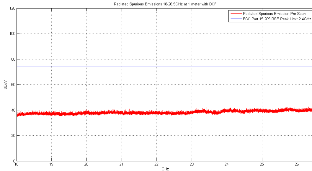
Plot 6-43. Radiated Spurious Plot above 18GHz (Pol. H)
