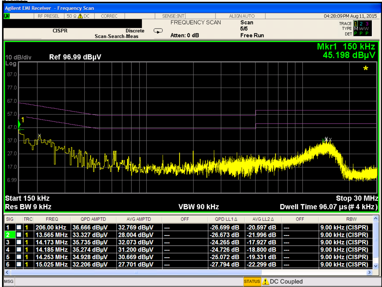
Plot 6-54. Line Conducted Plot with 802.11b (N)
