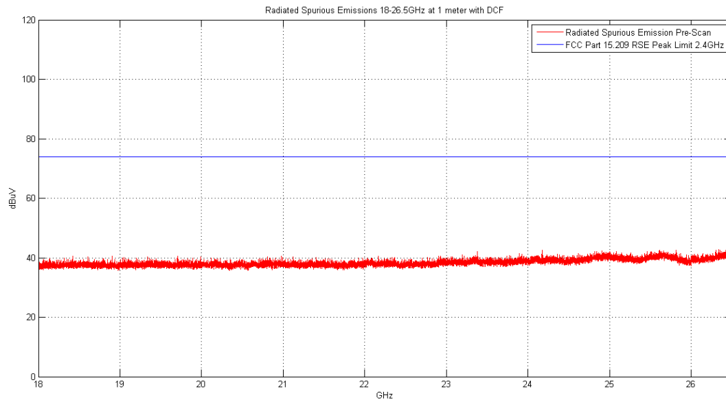
Plot 6-44. Radiated Spurious Plot above 18GHz (Pol. V)
