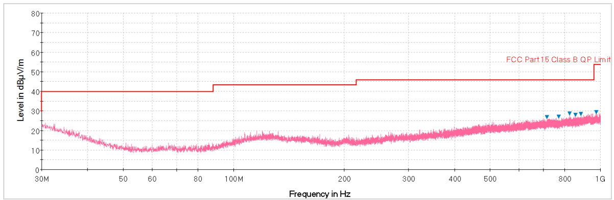
Plot 6-52. Radiated Spurious Plot below 1GHz (Pol. V)
