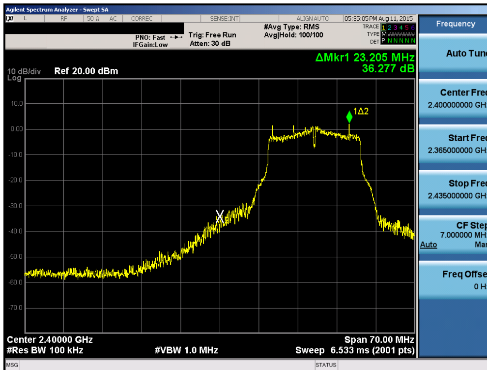
Plot 6-24. Band Edge Plot (802.11g– Ch. 2)
