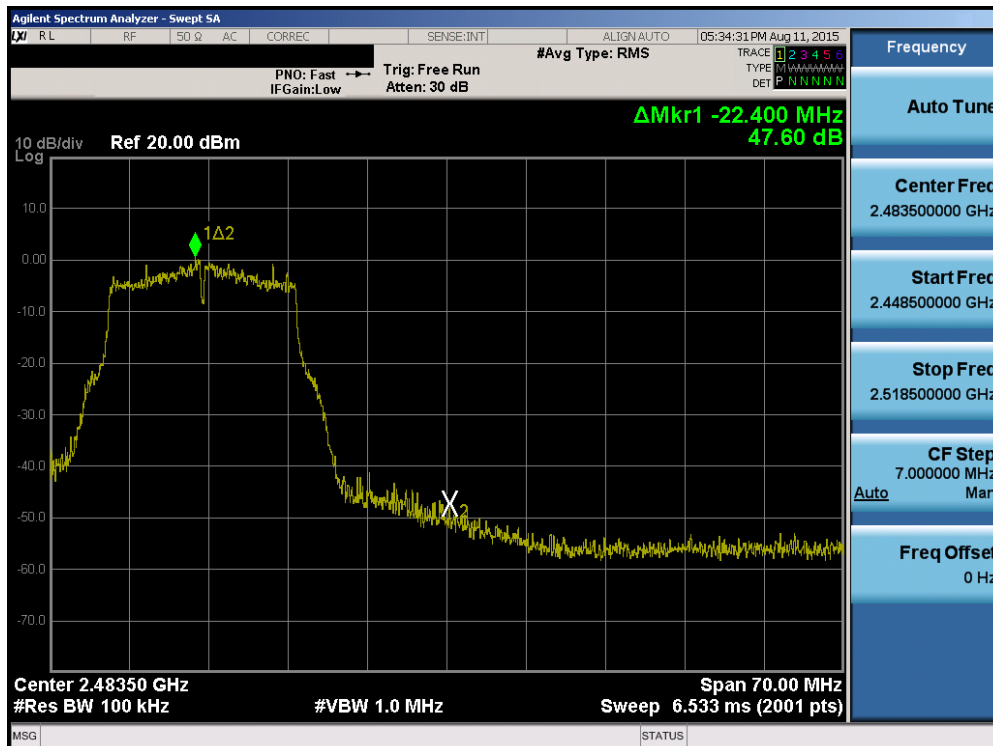
Plot 6-26. Band Edge Plot (802.11g – Ch. 11)
