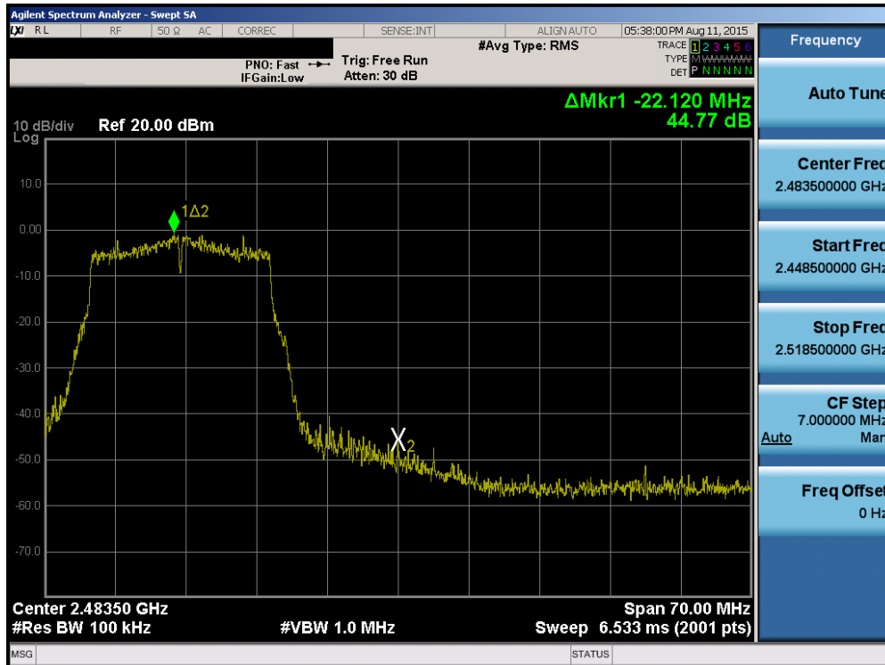
Plot 6-30. Band Edge Plot (802.11n (2.4GHz) – Ch. 11)
