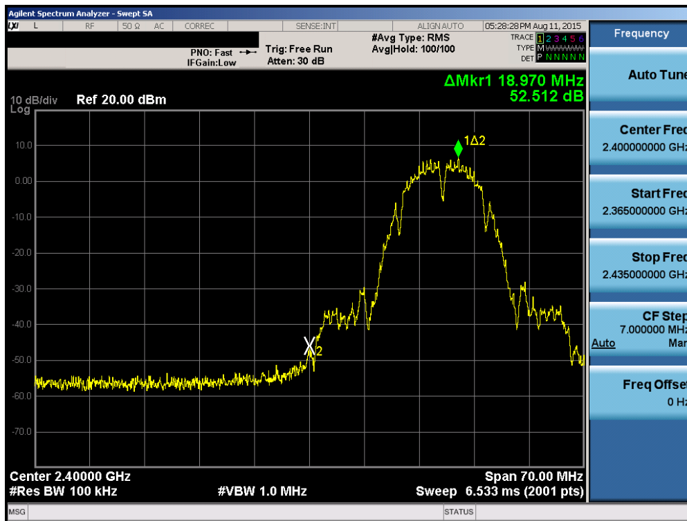
Plot 6-20. Band Edge Plot (802.11b – Ch. 2)
