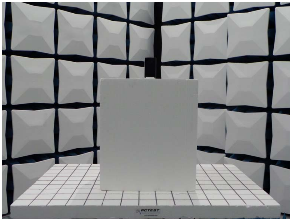
EUT with Wireless Charging Pad
