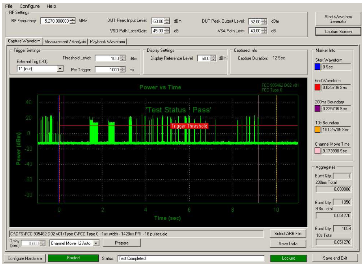
Figure 5-5. Band 2A Move Time and Aggregate Time
