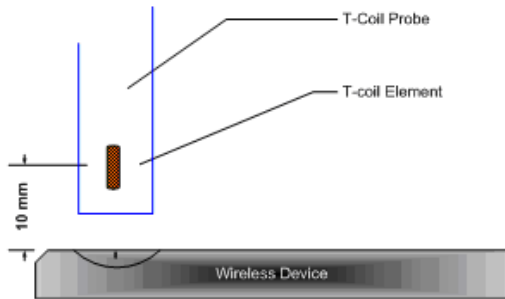
Figure 4-11 Measurement Distance
