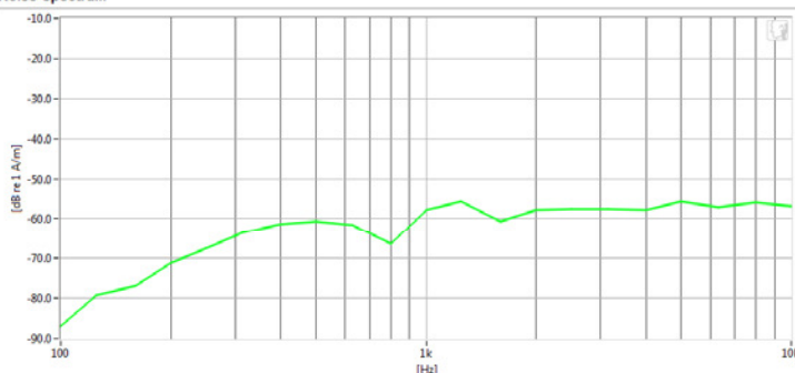
Noise Spectrum
