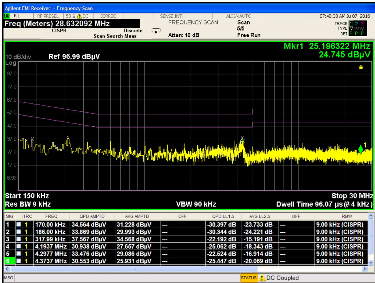
Plot 7-87. Line Conducted Plot with 802.11b (L1)
