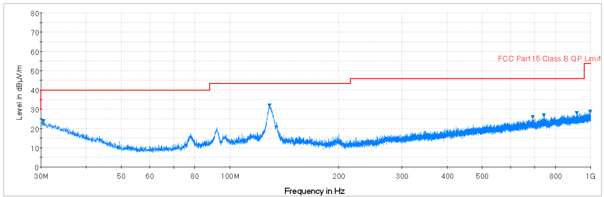
Plot 7-84. Radiated Spurious Plot below 1GHz (Pol. V)
