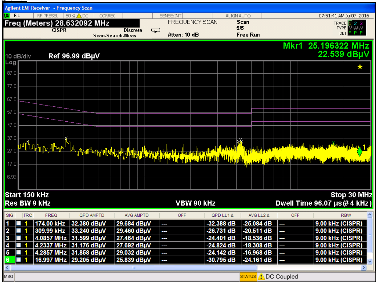
Plot 7-88. Line Conducted Plot with 802.11b (N)
