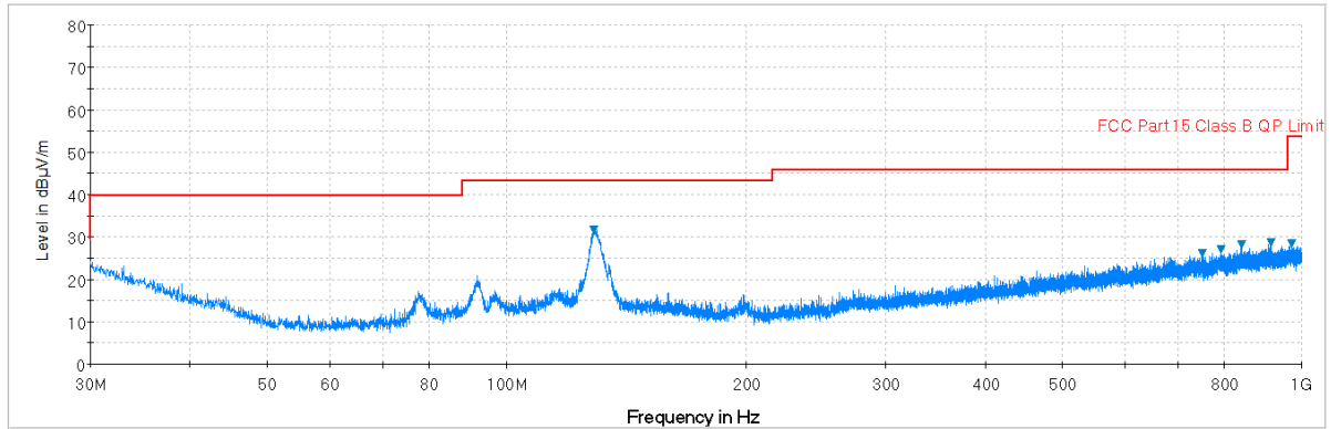
Plot 7-83. Radiated Spurious Plot below 1GHz (Pol. H)
