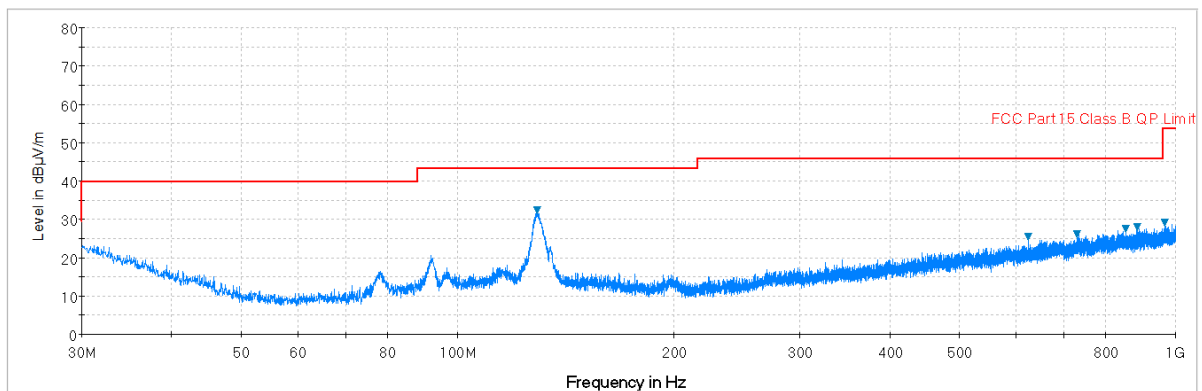
Plot 7-86. Radiated Spurious Plot below 1GHz (Pol. V)
