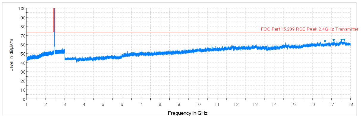
Plot 7-73. Radiated Spurious Plot above 1GHz (802.11b – Ch. 11, Ant. Pol. H)
