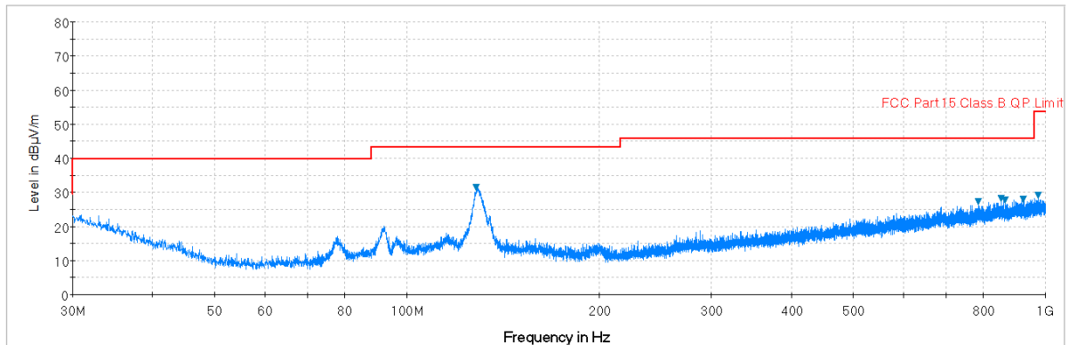
Plot 7-85. Radiated Spurious Plot below 1GHz (Pol. H)
