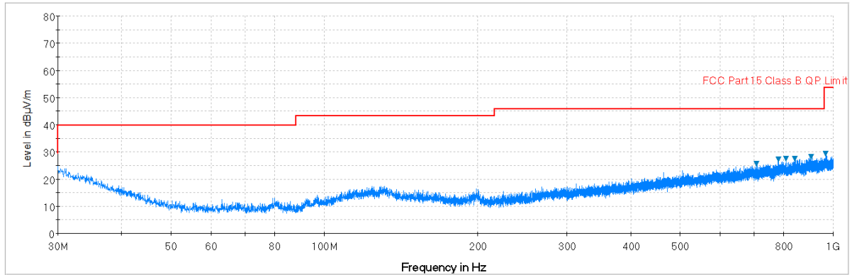
Plot 7-25. Radiated Spurious Plot below 1GHz (Pol. H)
