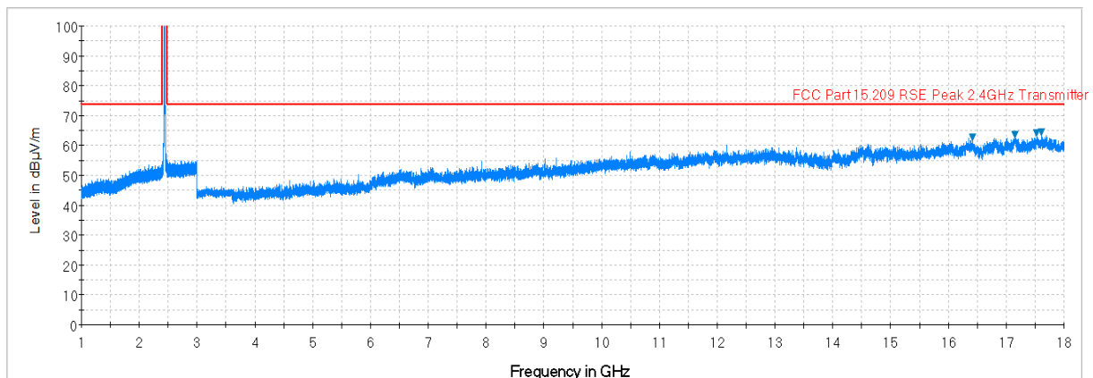
Plot 7-11. Radiated Spurious Plot above 1GHz (802.11b – Ch. 6, Ant. Pol. H)
