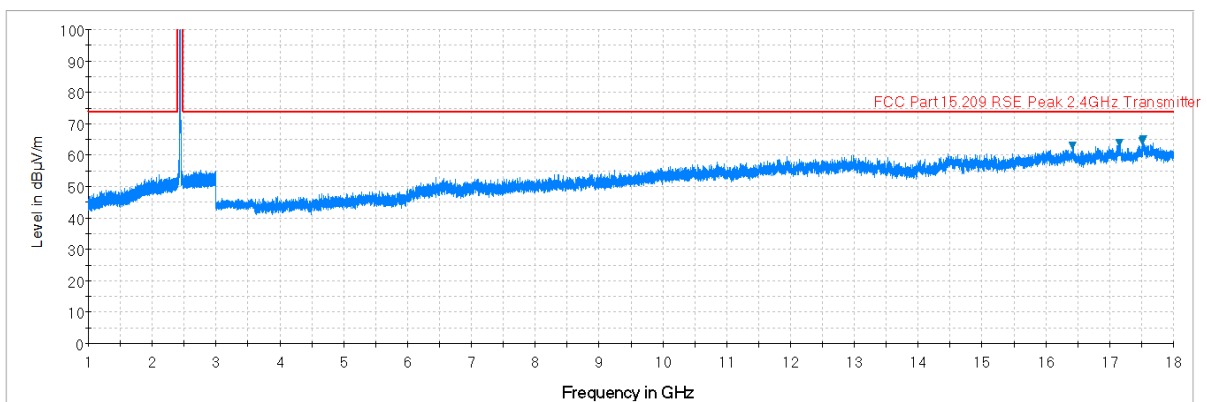
Plot 7-3. Radiated Spurious Plot above 1GHz (802.11b – Ch. 6, Ant. Pol. H)
