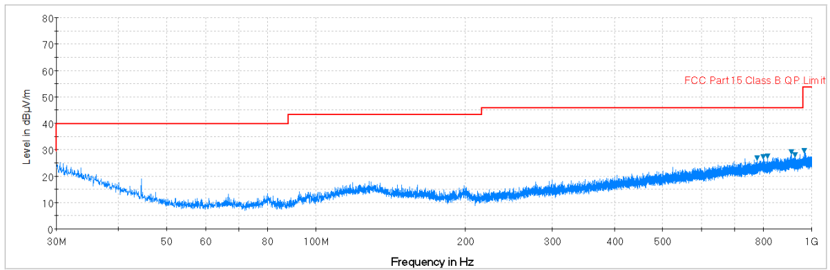
Plot 7-26. Radiated Spurious Plot below 1GHz (Pol. V)
