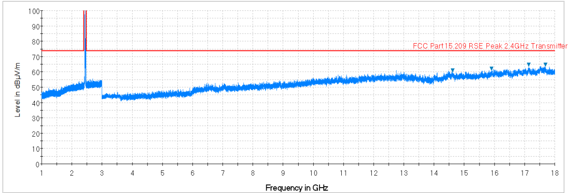
Plot 7-4. Radiated Spurious Plot above 1GHz (802.11b – Ch. 6, Ant. Pol. V)
