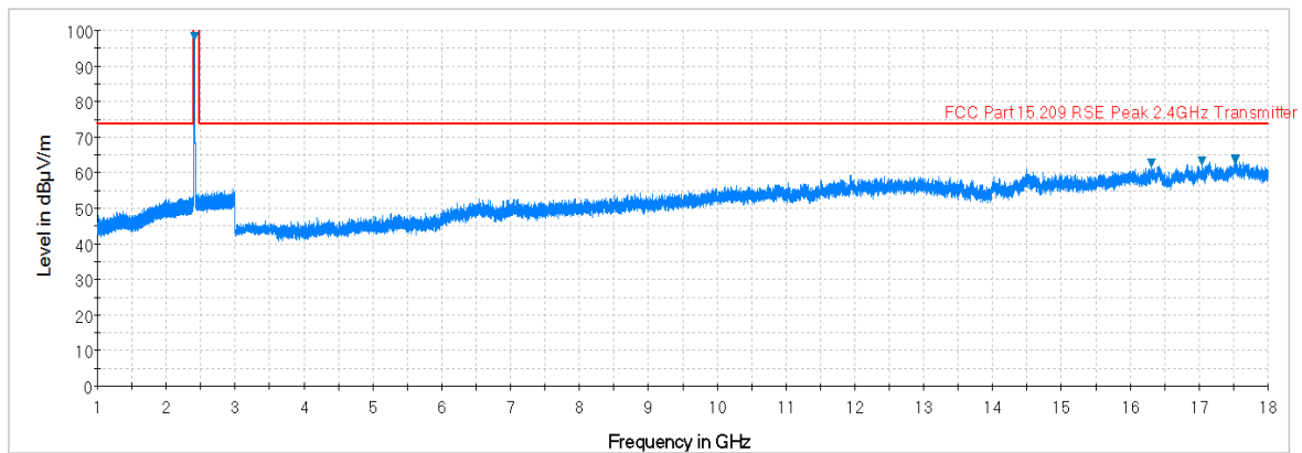
Plot 7-10. Radiated Spurious Plot above 1GHz (802.11b – Ch. 1, Ant. Pol. V)
