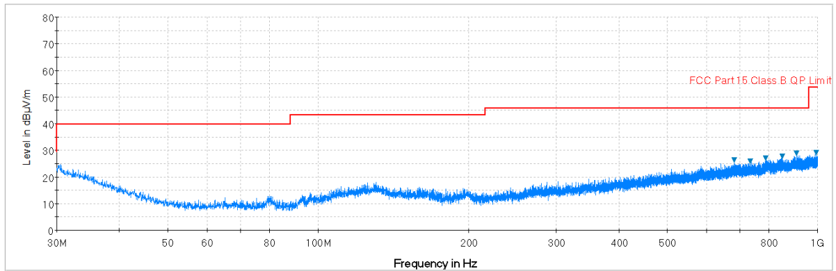
Plot 7-23. Radiated Spurious Plot below 1GHz (Pol. H)
