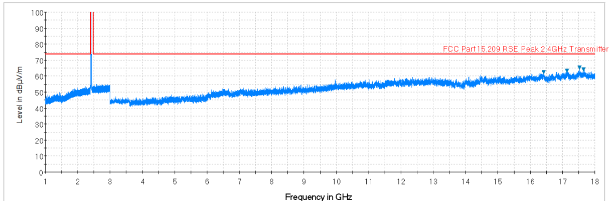
Plot 7-9. Radiated Spurious Plot above 1GHz (802.11b – Ch. 1, Ant. Pol. H)
