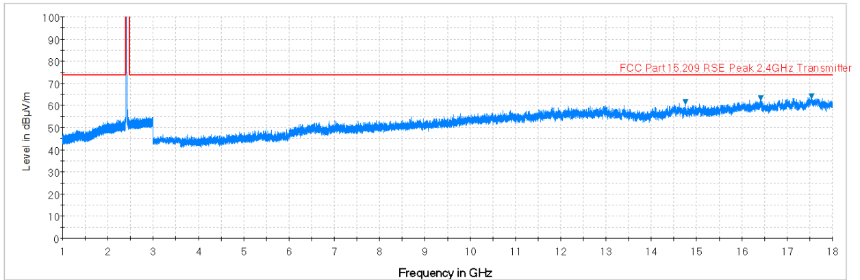
Plot 7-1. Radiated Spurious Plot above 1GHz (802.11b – Ch. 1, Ant. Pol. H)
