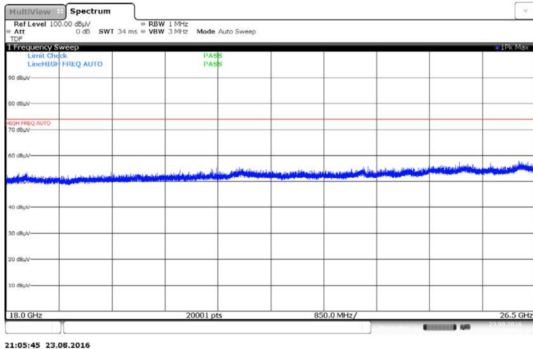
Plot 7-15. Radiated Spurious Plot above 18GHz (Pol. H)
