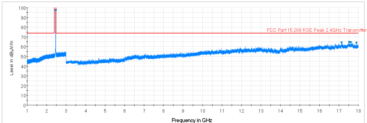
Plot 7-6. Radiated Spurious Plot above 1GHz (802.11b – Ch. 11, Ant. Pol. V)
