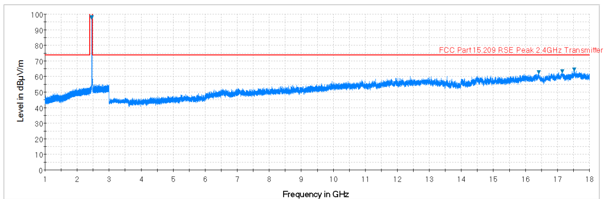
Plot 7-14. Radiated Spurious Plot above 1GHz (802.11b – Ch. 11, Ant. Pol. V)
