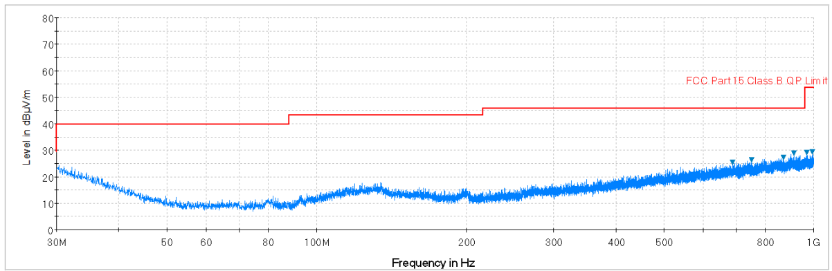
Plot 7-24. Radiated Spurious Plot below 1GHz (Pol. V)
