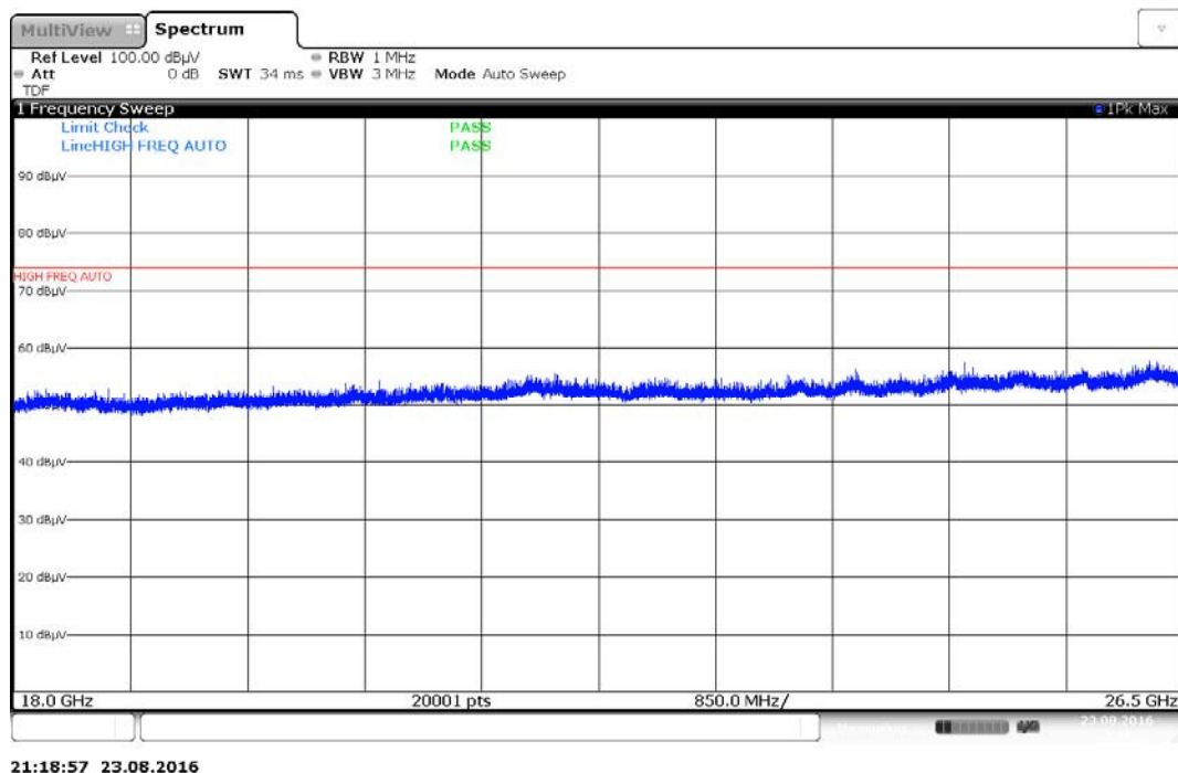
Plot 7-16. Radiated Spurious Plot above 18GHz (Pol. V)
