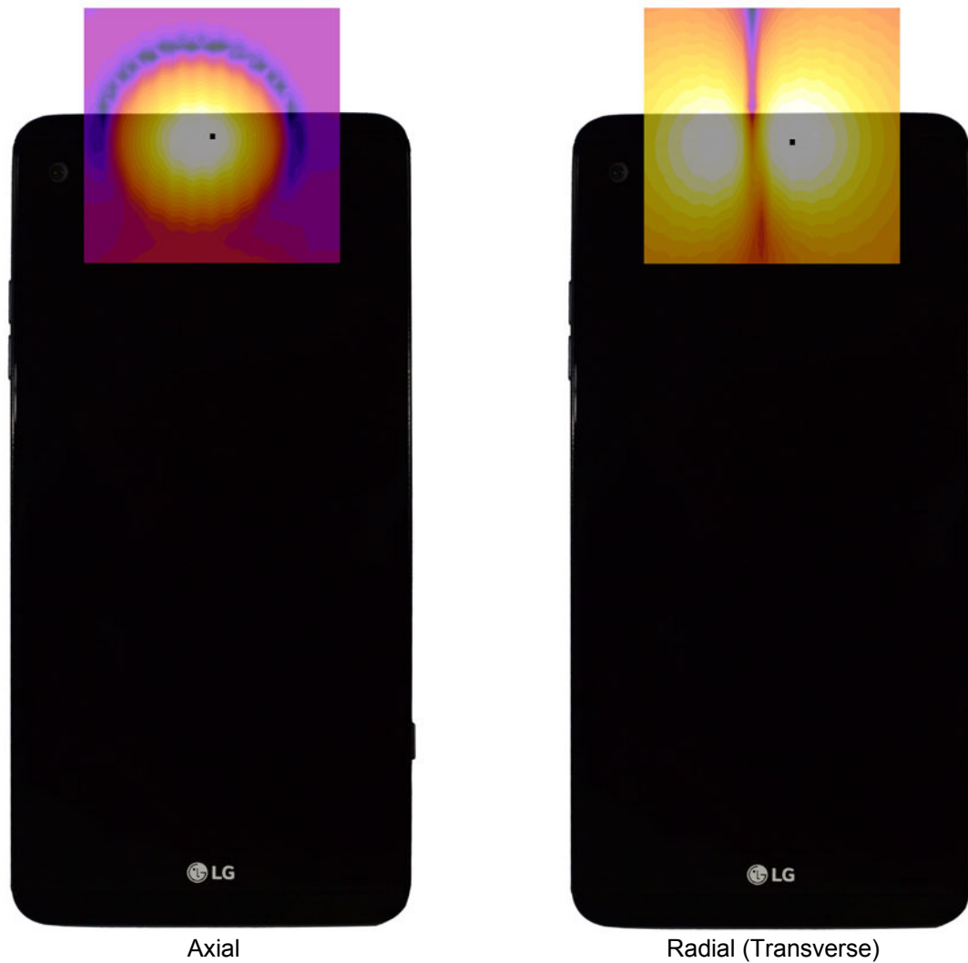
Axial Radial (Transverse) Figure 14-3 T-Coil Scan Overlay Magnetic Field Distributions
