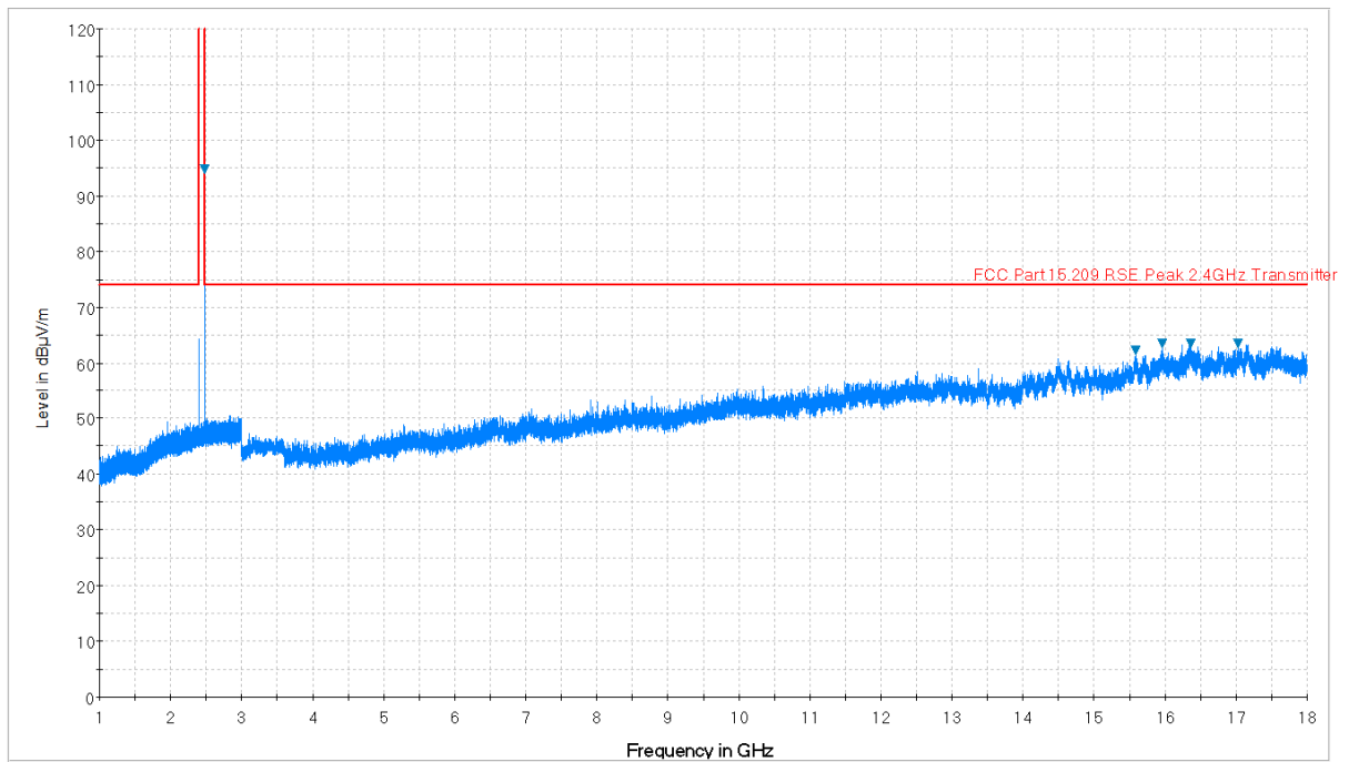
Plot 7-47. Radiated Spurious Plot above 1GHz (BT – Ch. 78, Ant. Pol. V)
