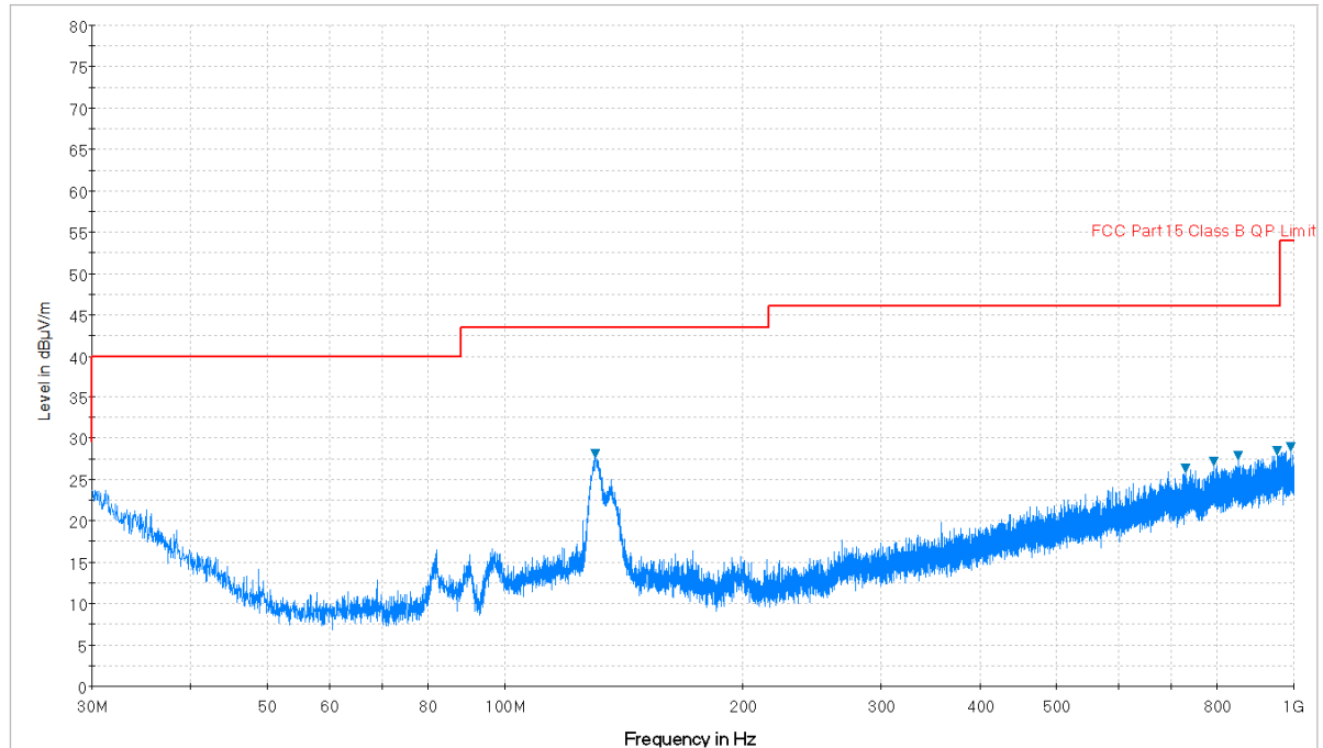
Plot 7-54. Radiated Spurious Plot below 1GHz (Pol. H)
