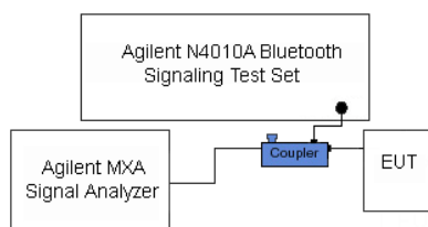
Figure 7-3. Test Instrument & Measurement Setup
