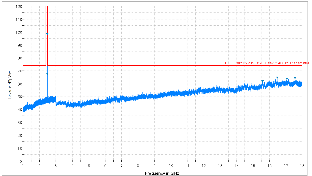
Plot 7-46. Radiated Spurious Plot above 1GHz (BT – Ch. 78, Ant. Pol. H)
