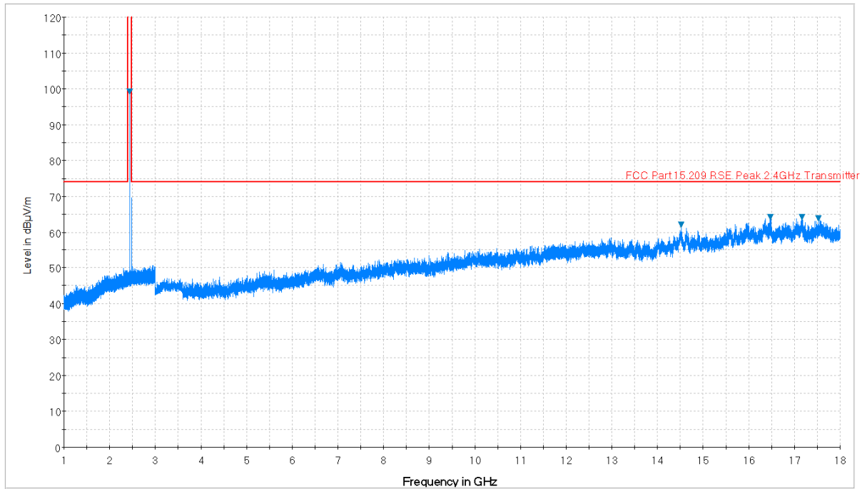
Plot 7-44. Radiated Spurious Plot above 1GHz (BT – Ch. 39, Ant. Pol. H)
