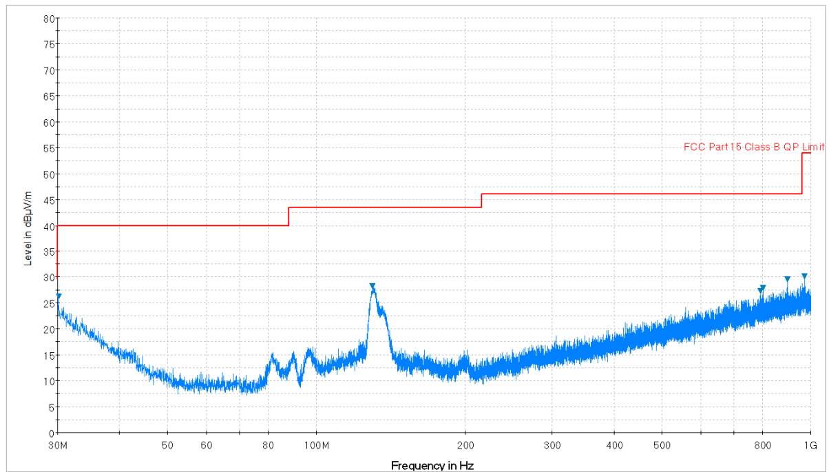
Plot 7-55. Radiated Spurious Plot below 1GHz (Pol. V)
