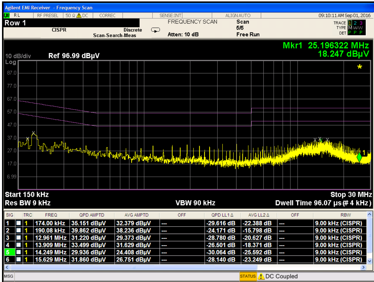
Plot 7-57. Line-Conducted Test Plot (N)
