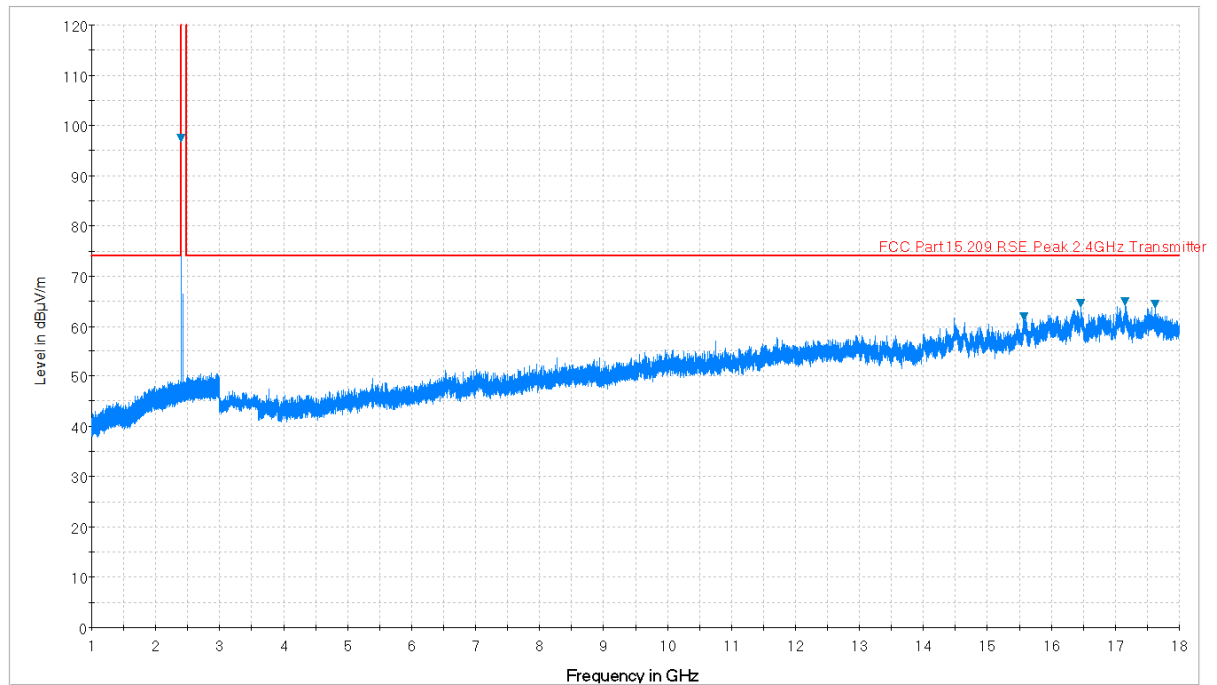
Plot 7-42. Radiated Spurious Plot above 1GHz (BT – Ch. 0, Ant. Pol. H)
