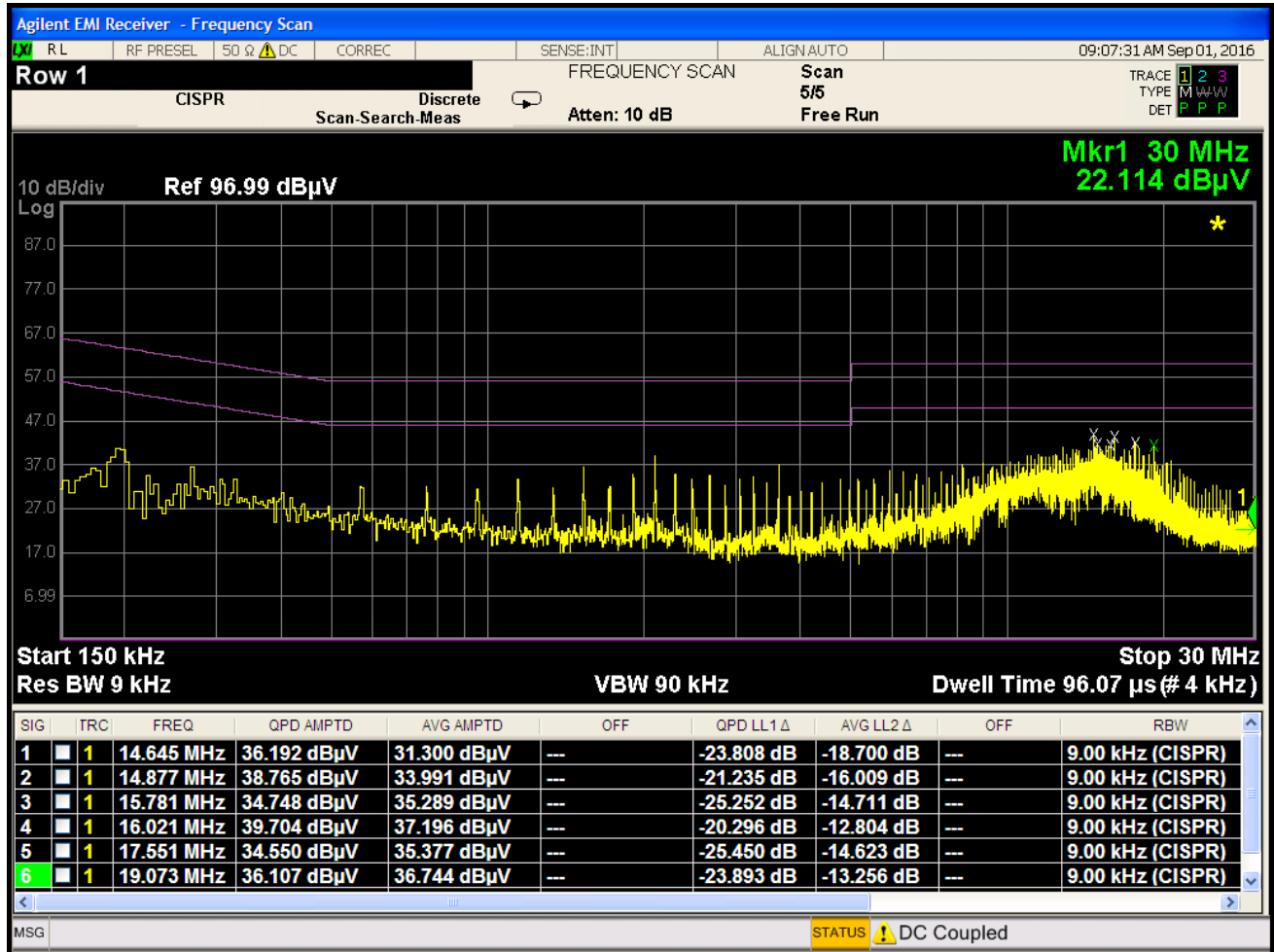
Plot 7-56. Line-Conducted Test Plot (L1)
