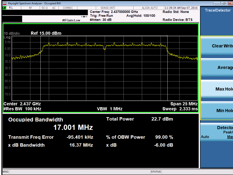
Plot 7-6. 6dB Bandwidth Plot (802.11g – Ch. 6)
