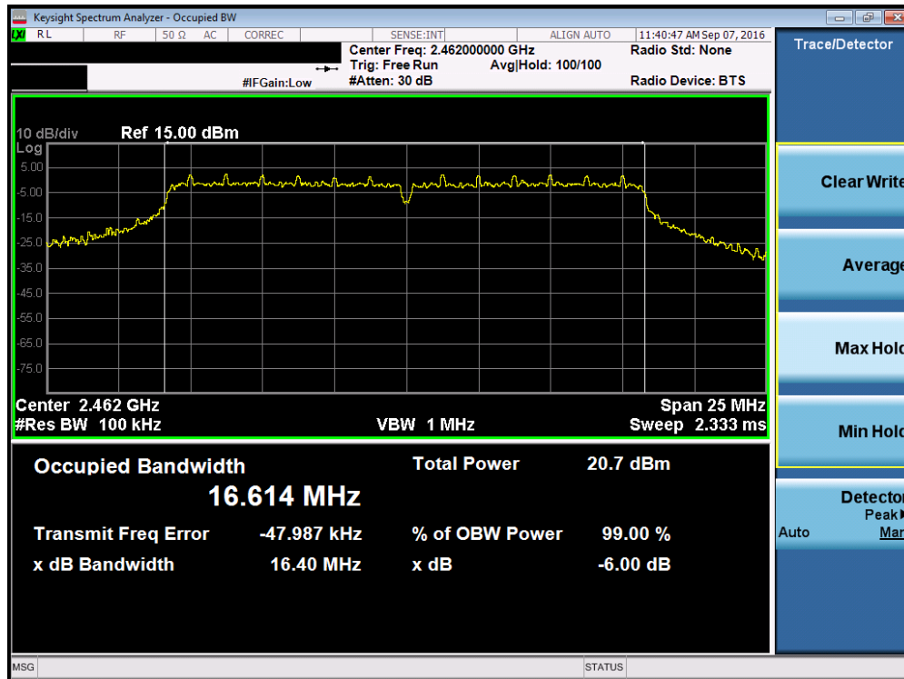
Plot 7-7. 6dB Bandwidth Plot (802.11g – Ch. 11)
