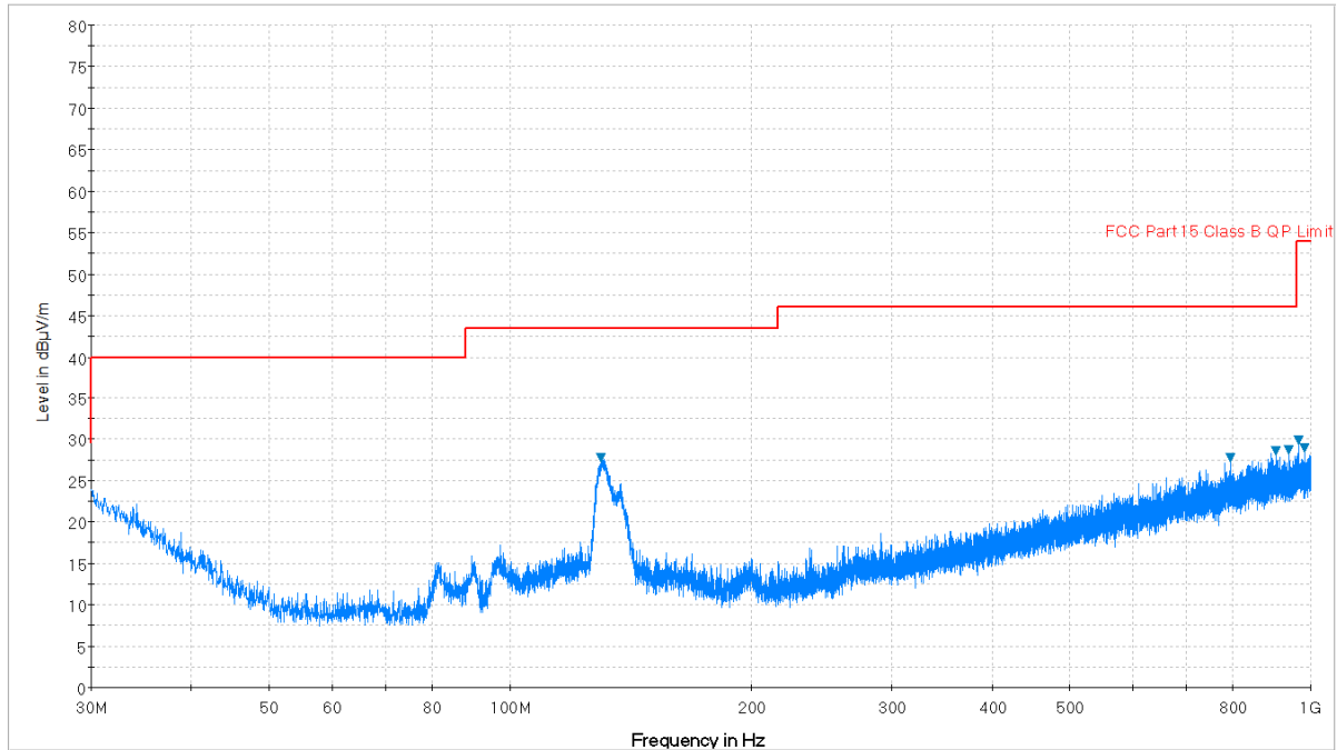
Plot 7-58. Radiated Spurious Plot below 1GHz (Pol. H)
