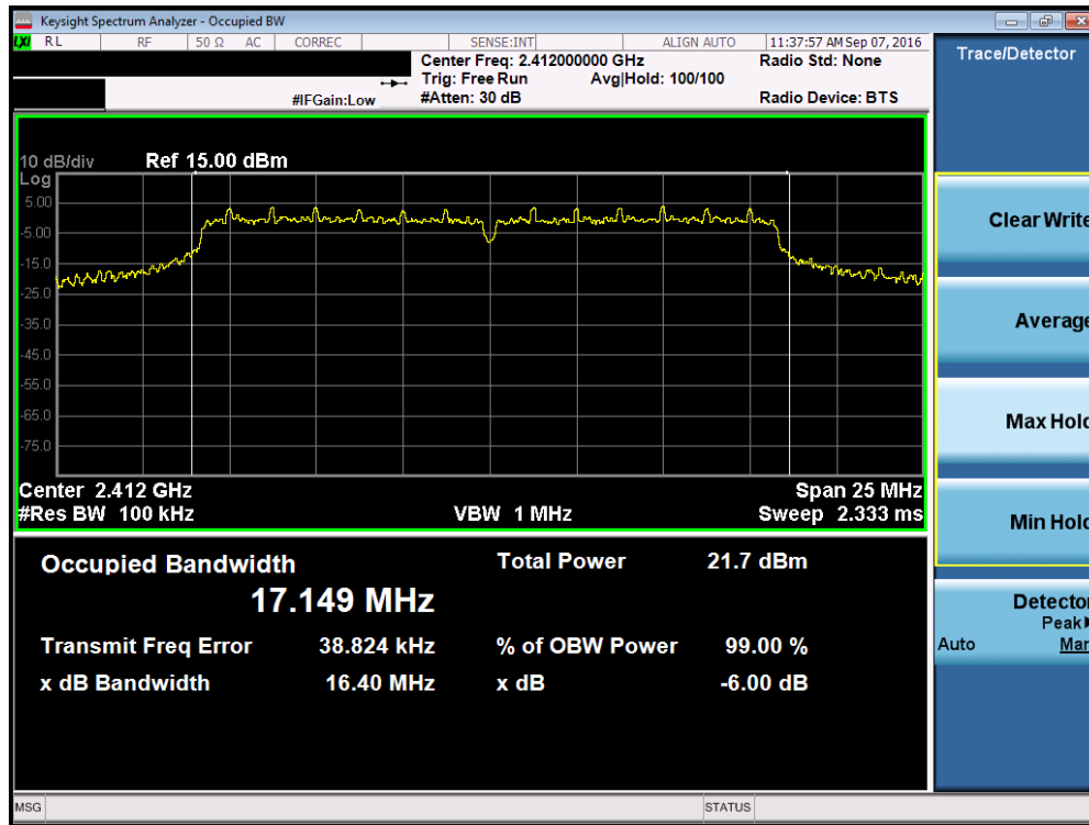
Plot 7-5. 6dB Bandwidth Plot (802.11g – Ch. 1)
