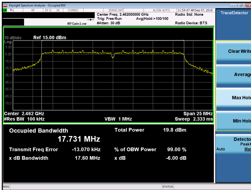
Plot 7-11. 6dB Bandwidth Plot (802.11n (2.4GHz) – Ch. 11)
