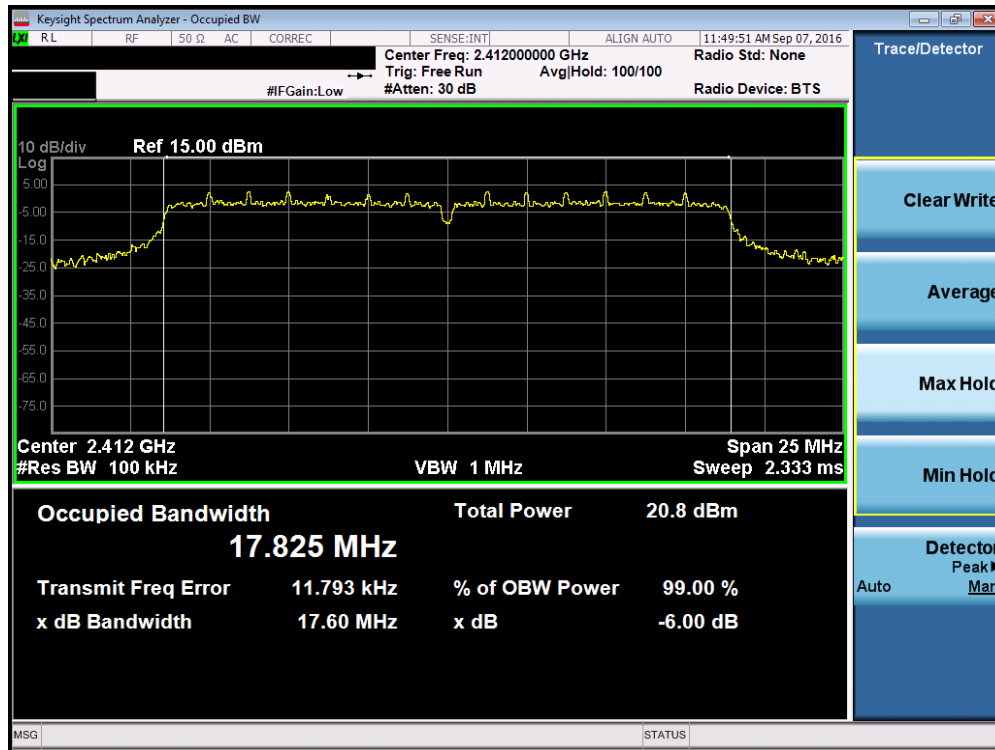
Plot 7-9. 6dB Bandwidth Plot (802.11n (2.4GHz) – Ch. 1)
