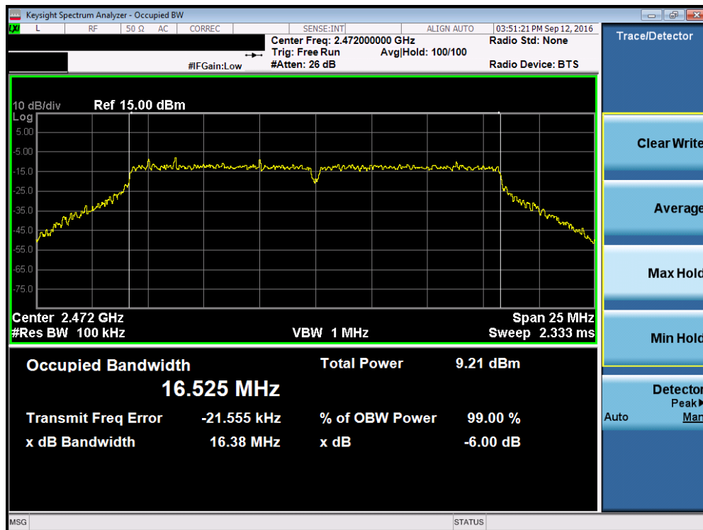
Plot 7-8. 6dB Bandwidth Plot (802.11g – Ch. 13)
