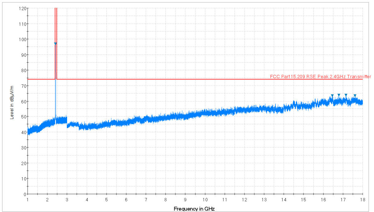
Plot 7-40. Radiated Spurious Plot above 1GHz (802.11b – Ch. 1, Ant. Pol. H)
