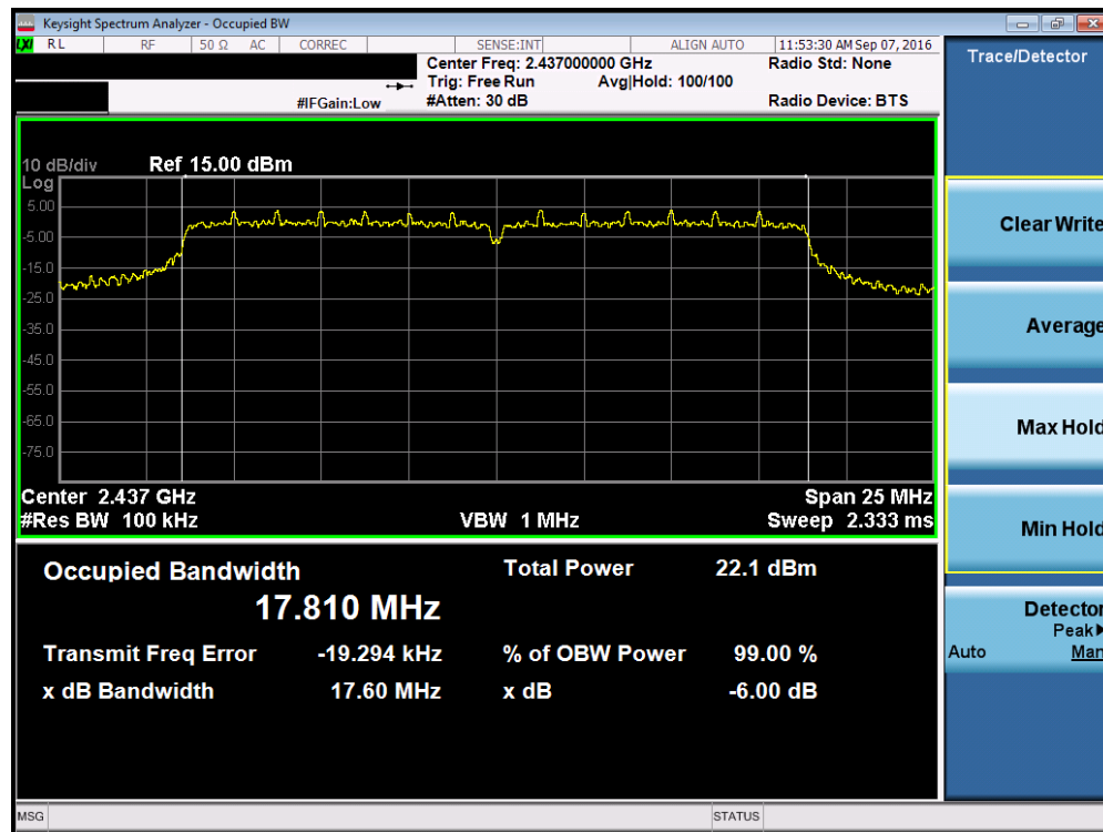
Plot 7-10. 6dB Bandwidth Plot (802.11n (2.4GHz) – Ch. 6)
