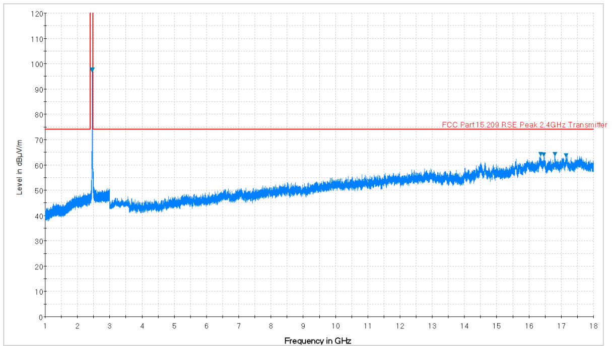
Plot 7-44. Radiated Spurious Plot above 1GHz (802.11b – Ch. 11, Ant. Pol. H)
