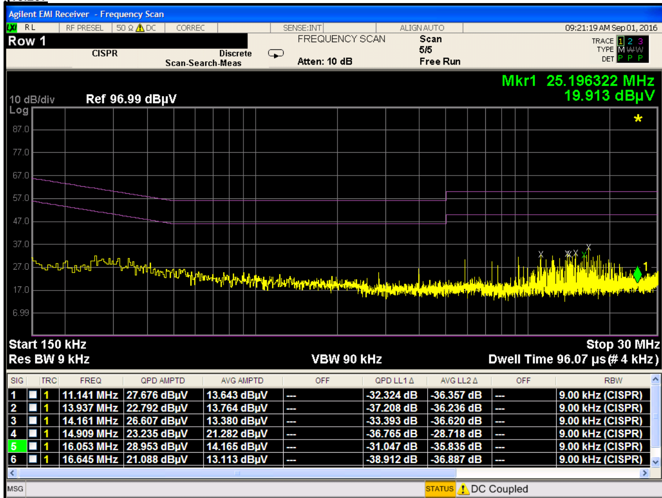
Plot 7-61. Line Conducted Plot with 802.11b (N)
