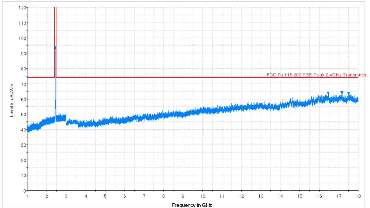
Plot 7-43. Radiated Spurious Plot above 1GHz (802.11b – Ch. 6, Ant. Pol. V)
