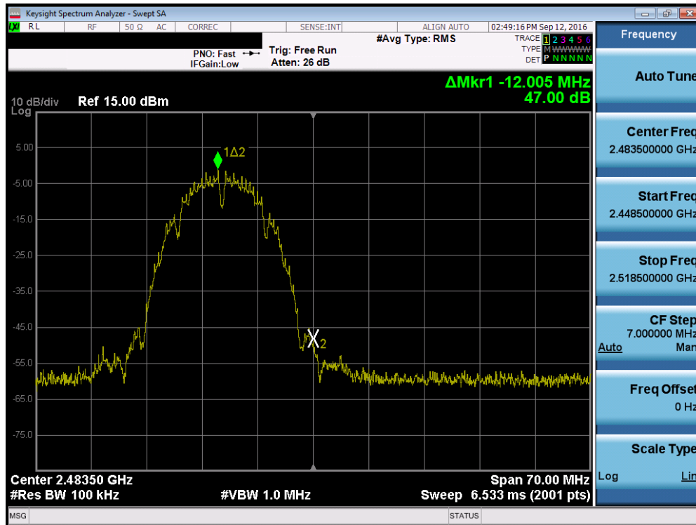
Plot 7-25. Band Edge Plot (802.11b – Ch. 13)
