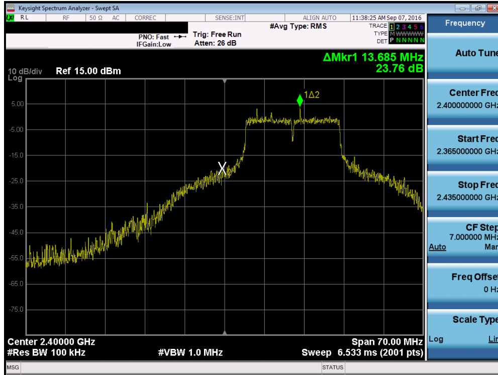
Plot 7-26. Band Edge Plot (802.11g- Ch. 1)
