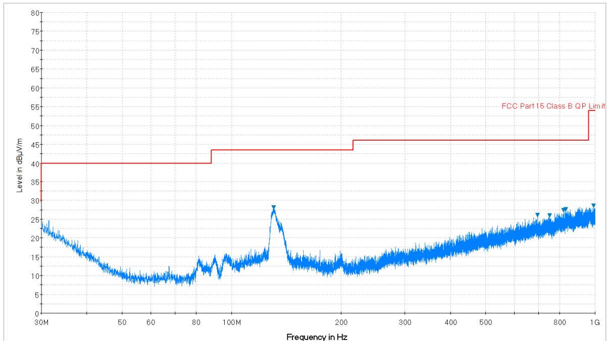
Plot 7-59. Radiated Spurious Plot below 1GHz (Pol. V)
