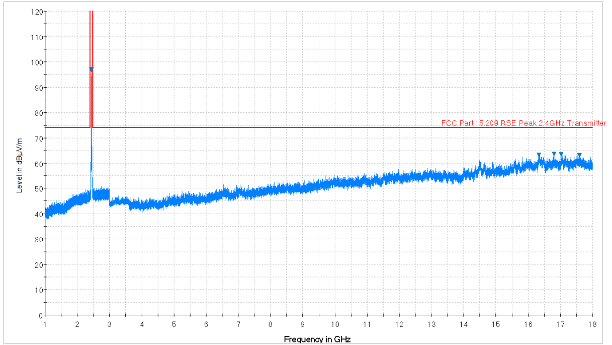
Plot 7-42. Radiated Spurious Plot above 1GHz (802.11b – Ch. 6, Ant. Pol. H)
