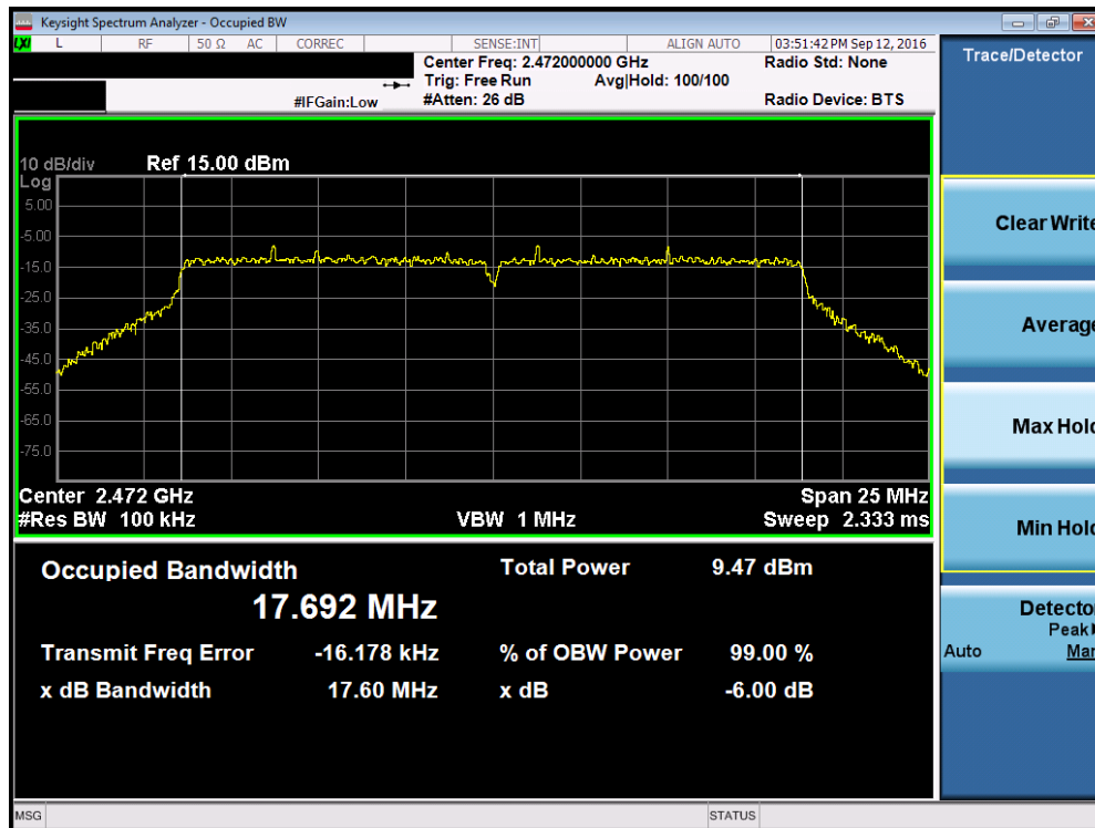
Plot 7-12. 6dB Bandwidth Plot (802.11n – Ch. 13)
