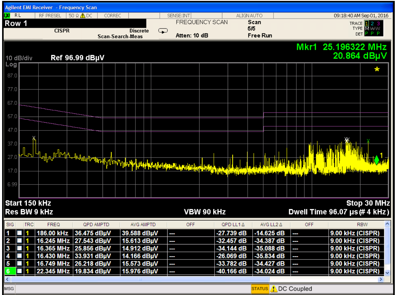
Plot 7-60. Line Conducted Plot with 802.11b (L1)
