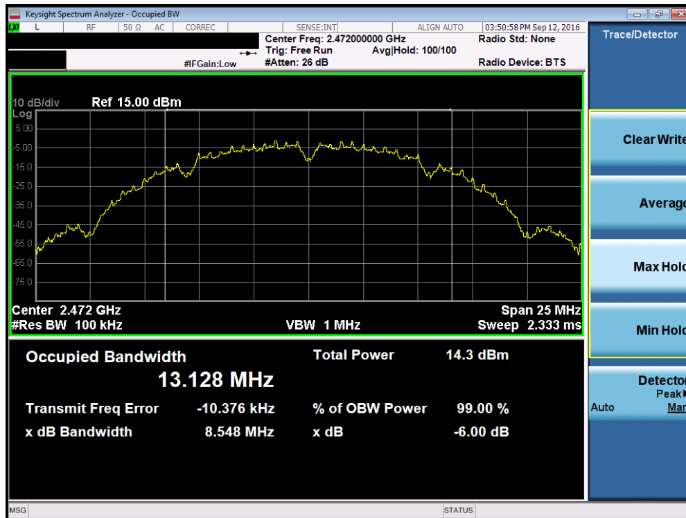
Plot 7-4. 6dB Bandwidth Plot (802.11b – Ch. 13)
