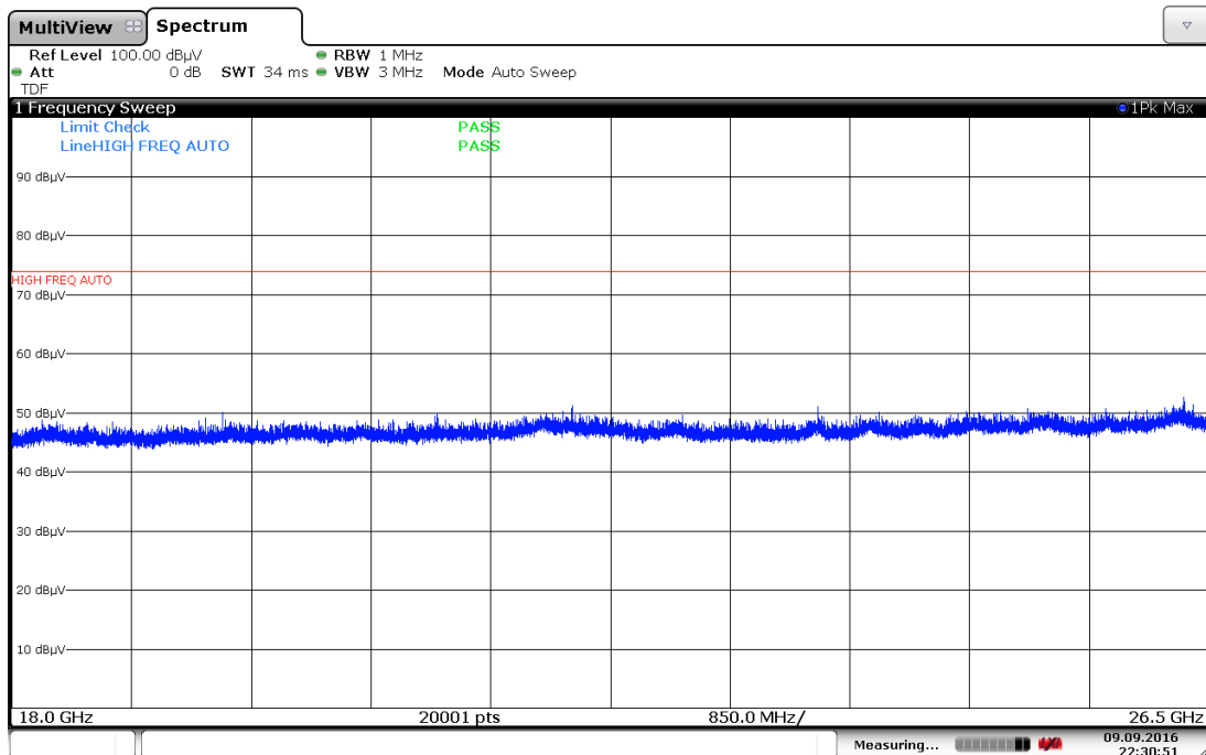
Plot 7-47. Radiated Spurious Plot above 18GHz (Pol. V)
