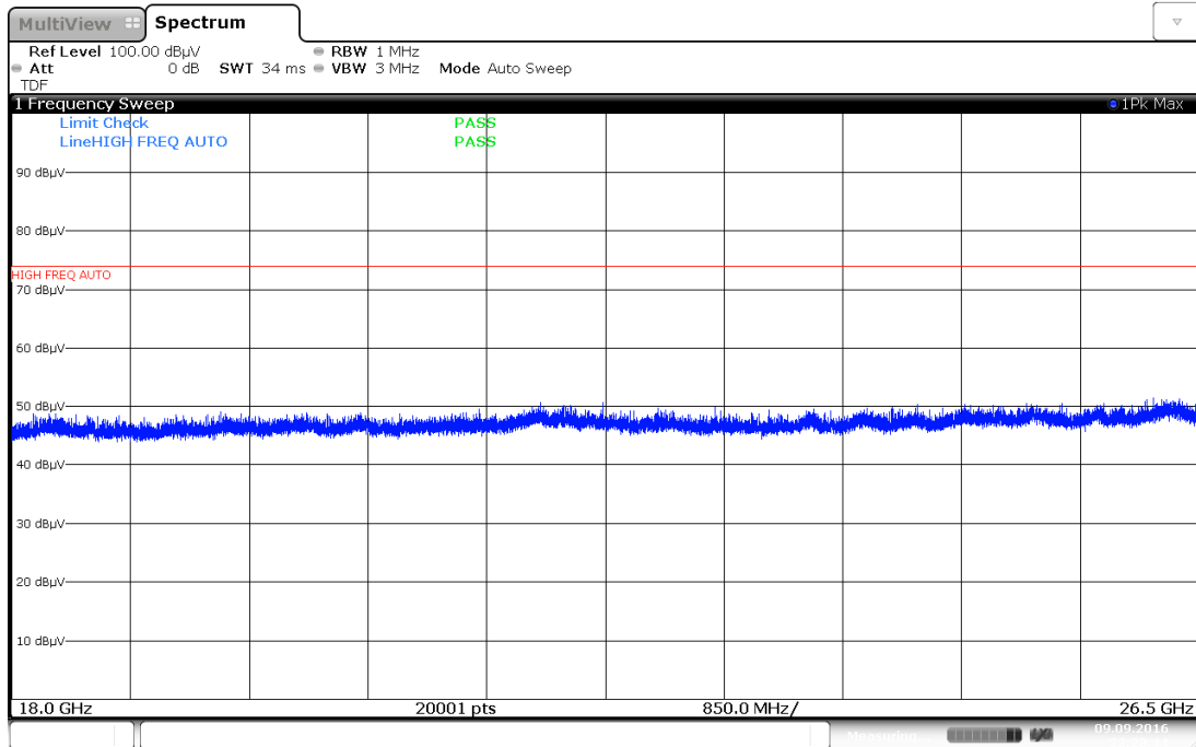
Plot 7-46. Radiated Spurious Plot above 18GHz (Pol. H)
