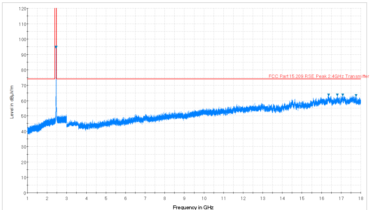
Plot 7-45. Radiated Spurious Plot above 1GHz (802.11b – Ch. 11, Ant. Pol. V)
