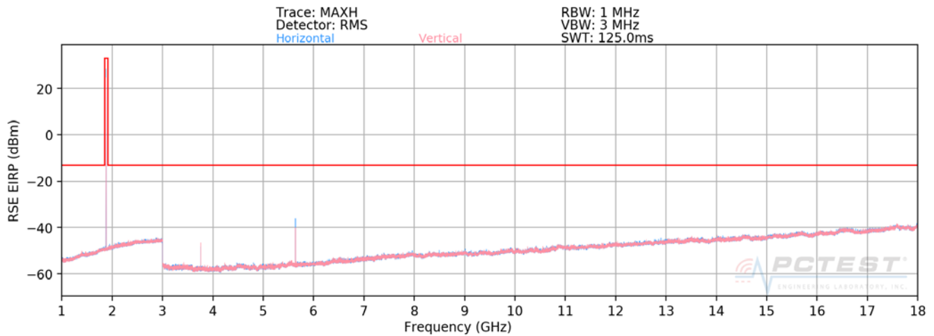
Plot 7-79. Radiated Spurious Plot above 1GHz (PCS GPRS Mode)
