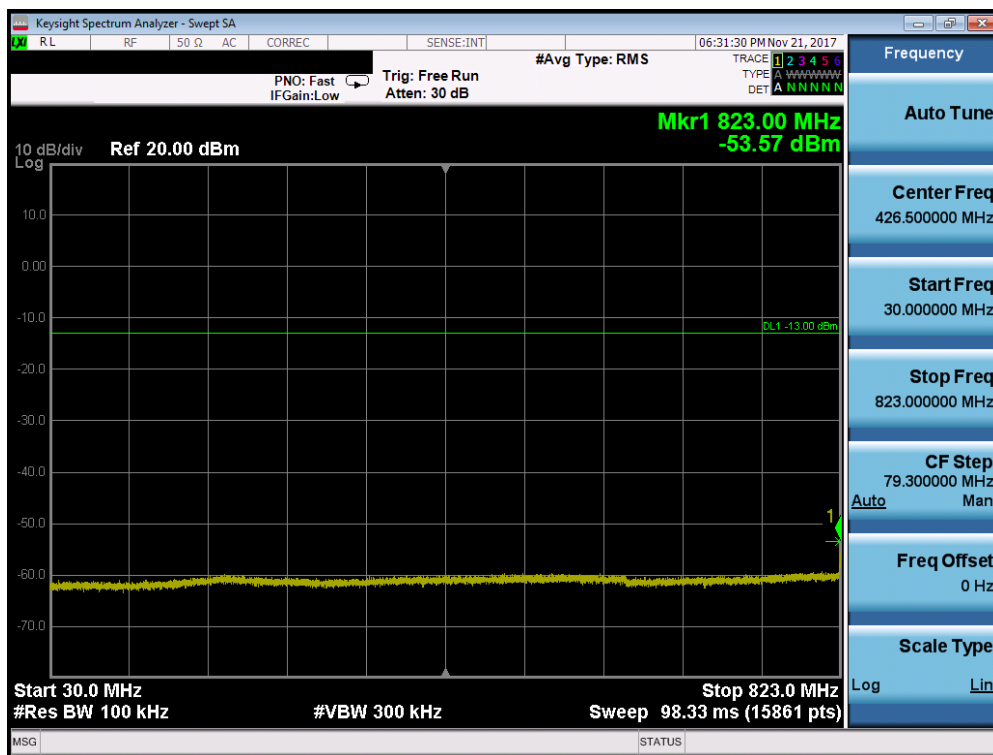
Plot 7-50. Conducted Spurious Plot (Band 5 - 5.0MHz QPSK - RB Size 1, RB Offset 0 - Low Channel)
