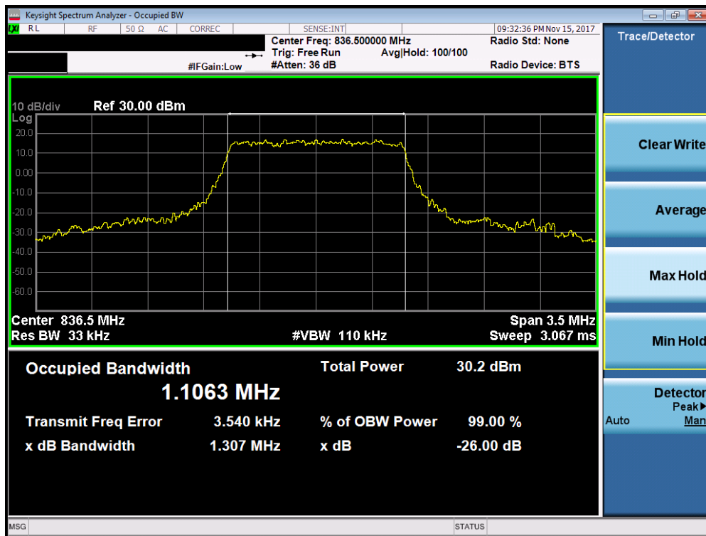
Plot 7-10. Occupied Bandwidth Plot (Band 5 - 1.4MHz QPSK - Full RB Configuration)
