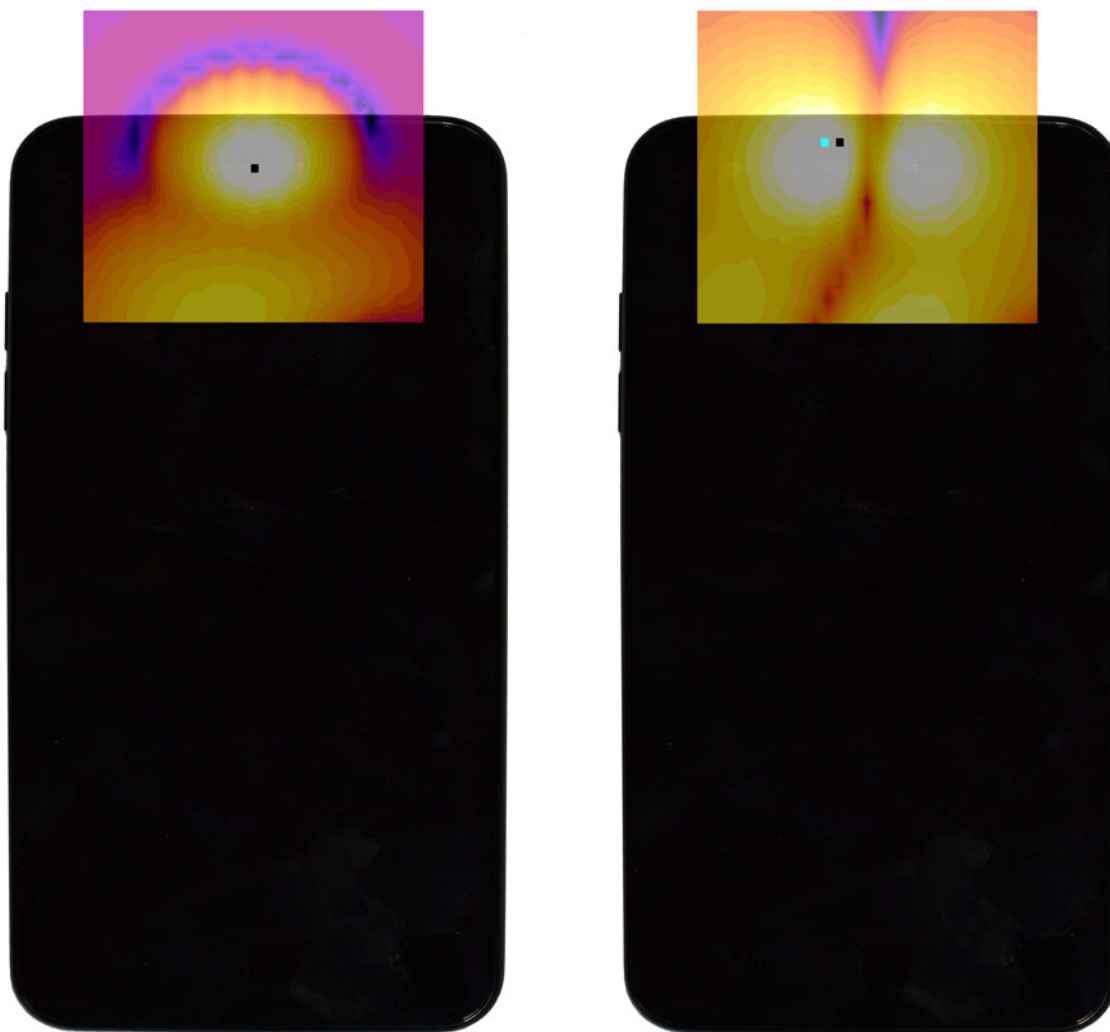
Figure 16-3 T-Coil Scan Overlay Magnetic Field Distributions
