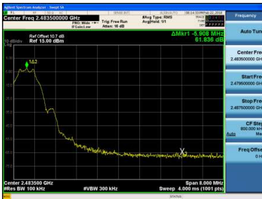
BandEdge (High-CH 39)
