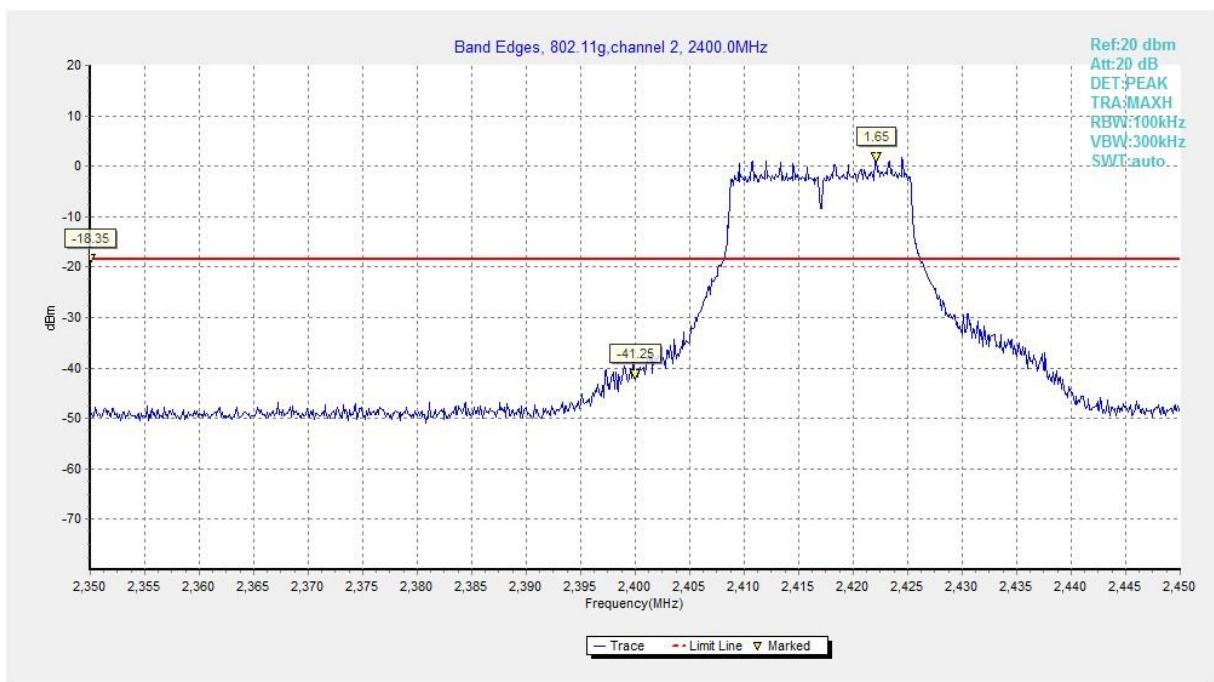
Fig.A.5.4 Band Edges (802.11g, Ch 2)
