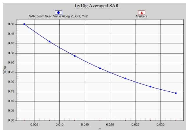
Fig.A.1- 18 Z-Scan at power reference point (LTE band17)
