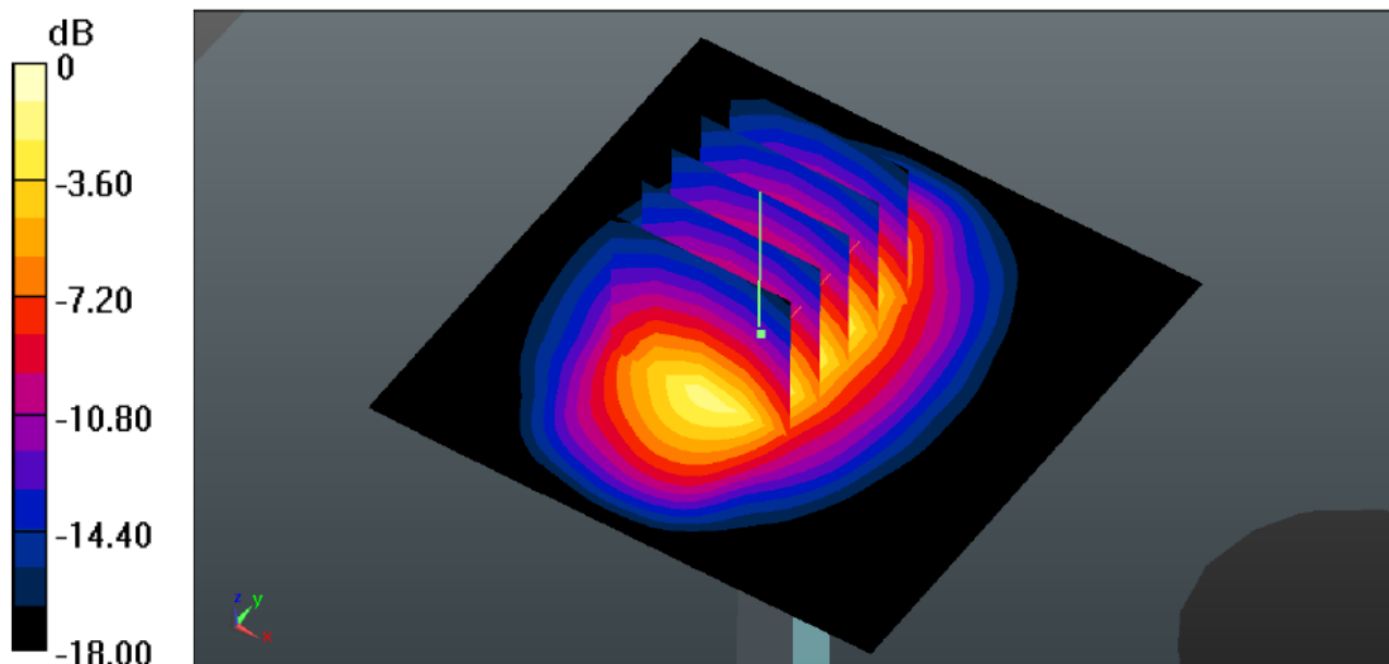
System Performance Check 1900MHz Head 250mW
