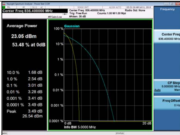
Channel 4183 / 836.4 MHz
