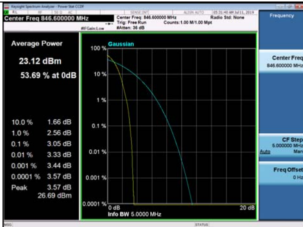
Channel 4233 / 846.6 MHz
