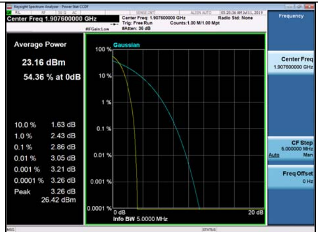
Channel 9538 / 1907.6 MHz
