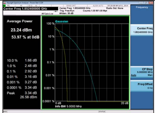
Channel 9262 / 1852.4 MHz
