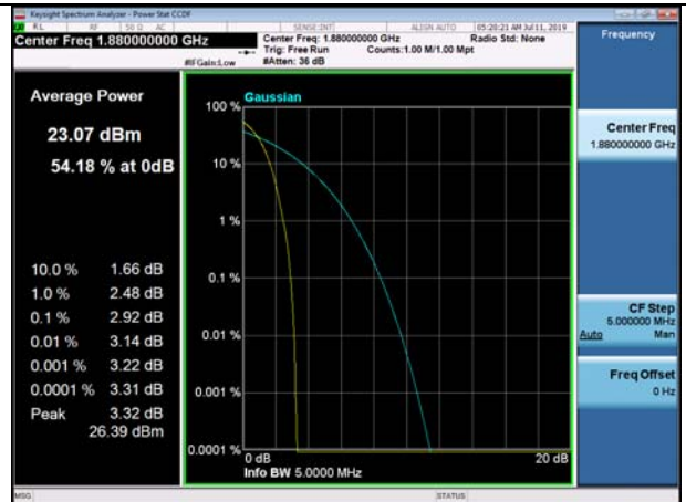
Channel 9400 / 1880.0 MHz
