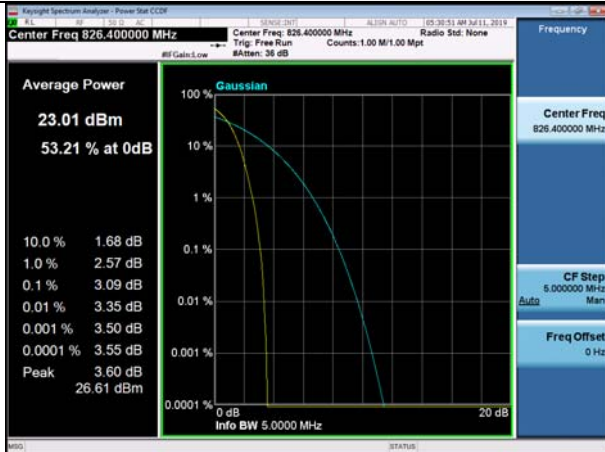
Channel 4132 / 826.4 MHz
