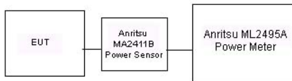
Figure 9-4 Power Measurement Setup
