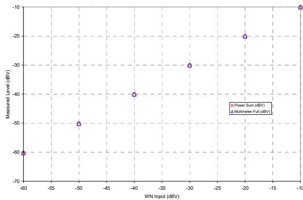
Figure 4-10 ABM2 Power Sum Validation
