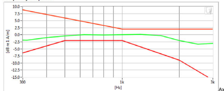
Frequency Response
