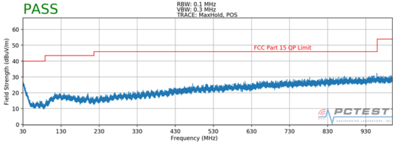
Plot 7-31. Radiated Spurious Plot below 1GHz (802.11a – U3 Ch. 157, Ant. Pol. H)
