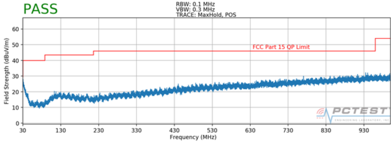
Plot 7-32. Radiated Spurious Plot below 1GHz (802.11a – U3 Ch. 157, Ant. Pol. V)
