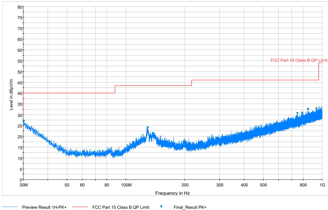
Plot 7-41. Radiated Spurious Plot below 1GHz (Pol. H)
