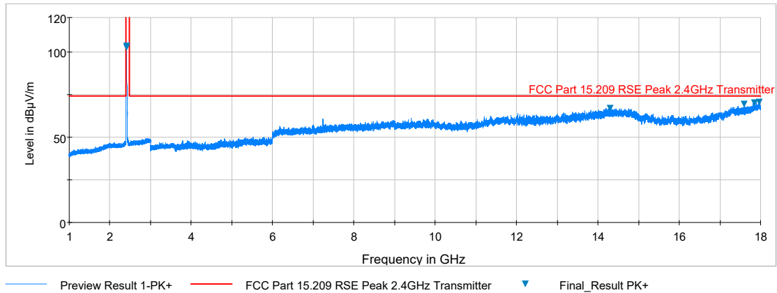
Plot 7-31. Radiated Spurious Plot above 1GHz (802.11b – Ch. 1, Ant. Pol. H)
