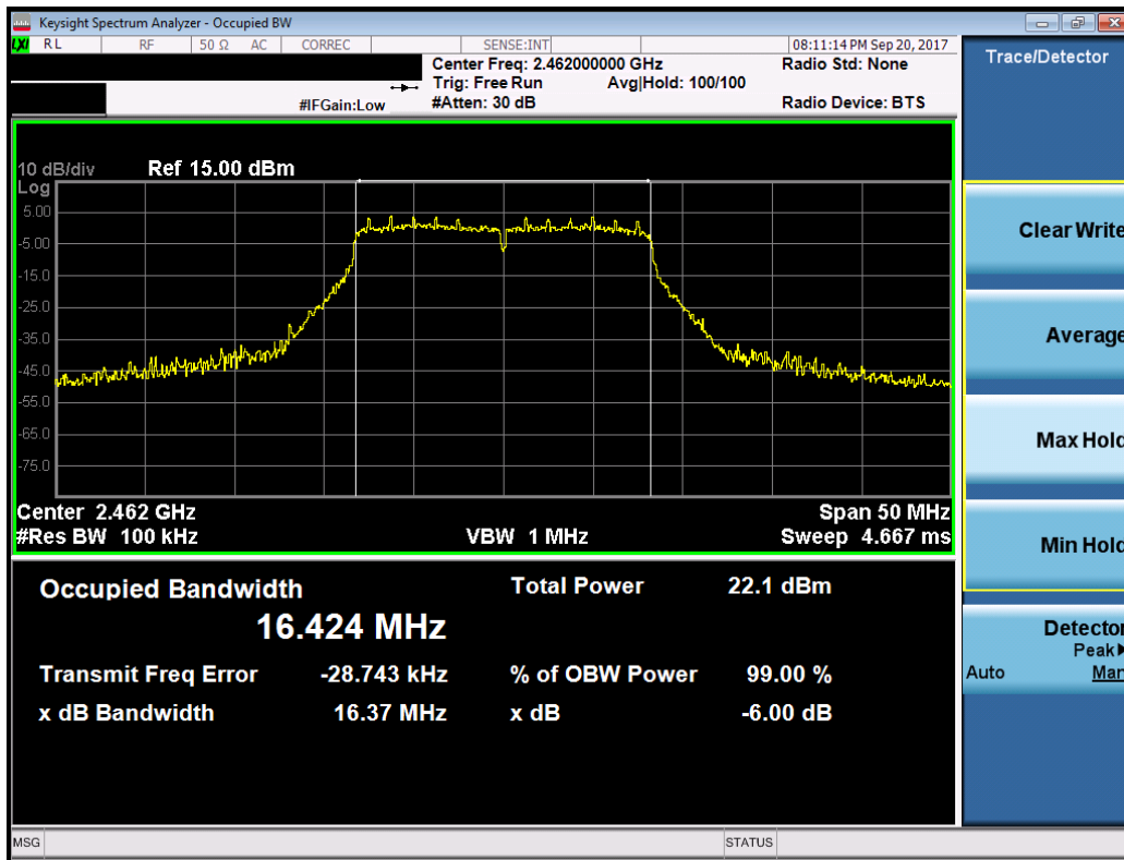
Plot 7-6. 6dB Bandwidth Plot (802.11g – Ch. 11)
