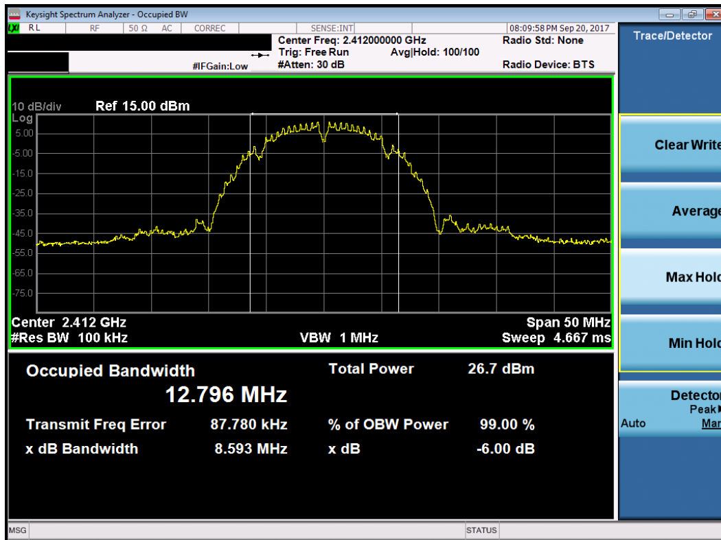
Plot 7-1. 6dB Bandwidth Plot (802.11b – Ch. 1)
