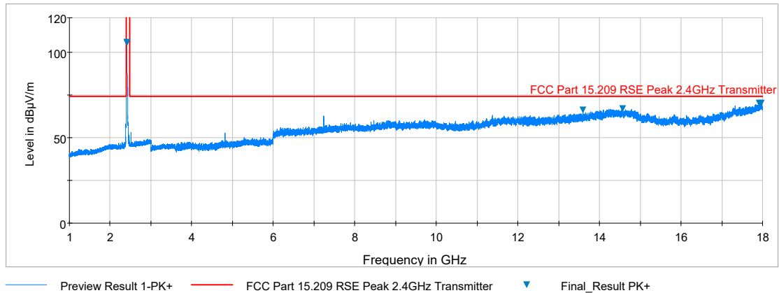
Plot 7-32. Radiated Spurious Plot above 1GHz (802.11b – Ch. 1, Ant. Pol. V)
