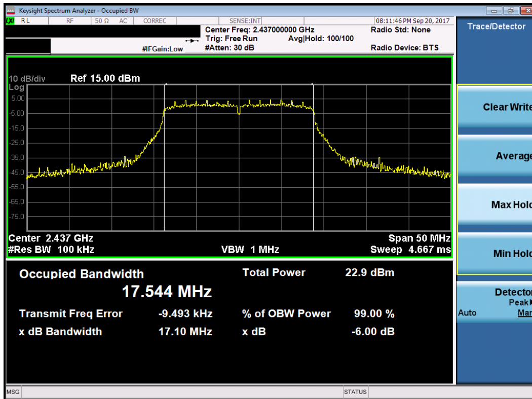
Plot 7-8. 6dB Bandwidth Plot (802.11n (2.4GHz) – Ch. 6)
