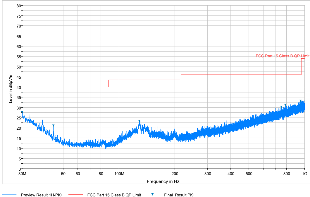
Plot 7-42. Radiated Spurious Plot below 1GHz (Pol. V)
