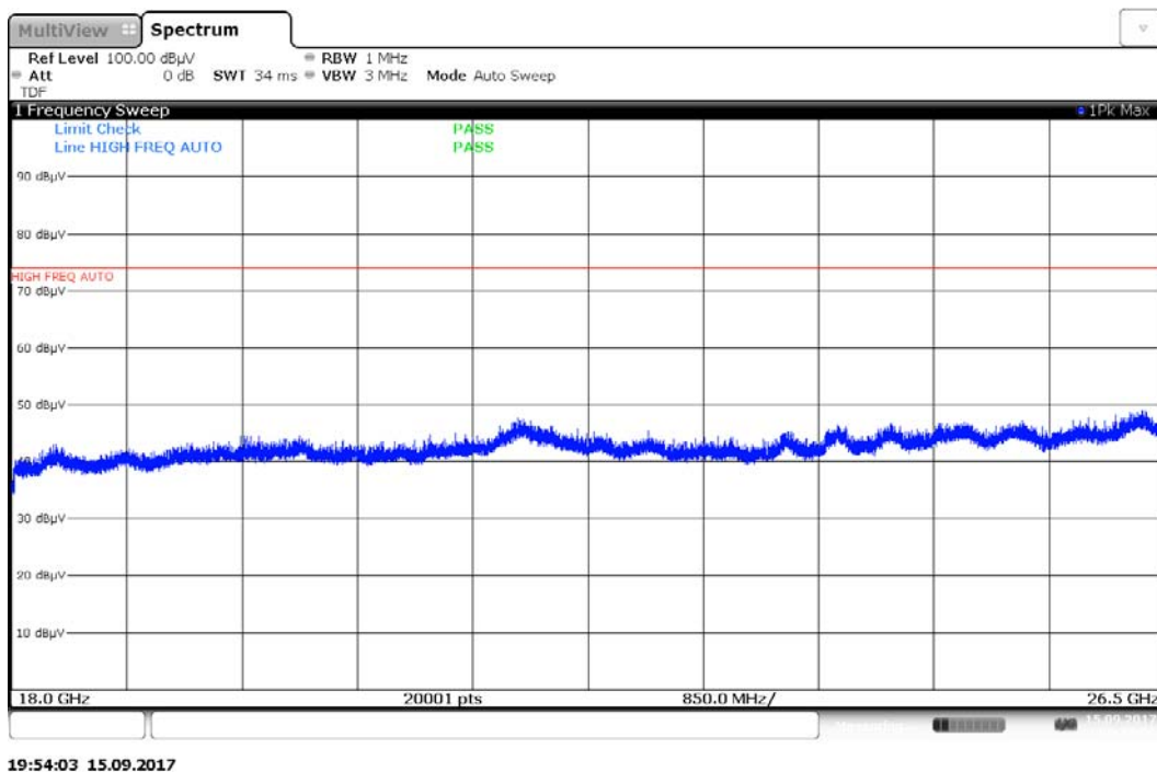
Plot 7-38. Radiated Spurious Plot above 18GHz (Pol. V)
