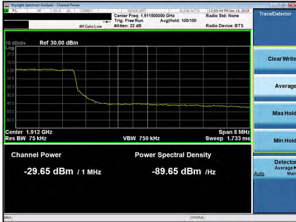
Plot 7-140. Upper Extended Band Edge Plot (Band 2 - 10.0MHz QPSK - Full RB Configuration)
