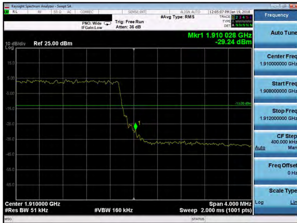
Plot 7-133. Upper Band Edge Plot (Band 2- 5.0MHz QPSK - Full RB Configuration)
