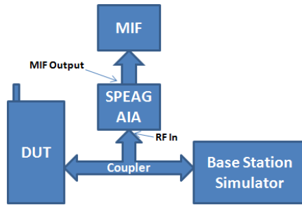
Figure 7-1 MIF Measurement Setup for licensed modes
