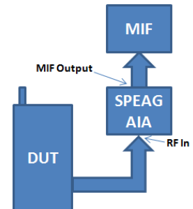
Figure 7-2 MIF Measurement Setup for unlicensed modes
