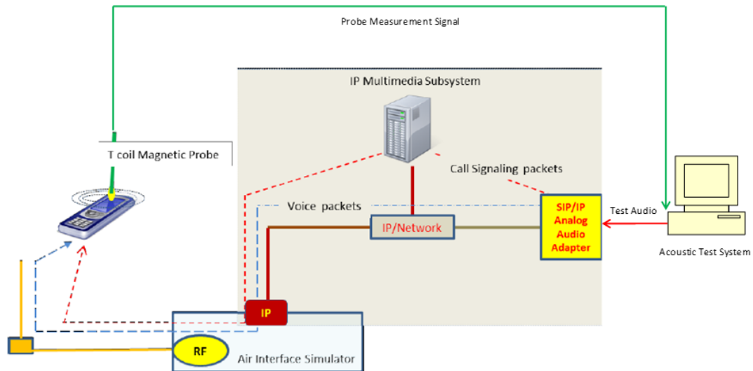
Figure 5-1 Test Setup for VoLTE T-Coil Measurements
