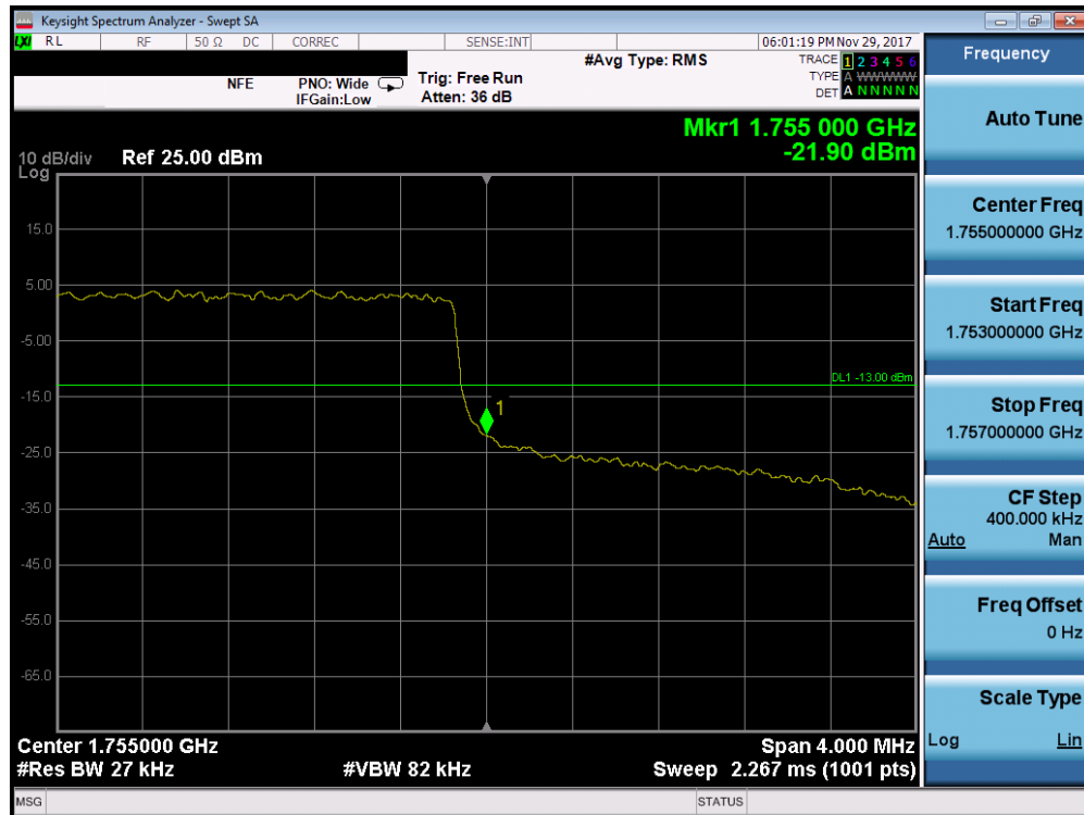
Plot 7-95. Upper Band Edge Plot (Band 4 - 3.0MHz QPSK - Full RB Configuration)
