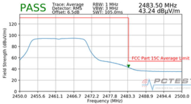
Plot 7-41. Radiated Restricted Upper Band Edge Measurement (Average)
