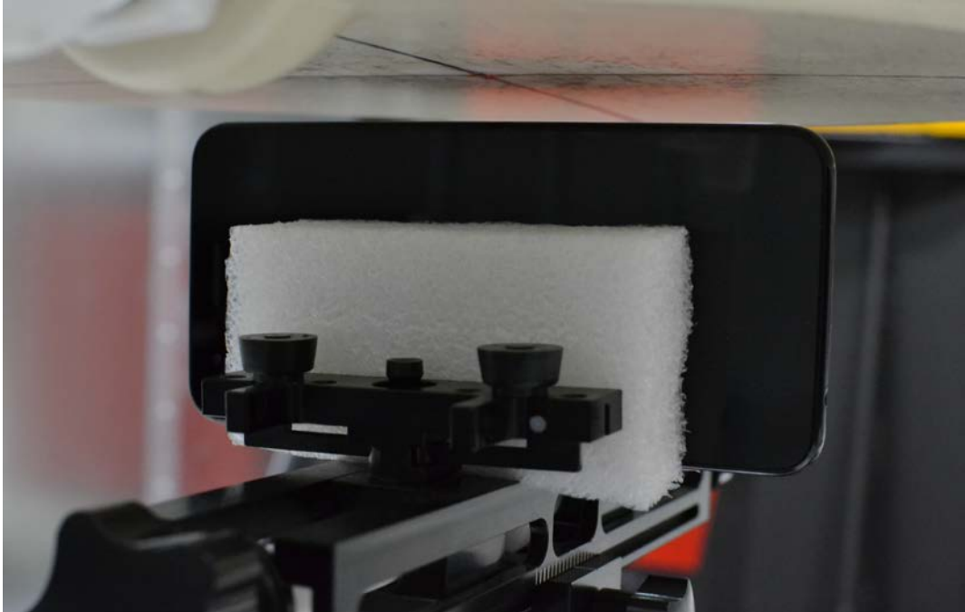
SAR Test Setup Photo 9: Right Edge at 1.0 cm
