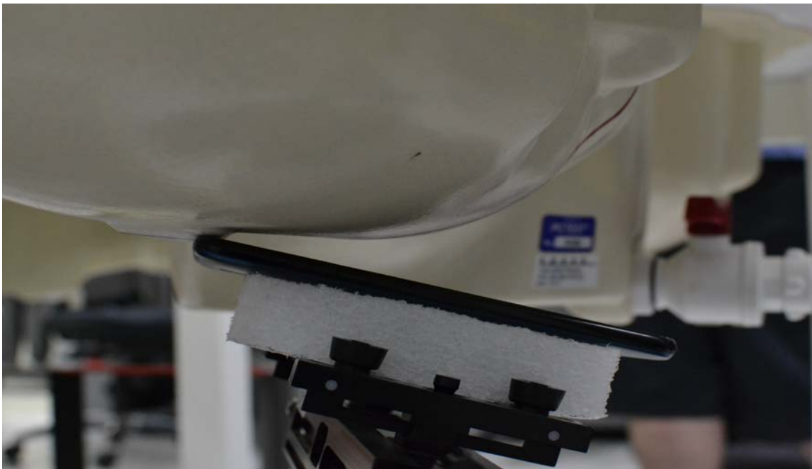
SAR Test Setup Photo 2: Right Tilt
