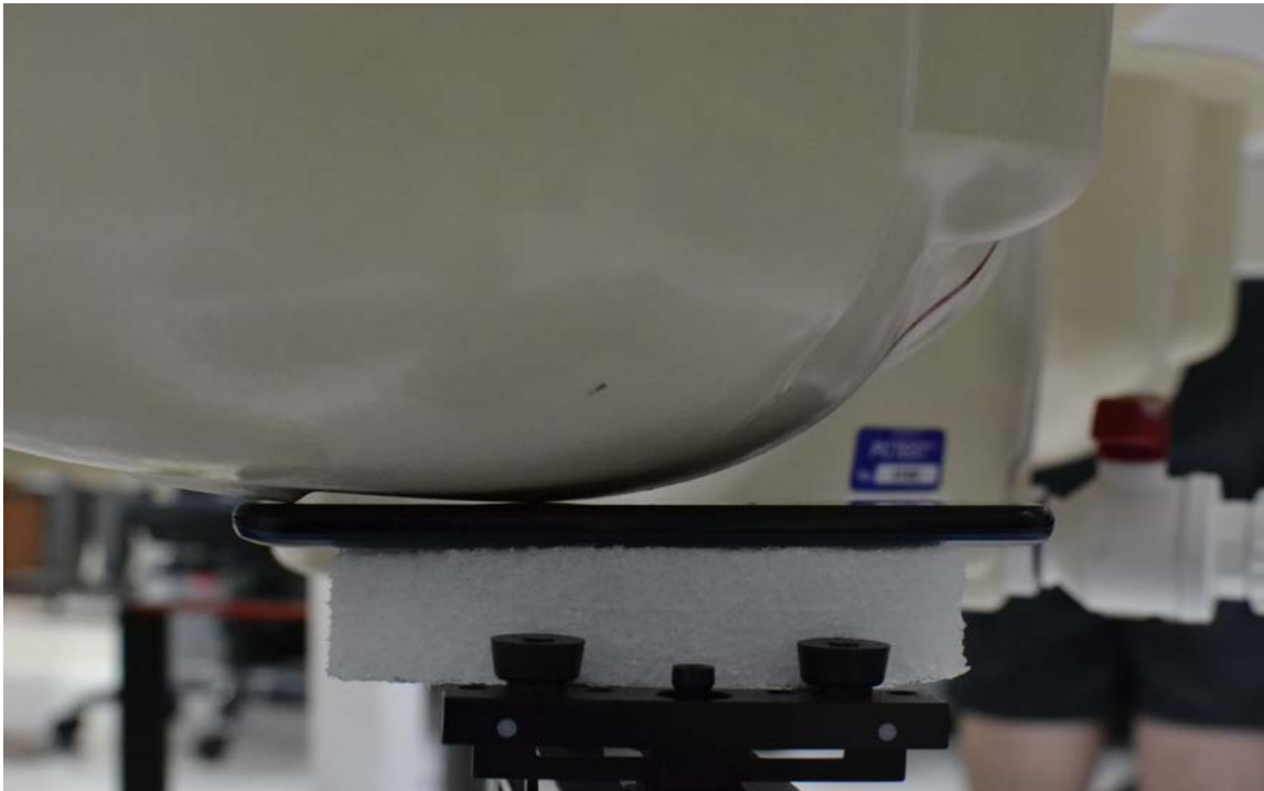
SAR Test Setup Photo 1: Right Cheek
