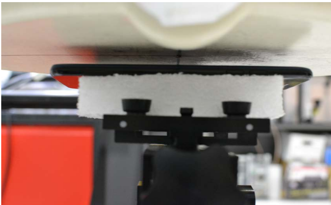
SAR Test Setup Photo 5: Back side at 1.0 cm
