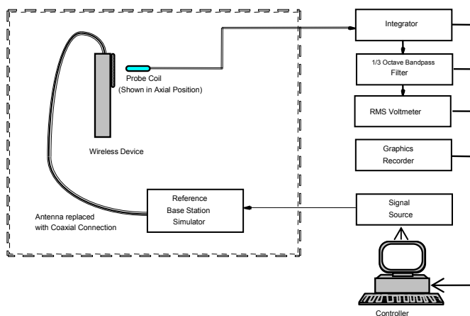
Figure 4-14 Audio Magnetic Field Test Setup
