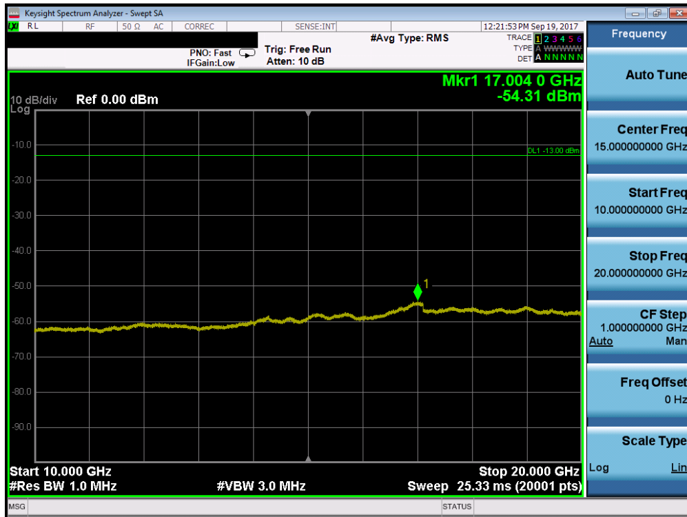
Plot 7-78. Conducted Spurious Plot (Band 66/4 - 5.0MHz QPSK - RB Size 1, RB Offset 0 - Low Channel)
