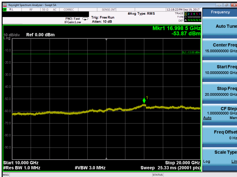
Plot 7-81. Conducted Spurious Plot (Band 66/4 - 5.0MHz QPSK - RB Size 1, RB Offset 0 - Mid Channel)
