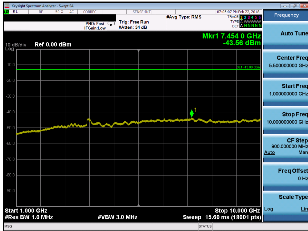
Plot 7-51. Conducted Spurious Plot (Band 71 - 5.0MHz QPSK - RB Size 1, RB Offset 0 - Low Channel)
