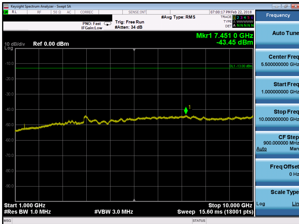
Plot 7-54. Conducted Spurious Plot (Band 71 - 5.0MHz QPSK - RB Size 1, RB Offset 0 - Mid Channel)
