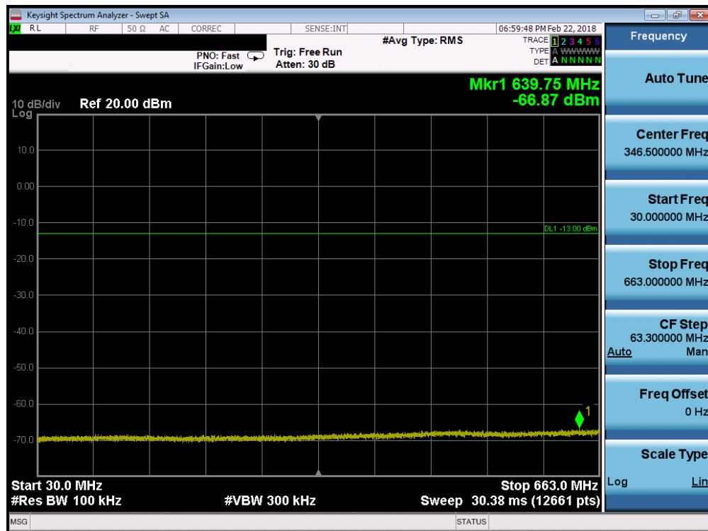
Plot 7-52. Conducted Spurious Plot (Band 71 - 5.0MHz QPSK - RB Size 1, RB Offset 0 - Mid Channel)
