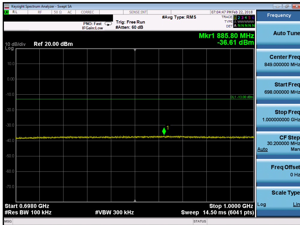
Plot 7-50. Conducted Spurious Plot (Band 71 - 5.0MHz QPSK - RB Size 1, RB Offset 0 - Low Channel)
