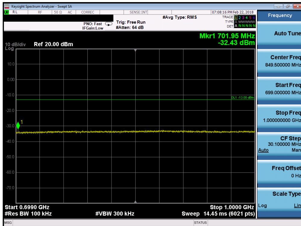
Plot 7-56. Conducted Spurious Plot (Band 71 - 5.0MHz QPSK - RB Size 1, RB Offset 0 - High Channel)
