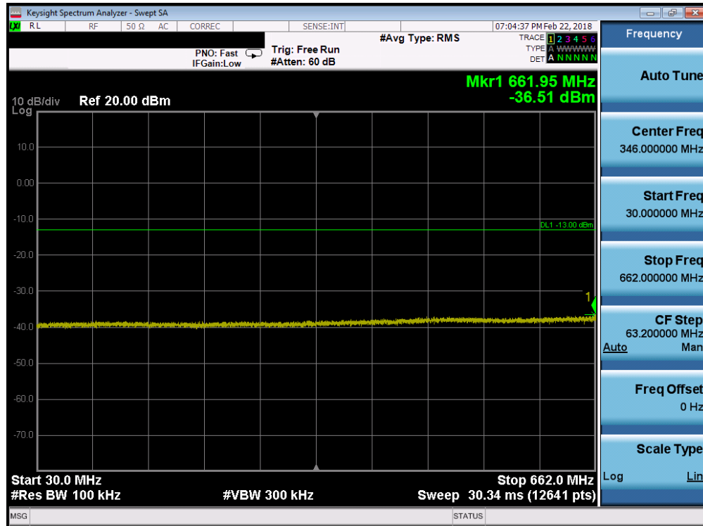
Plot 7-49. Conducted Spurious Plot (Band 71 - 5.0MHz QPSK - RB Size 1, RB Offset 0 - Low Channel)
