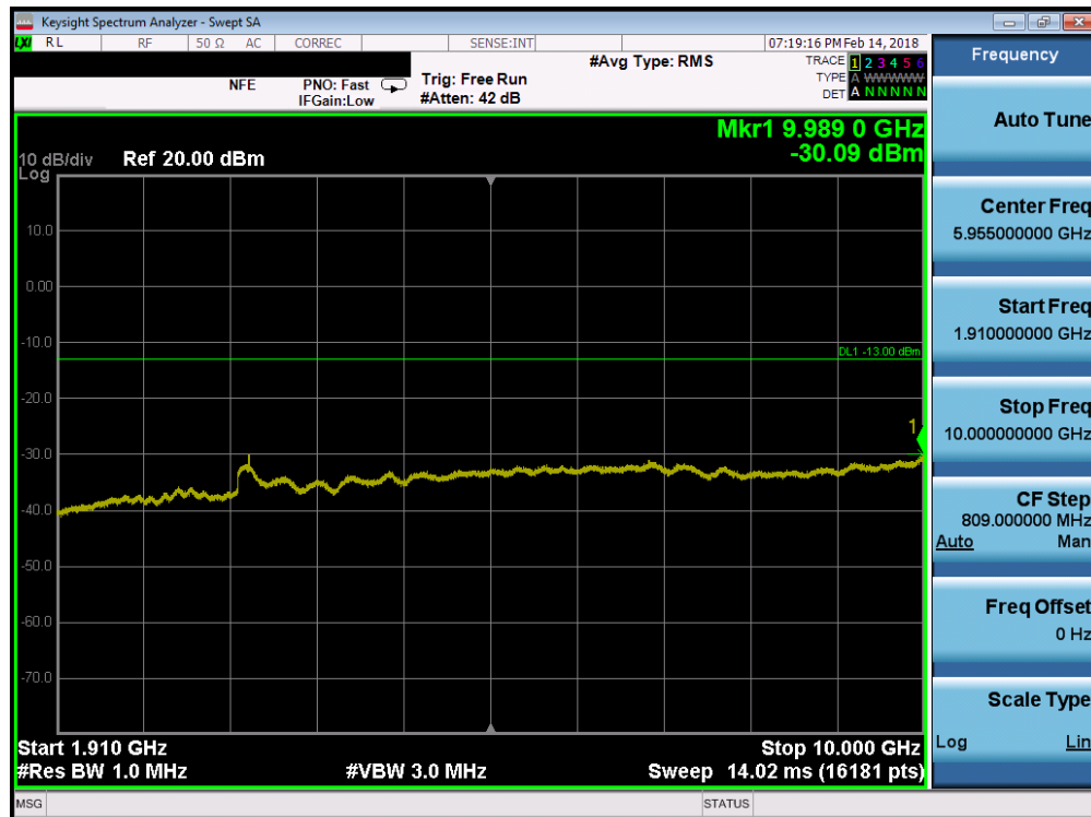
Plot 7-86. Conducted Spurious Plot (Band 2 - 10.0MHz QPSK - RB Size 1, RB Offset 0 - Low Channel)
