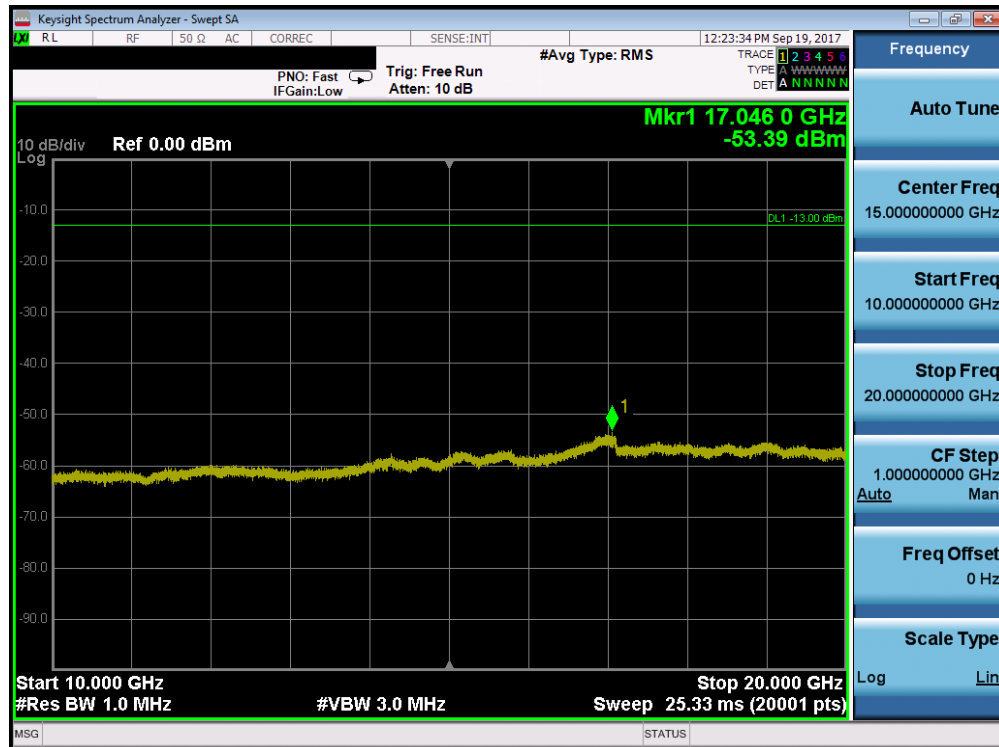
Plot 7-84. Conducted Spurious Plot (Band 66/4 - 5.0MHz QPSK - RB Size 1, RB Offset 0 - High Channel)
