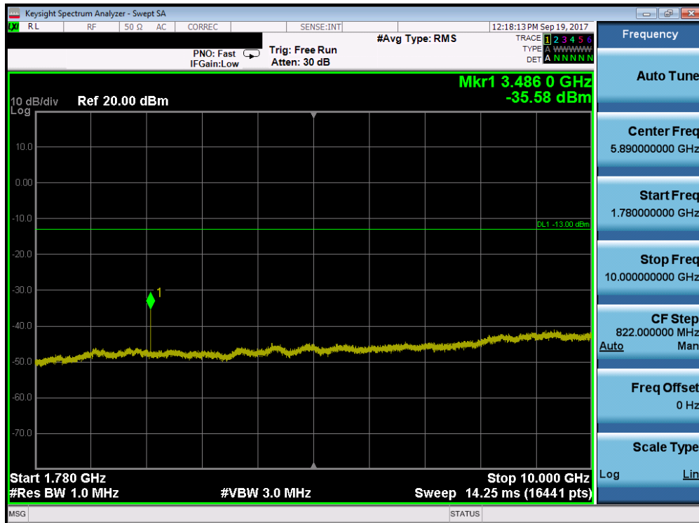
Plot 7-80. Conducted Spurious Plot (Band 66/4 - 5.0MHz QPSK - RB Size 1, RB Offset 0 - Mid Channel)
