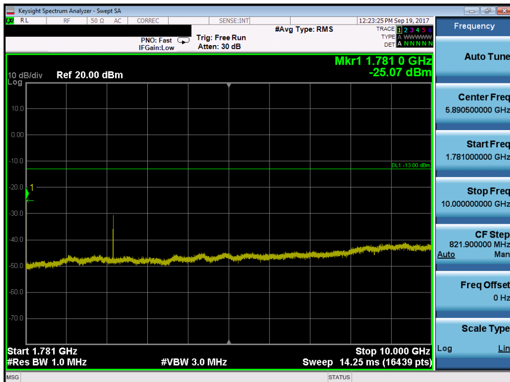
Plot 7-83. Conducted Spurious Plot (Band 66/4 - 5.0MHz QPSK - RB Size 1, RB Offset 0 - High Channel)
