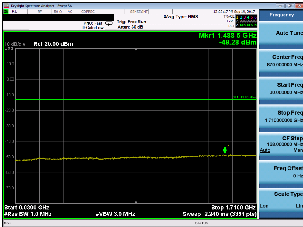
Plot 7-82. Conducted Spurious Plot (Band 66/4 - 5.0MHz QPSK - RB Size 1, RB Offset 0 - High Channel)
