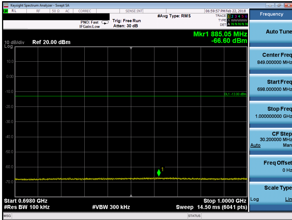
Plot 7-53. Conducted Spurious Plot (Band 71 - 5.0MHz QPSK - RB Size 1, RB Offset 0 - Mid Channel)
