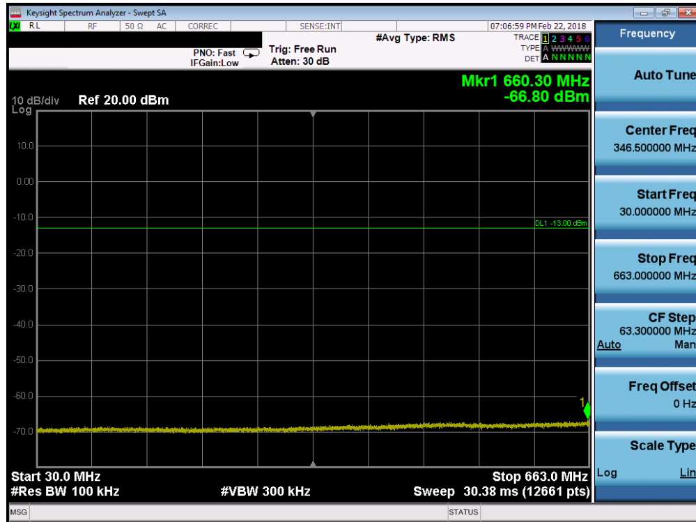
Plot 7-55. Conducted Spurious Plot (Band 71 - 5.0MHz QPSK - RB Size 1, RB Offset 0 - High Channel)
