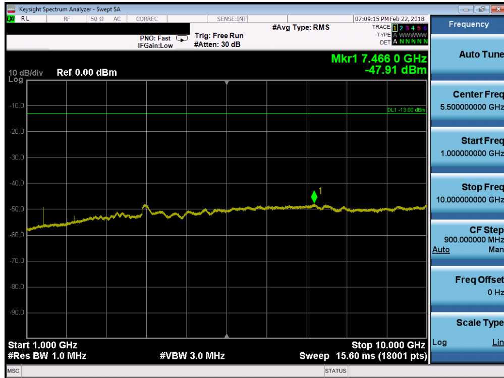
Plot 7-57. Conducted Spurious Plot (Band 71 - 5.0MHz QPSK - RB Size 1, RB Offset 0 - High Channel)
