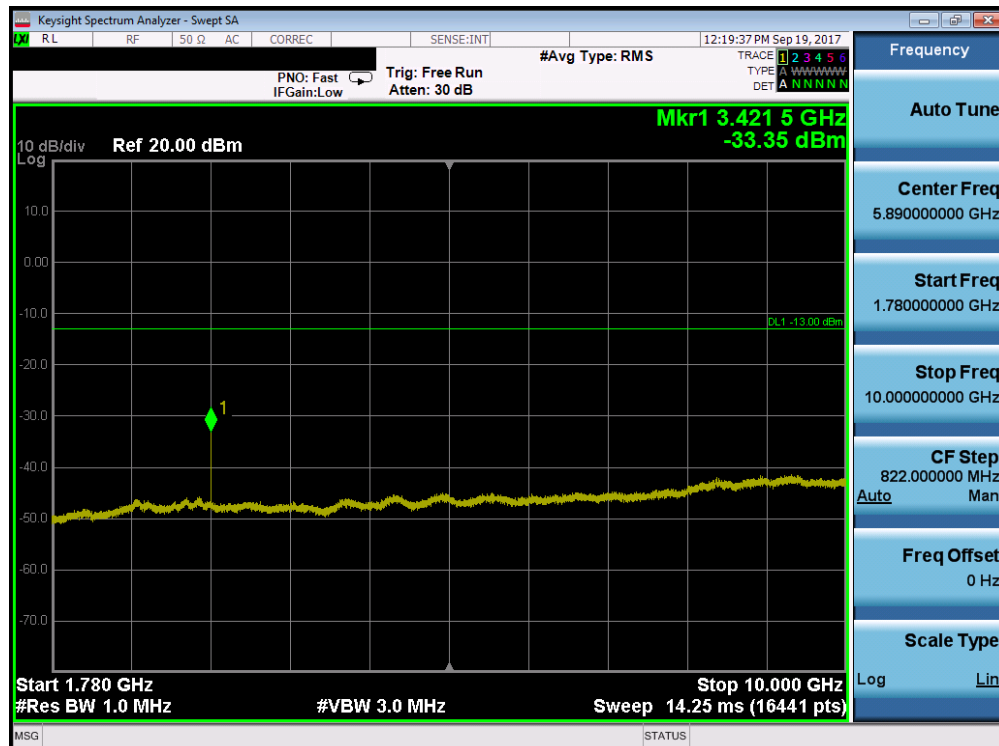
Plot 7-77. Conducted Spurious Plot (Band 66/4 - 5.0MHz QPSK - RB Size 1, RB Offset 0 - Low Channel)
