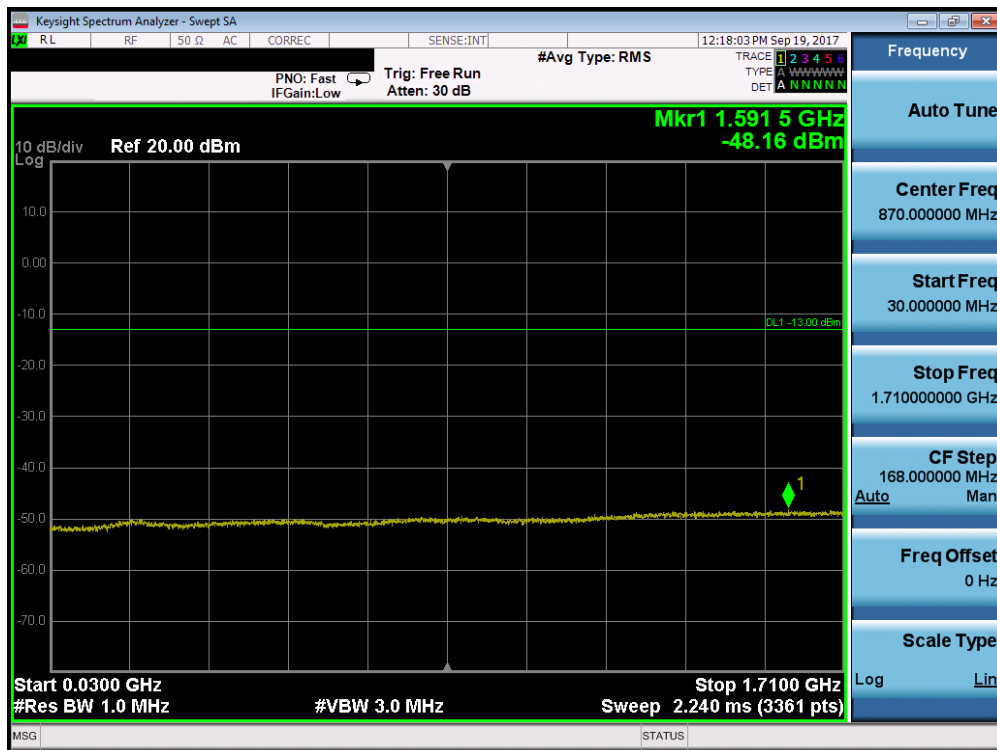
Plot 7-79. Conducted Spurious Plot (Band 66/4 - 5.0MHz QPSK - RB Size 1, RB Offset 0 - Mid Channel)
