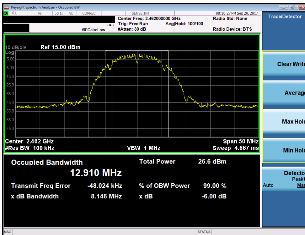
Plot 7-3. 6dB Bandwidth Plot (802.11b – Ch. 11)
